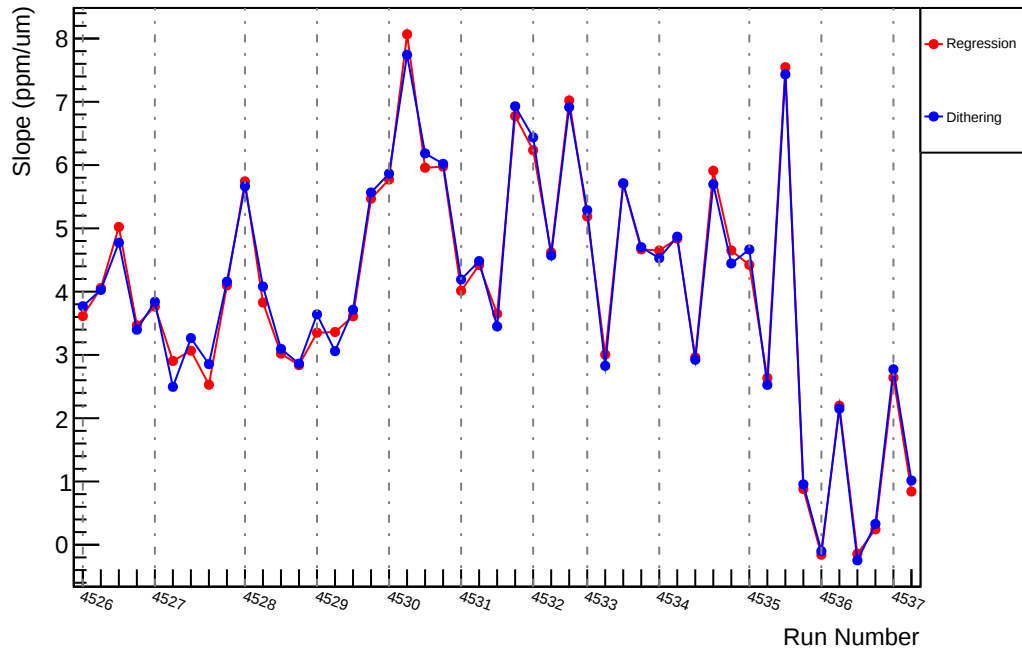
Slug65: Slope : us_dd_vs_evMon2 (ppm/um)
