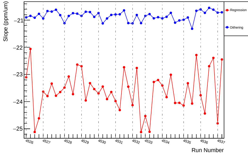
Slug65: Slope : us_dd_vs_evMon3 (ppm/um)
