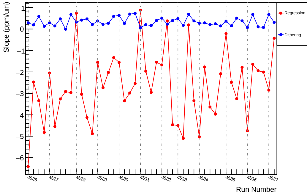
Slug65: Slope : us_dd_vs_evMon4 (ppm/um)
