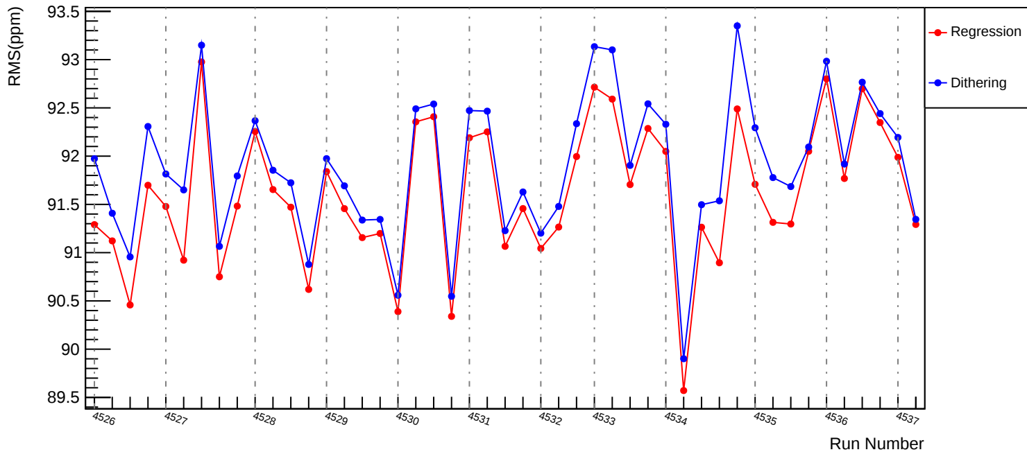
Slug65: Corrected RMS (ppm): asym_us_dd
