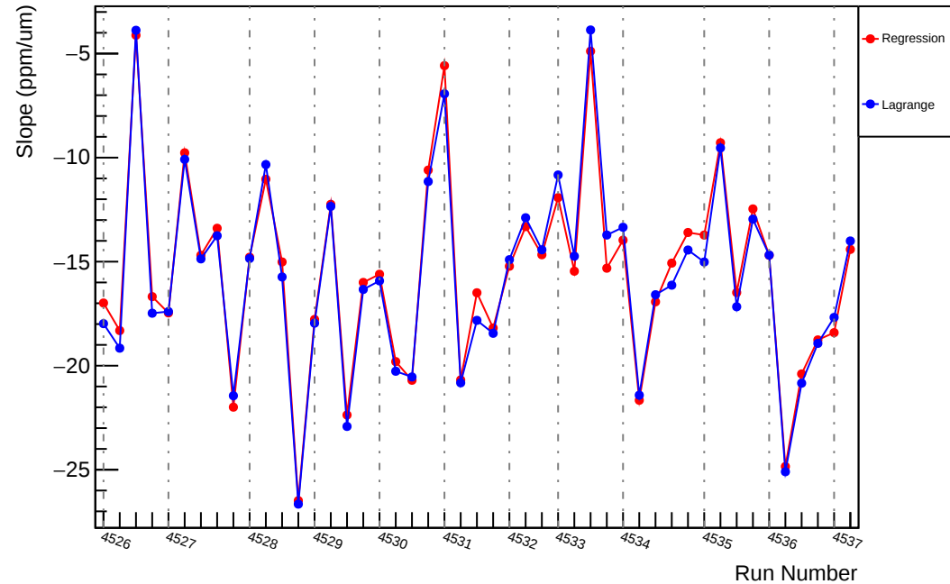
Slug65: Slope : usl_vs_evMon11 (ppm/um)
