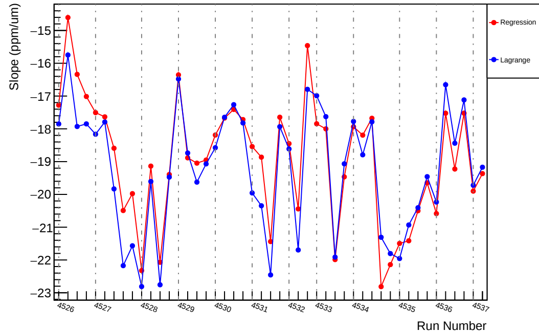
Slug65: Slope : usl_vs_evMon6 (ppm/um)
