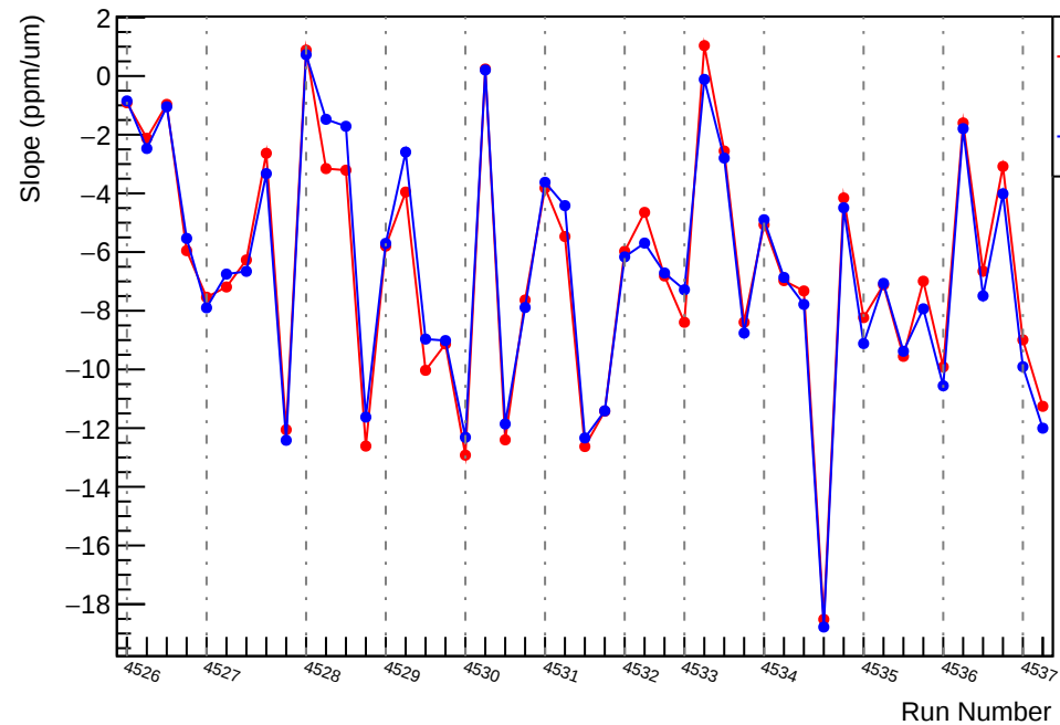
Slug65: Slope : usl_vs_evMon10 (ppm/um)
