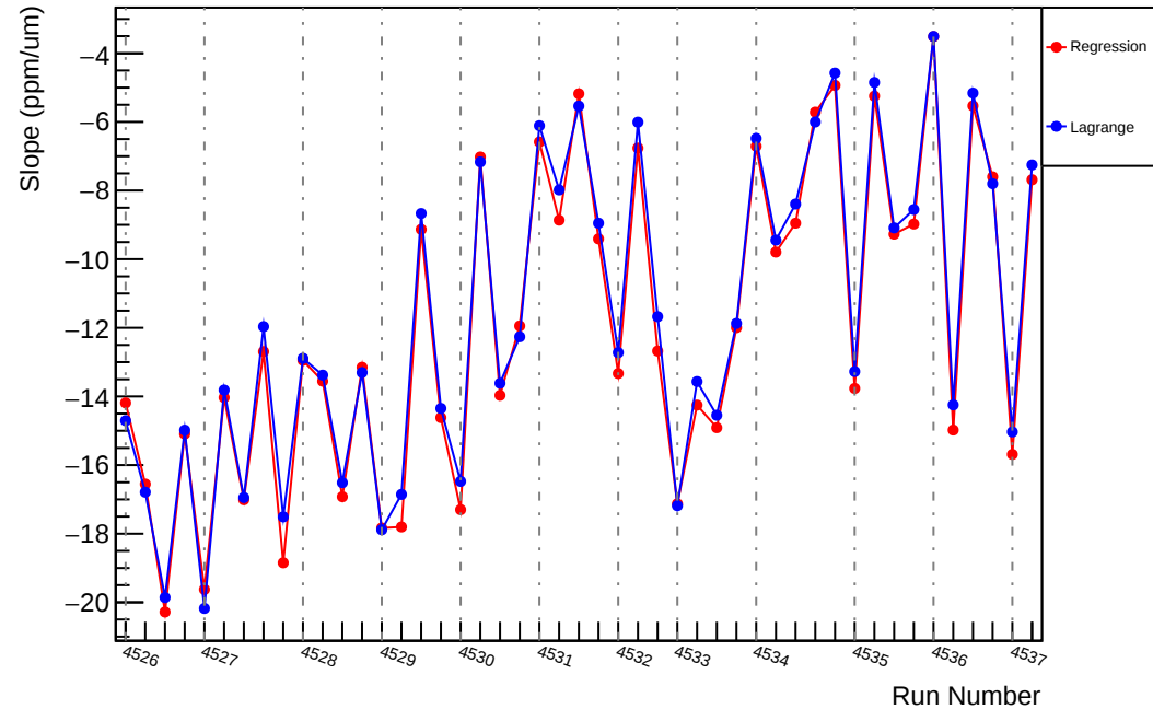
Slug65: Slope : usl_vs_evMon4 (ppm/um)
