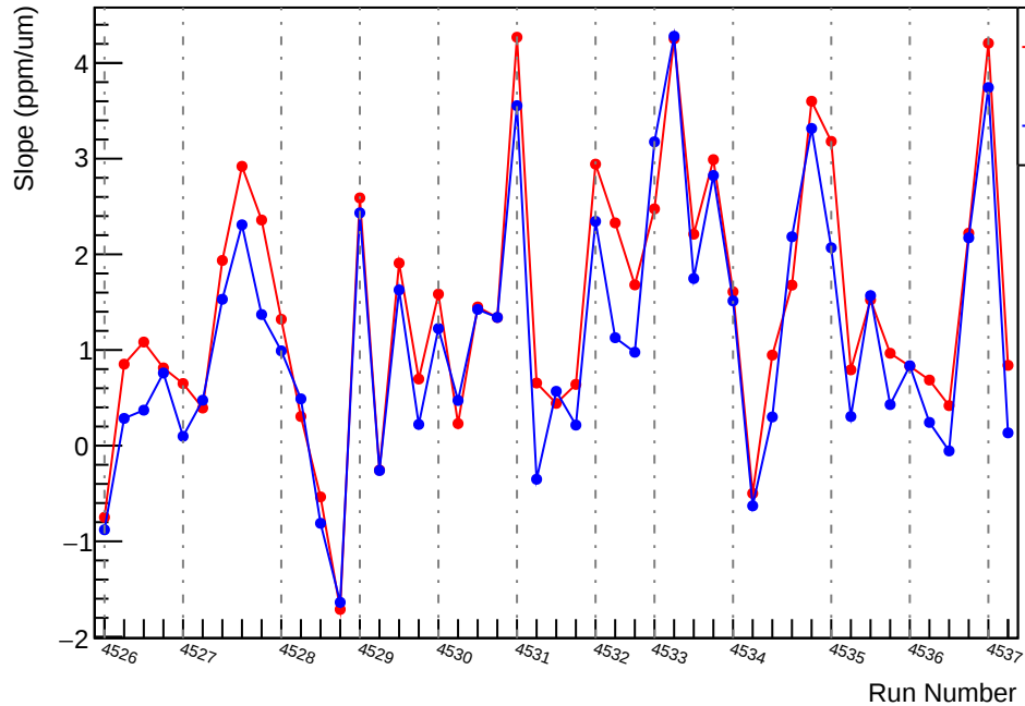
Slug65: Slope : usl_vs_evMon5 (ppm/um)
