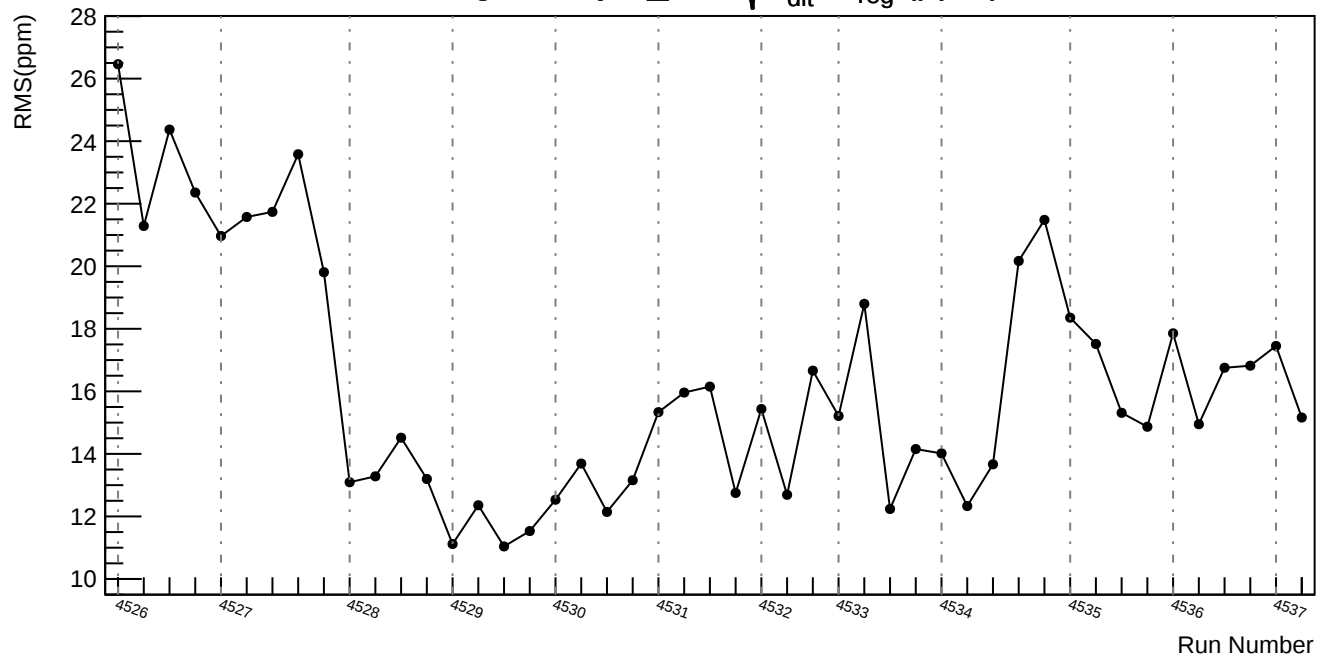
Slug65: asym_usr: \sqrt{\sigma_{\text{dit}}^2 - \sigma_{\text{reg}}^2} (ppm)
