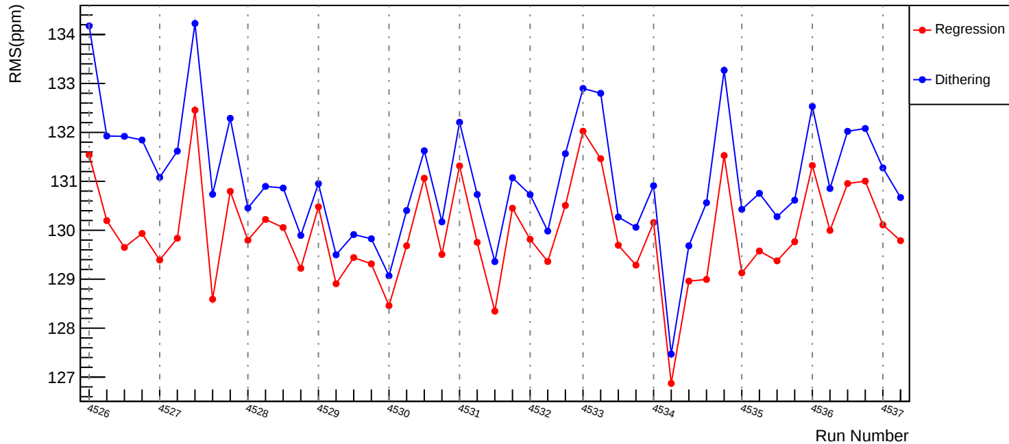
Slug65: Corrected RMS (ppm): asym_usr
