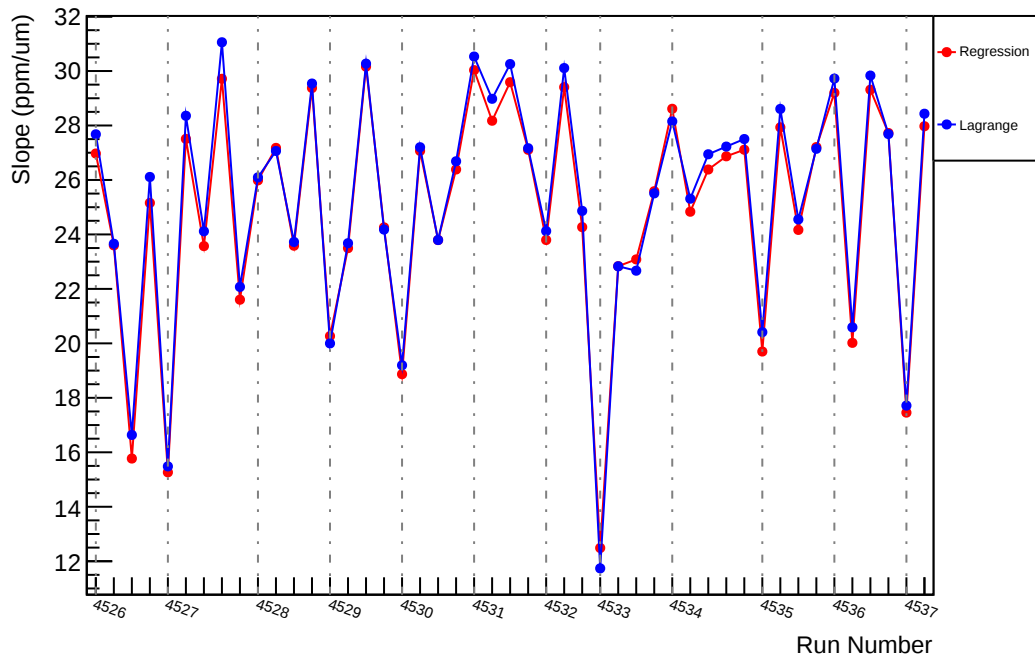
Slug65: Slope : usr_vs_evMon3 (ppm/um)
