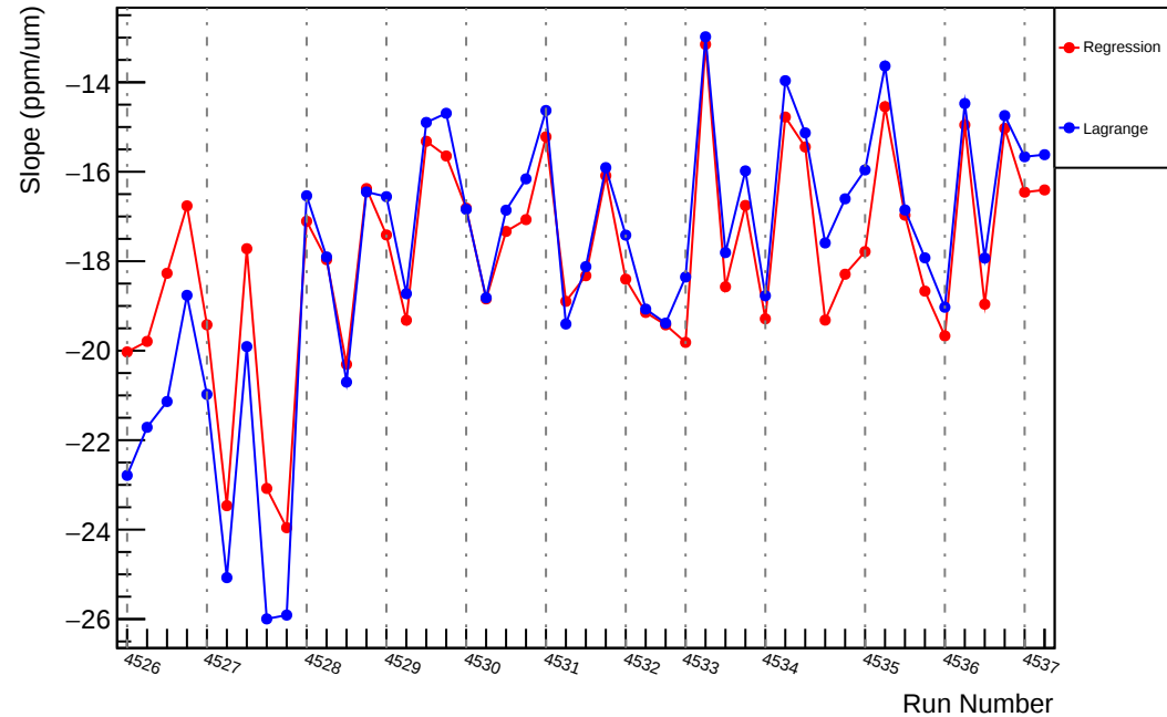
Slug65: Slope : usr_vs_evMon6 (ppm/um)
