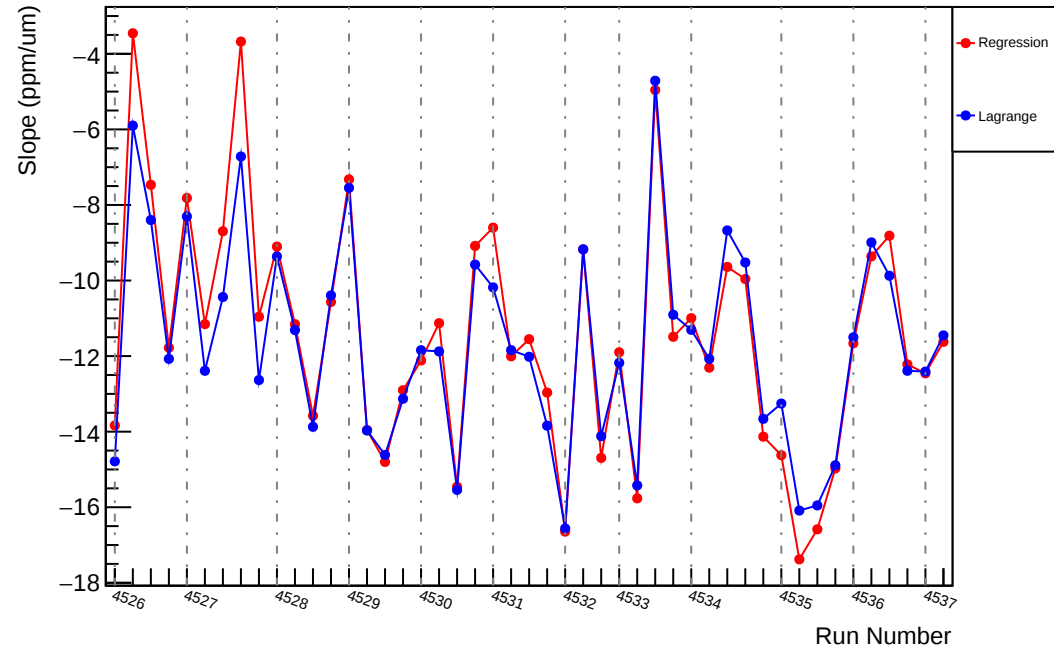
Slug65: Slope : usr_vs_evMon8 (ppm/um)
