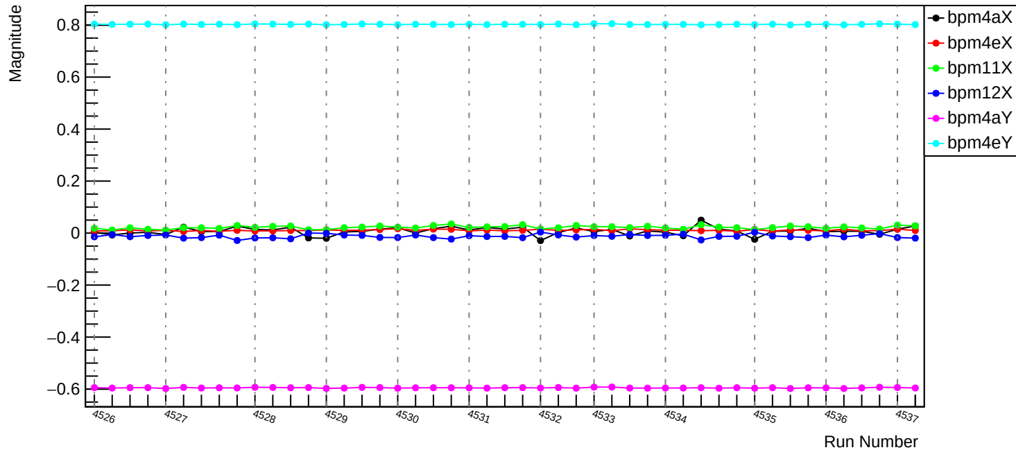
Slug65: EigenVector #4
