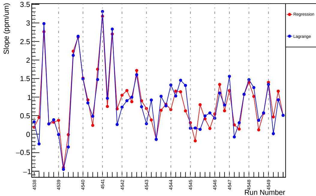
Slug66: Slope : us_avg_vs_evMon5 (ppm/um)
