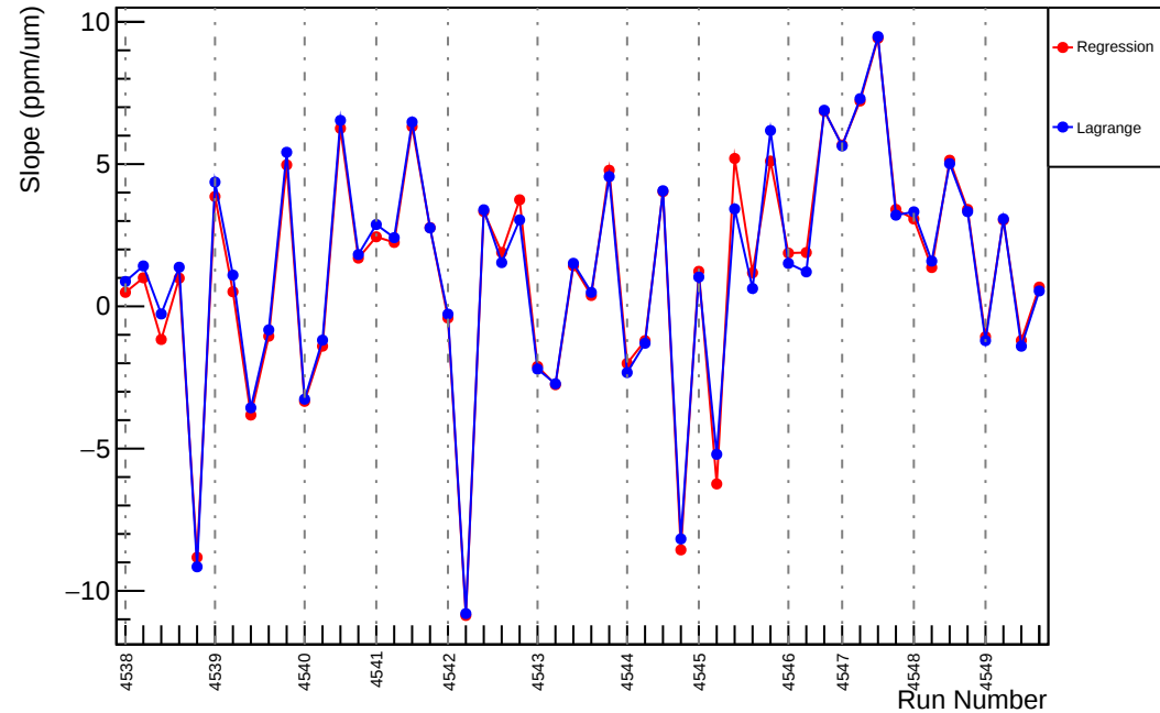
Slug66: Slope : us_avg_vs_evMon10 (ppm/um)
