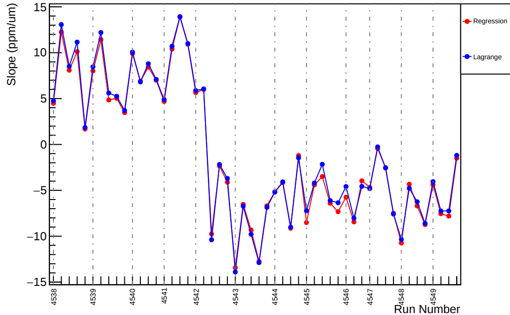
Slug66: Slope : us_avg_vs_evMon9 (ppm/um)
