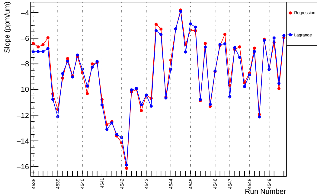
Slug66: Slope : us_avg_vs_evMon8 (ppm/um)
