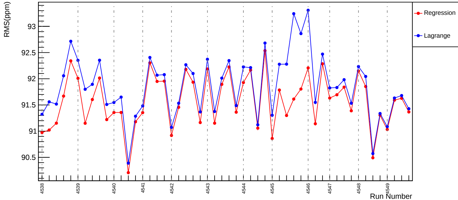
Slug66: Corrected RMS (ppm): asym_us_avg
