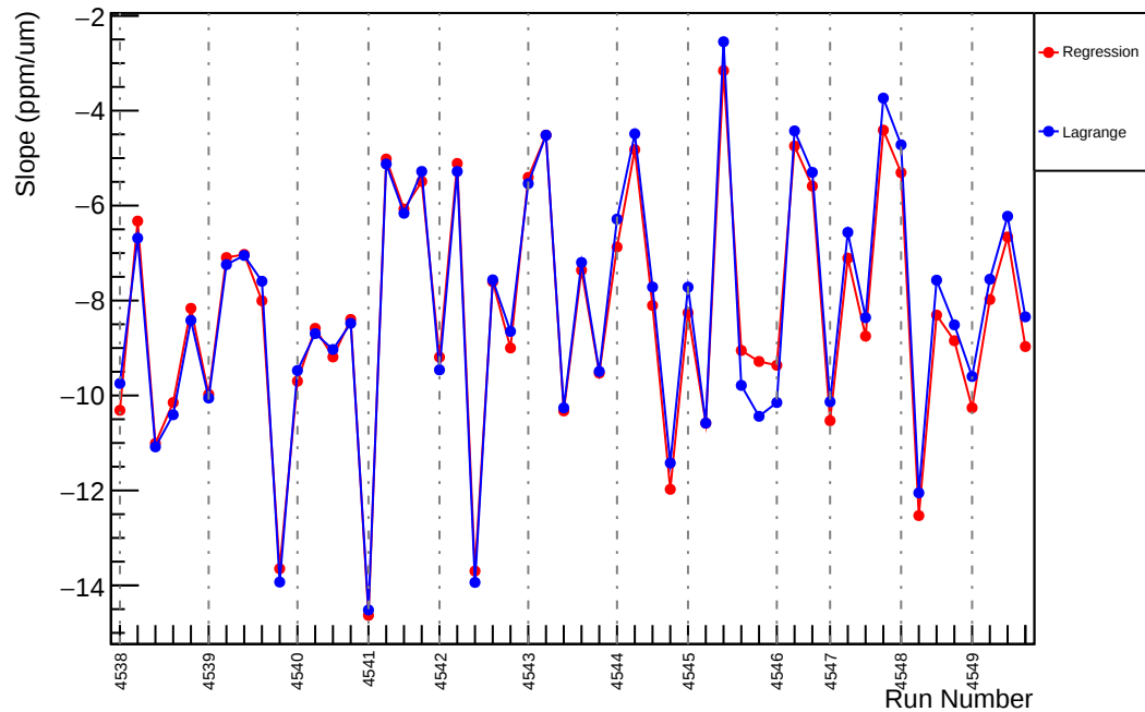
Slug66: Slope : us_avg_vs_evMon7 (ppm/um)
