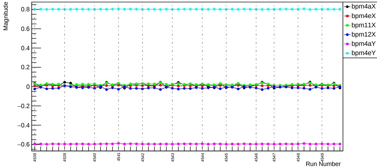
Slug66: EigenVector #4
