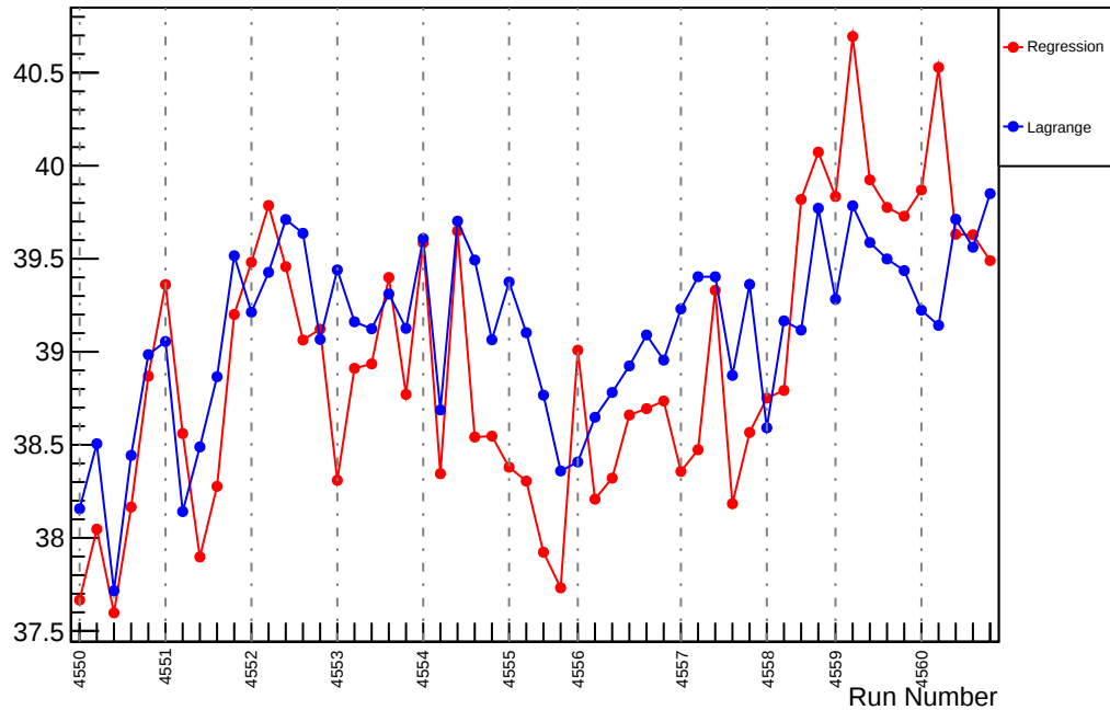
Slug67: Slope : us_avg_vs_evMon3 (ppm/um)
