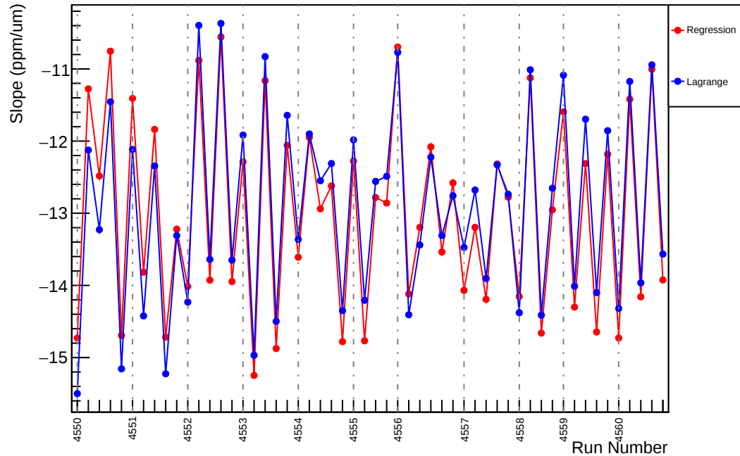
Slug67: Slope : us_avg_vs_evMon0 (ppm/um)
