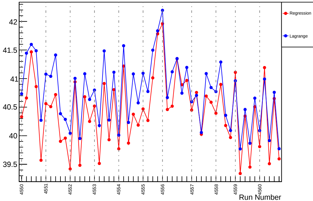
Slug67: Slope : us_avg_vs_evMon2 (ppm/um)
