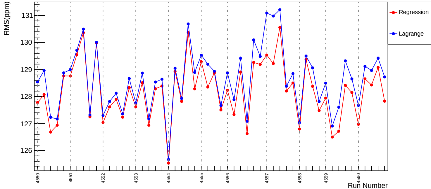
Slug67: Corrected RMS (ppm): asym_usl
