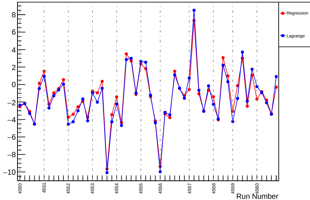
Slug67: Slope : usl_vs_evMon7 (ppm/um)
