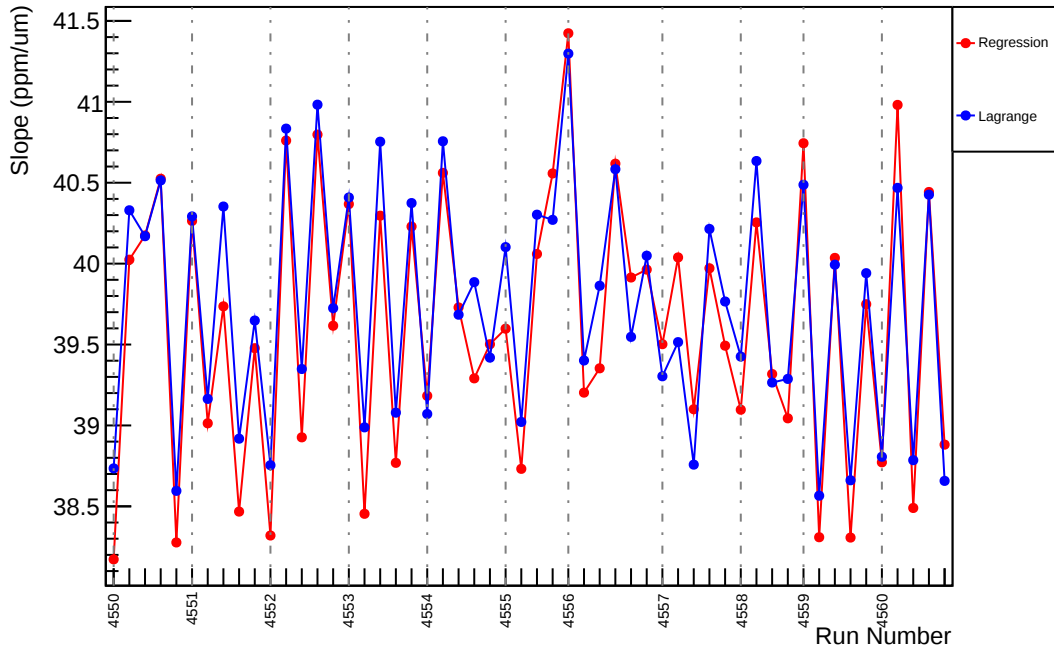
Slug67: Slope : usl_vs_evMon2 (ppm/um)
