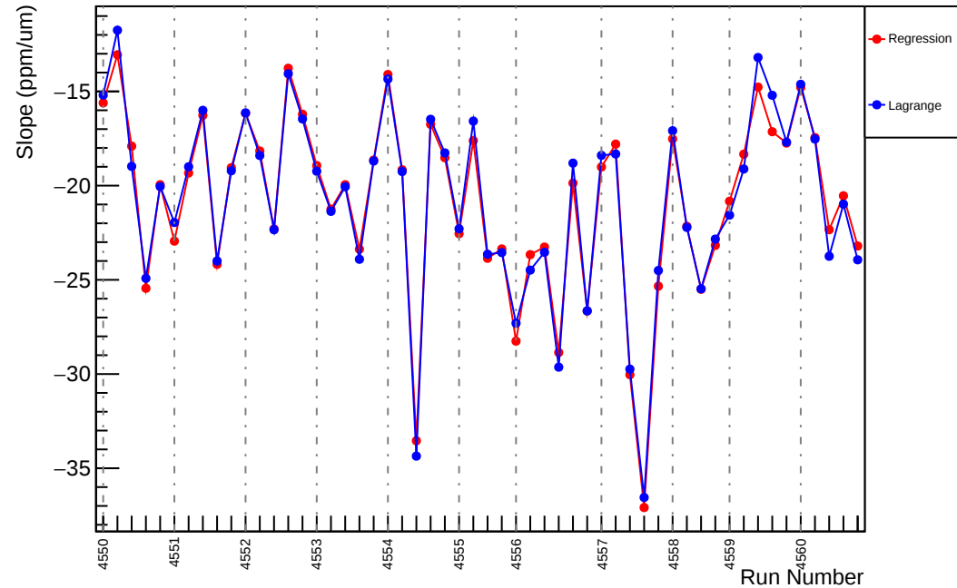
Slug67: Slope : usl_vs_evMon11 (ppm/um)
