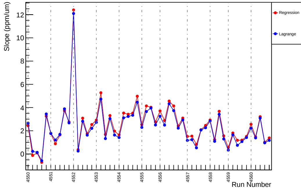
Slug67: Slope : usl_vs_evMon1 (ppm/um)
