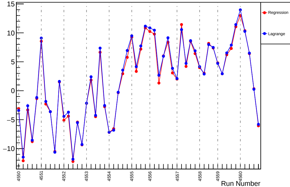
Slug67: Slope : usl_vs_evMon10 (ppm/um)
