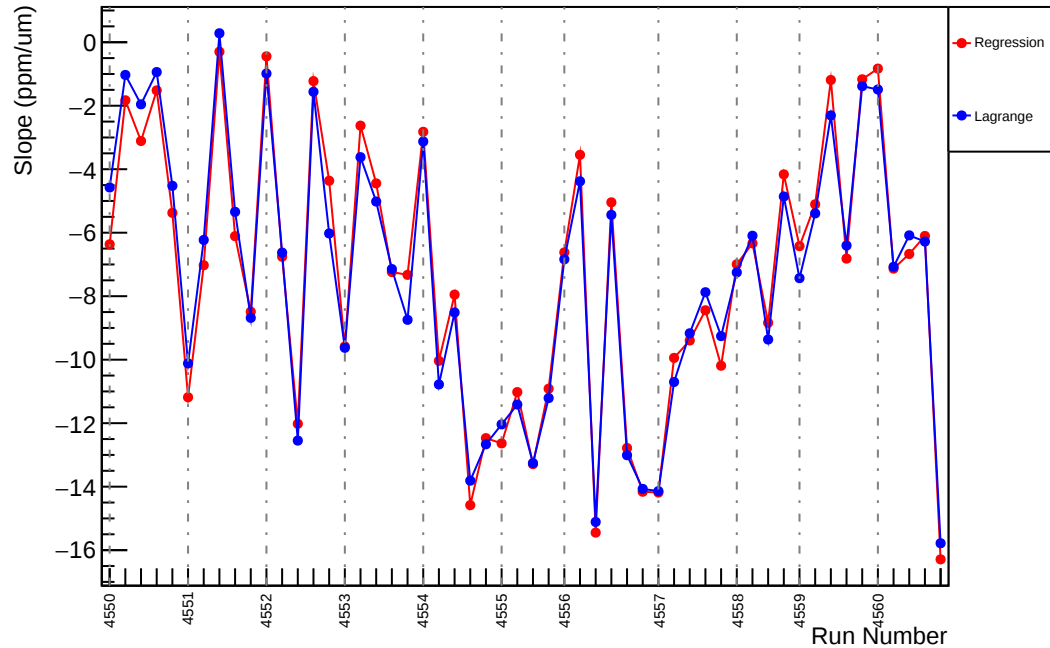
Slug67: Slope : usl_vs_evMon8 (ppm/um)
