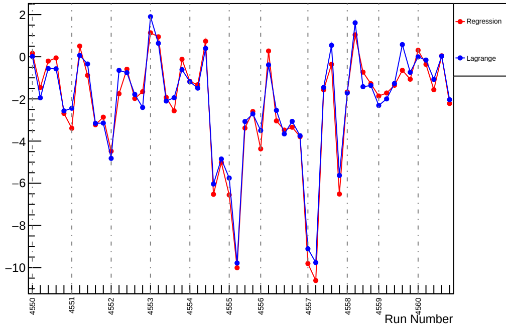
Slug67: Slope : usl_vs_evMon5 (ppm/um)
