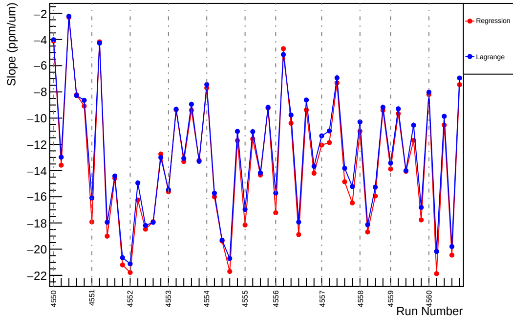
Slug67: Slope : usl_vs_evMon4 (ppm/um)
