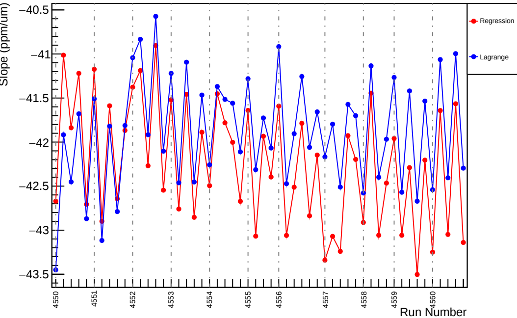
Slug67: Slope : usl_vs_evMon0 (ppm/um)
