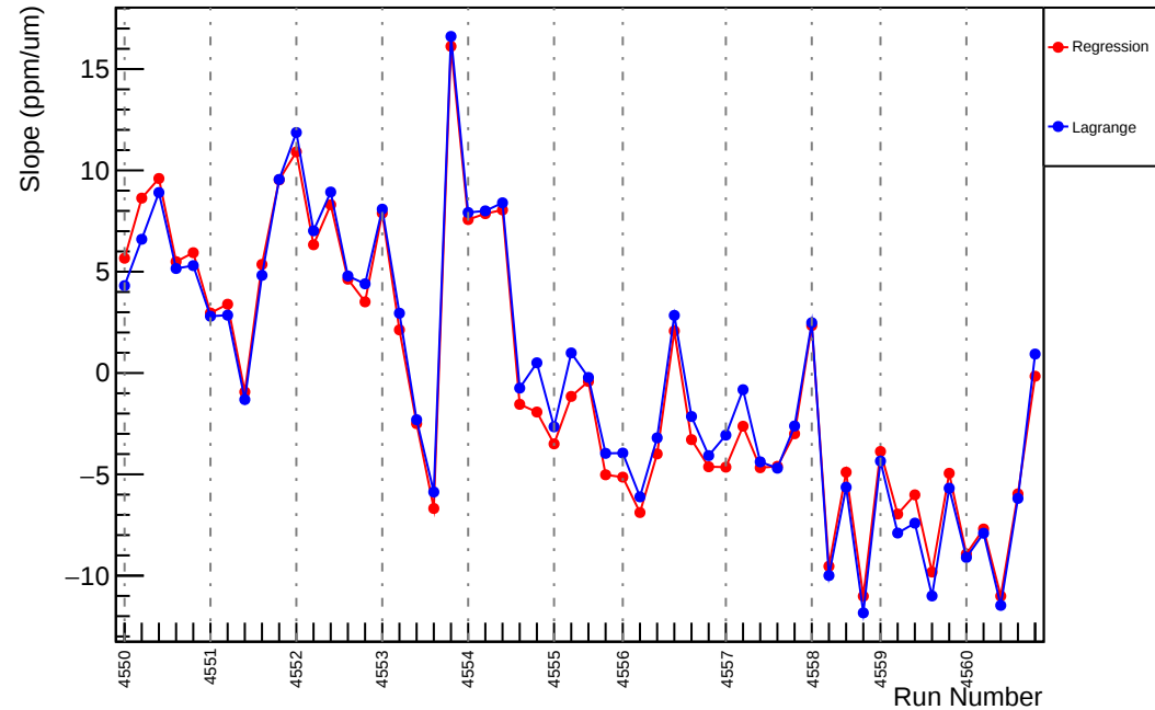
Slug67: Slope : usl_vs_evMon9 (ppm/um)
