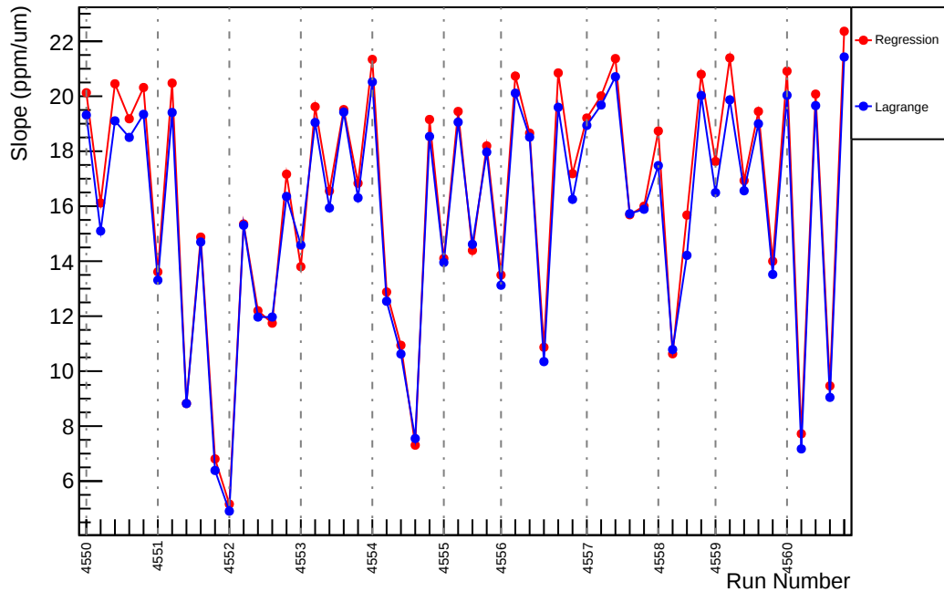
Slug67: Slope : usl_vs_evMon3 (ppm/um)
