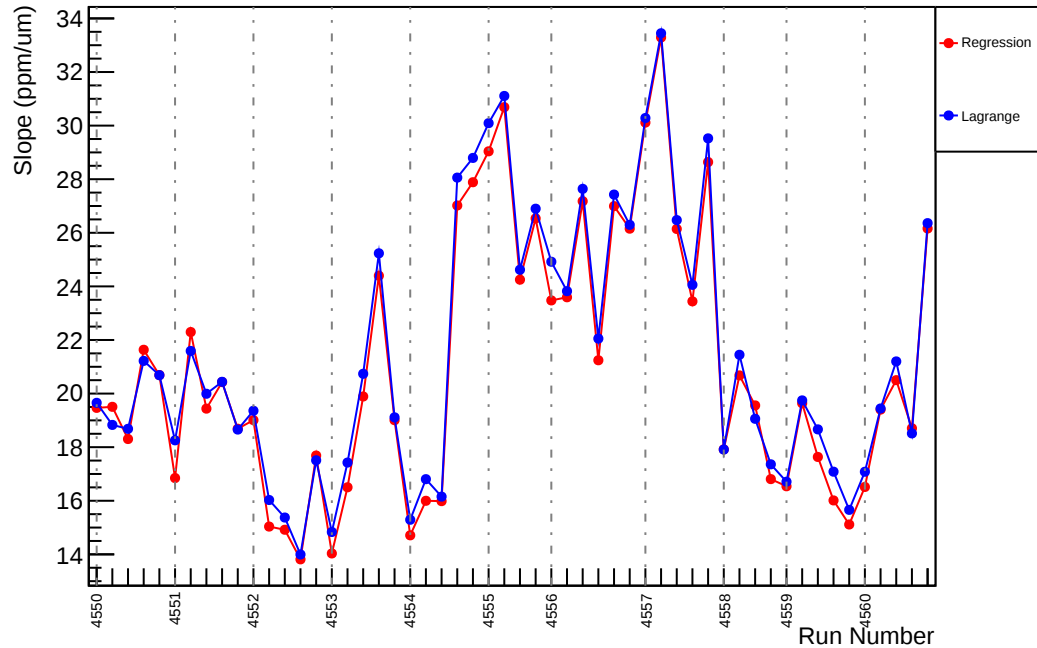
Slug67: Slope : usl_vs_evMon6 (ppm/um)
