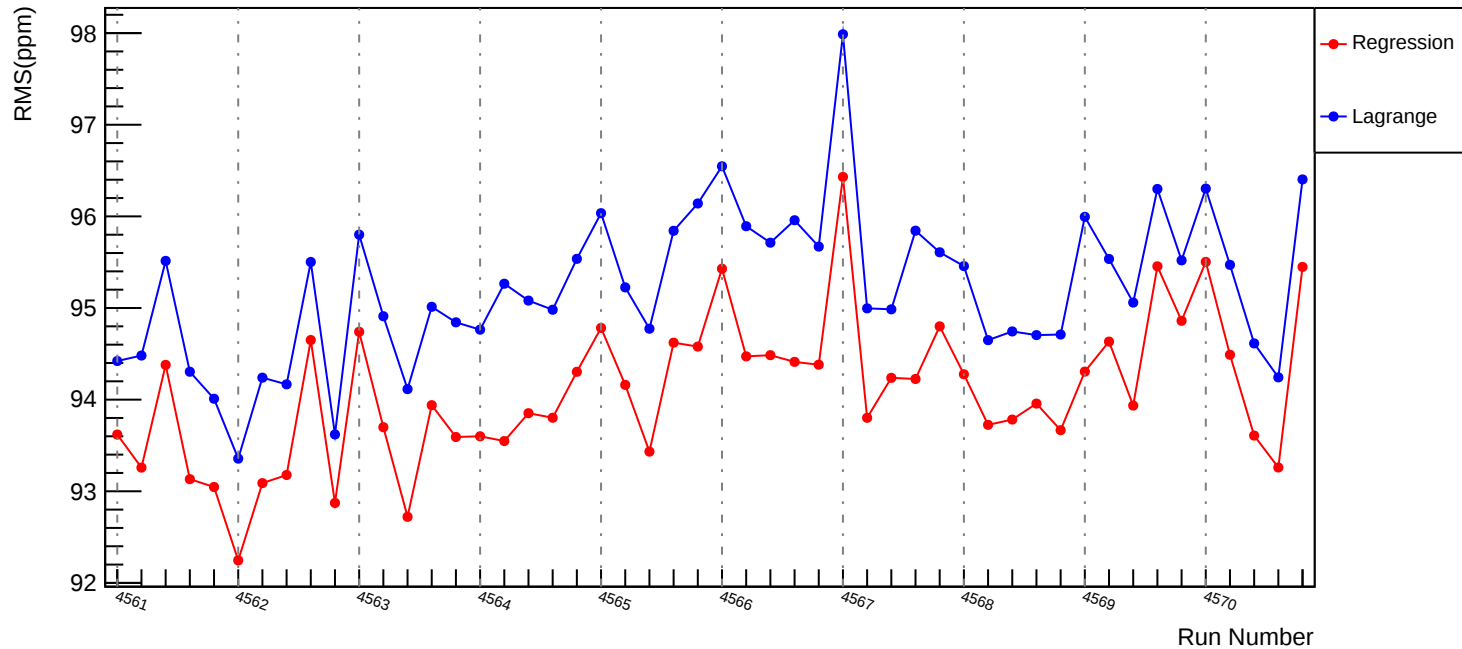
Slug68: Corrected RMS (ppm): asym_us_avg
