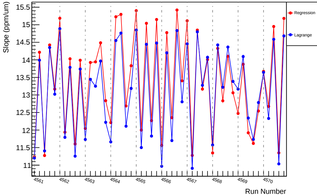
Slug68: Slope : us_avg_vs_evMon0 (ppm/um)
