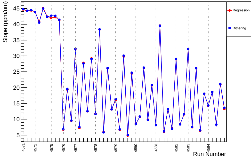
Slug69: Slope : us_dd_vs_evMon0 (ppm/um)
