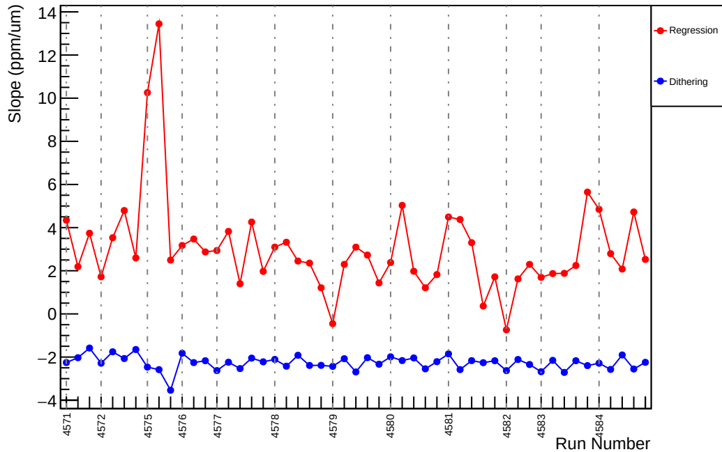
Slug69: Slope : us_dd_vs_evMon4 (ppm/um)
