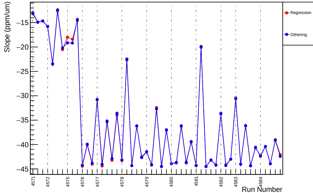
Slug69: Slope : us_dd_vs_evMon1 (ppm/um)
