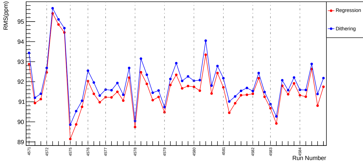
Slug69: Corrected RMS (ppm): asym_us_dd
