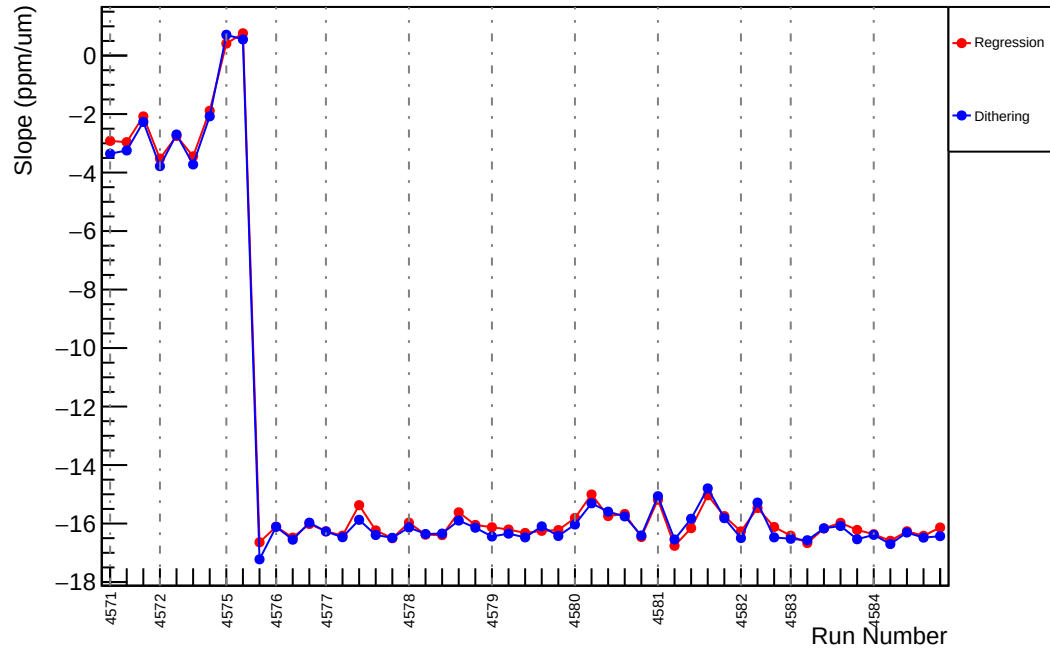
Slug69: Slope : us_dd_vs_evMon2 (ppm/um)
