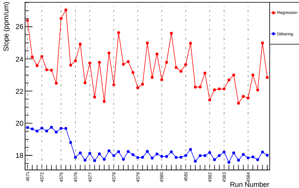
Slug69: Slope : us_dd_vs_evMon3 (ppm/um)
