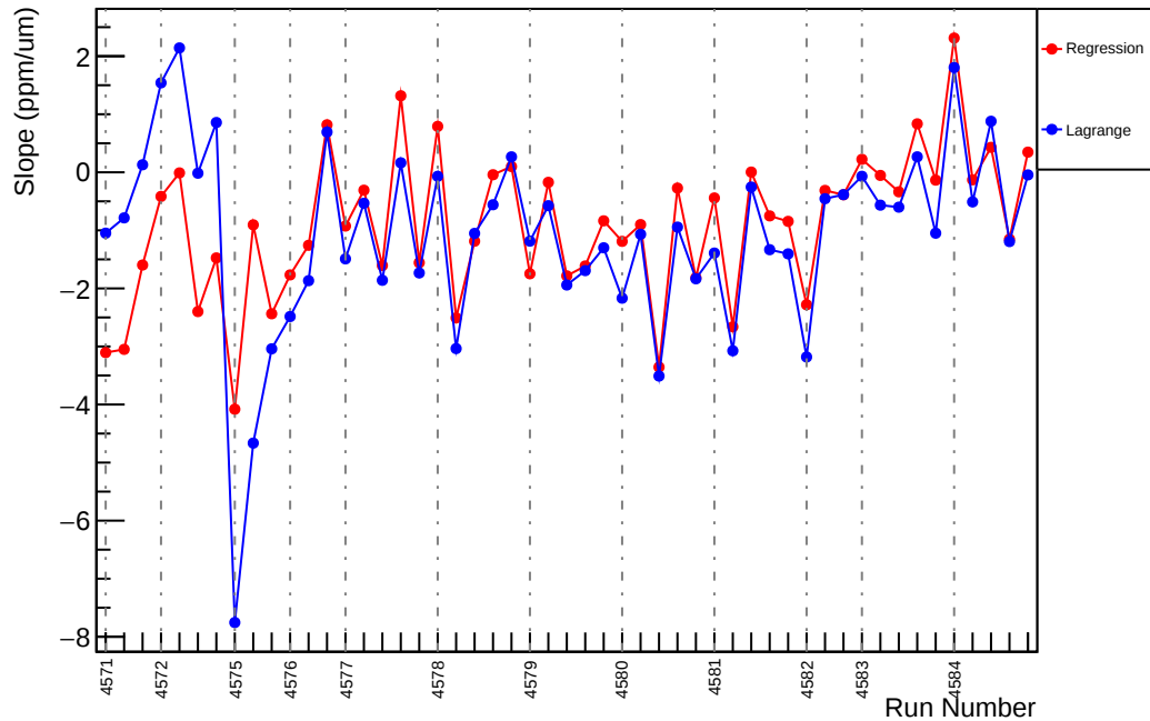
Slug69: Slope : usl_vs_evMon5 (ppm/um)
