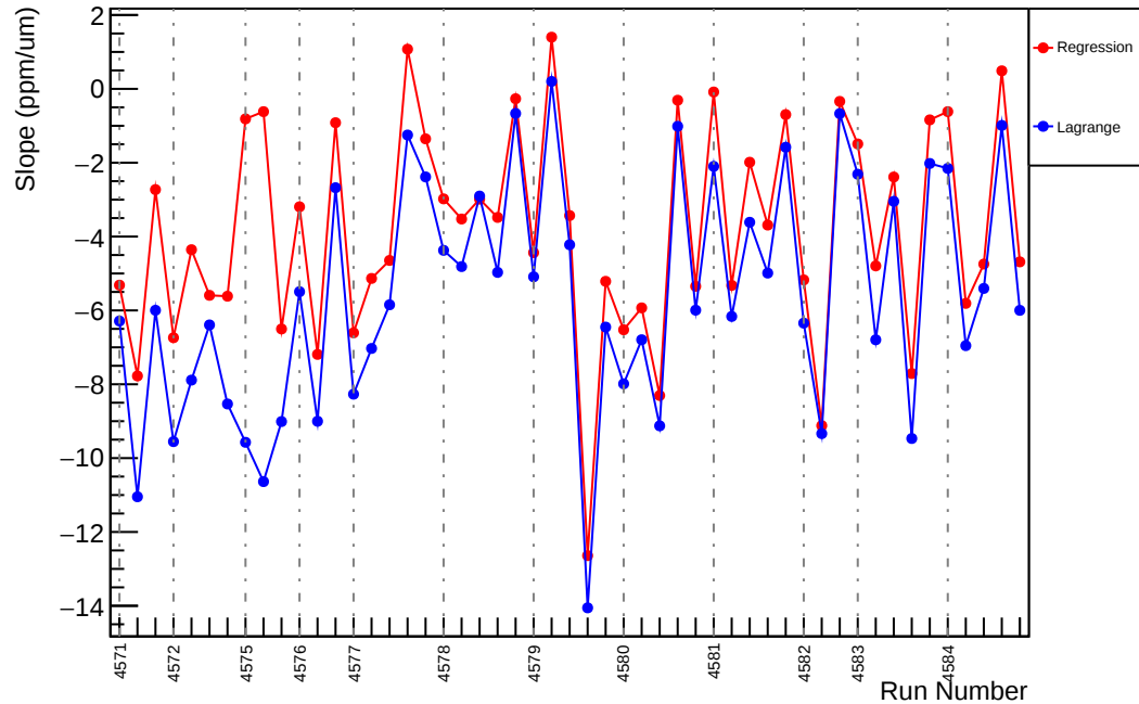
Slug69: Slope : usl_vs_evMon8 (ppm/um)
