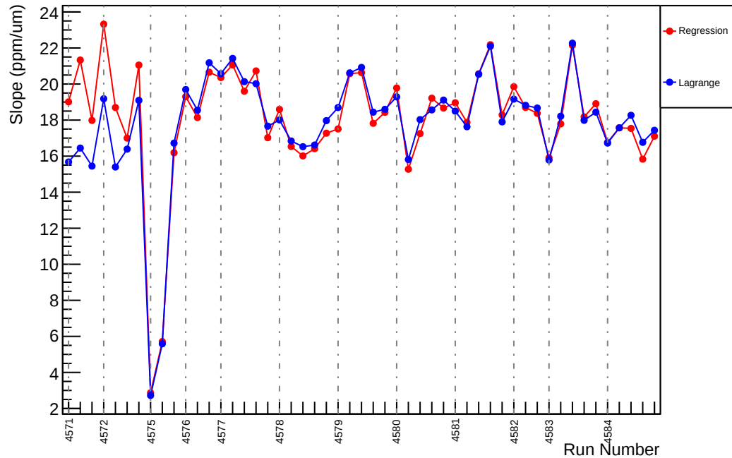
Slug69: Slope : usl_vs_evMon6 (ppm/um)
