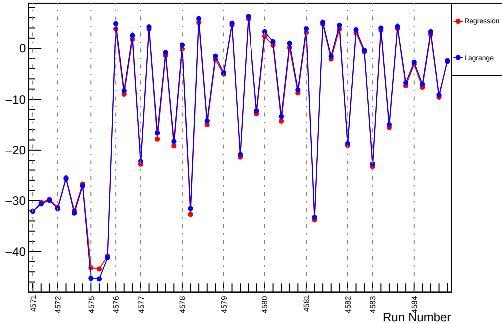
Slug69: Slope : usr_vs_evMon0 (ppm/um)
