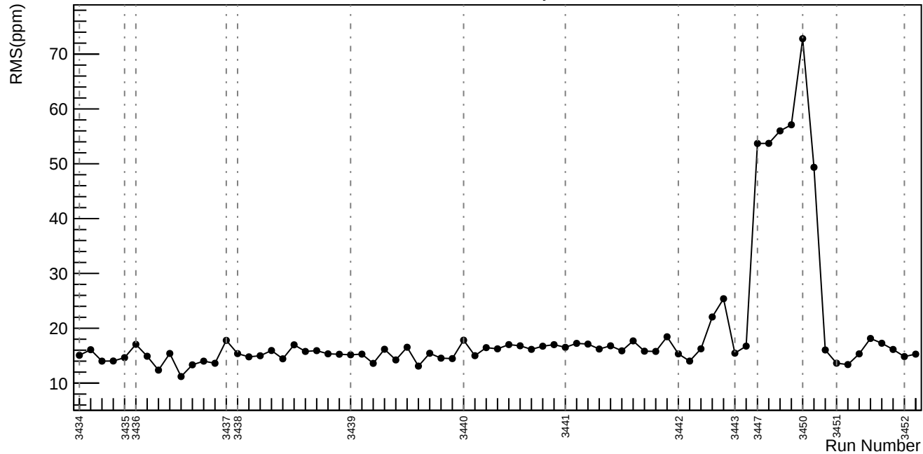
Slug6: asym_us_avg: \sqrt{\sigma_{\text{dit}}^2 - \sigma_{\text{reg}}^2} (ppm)
