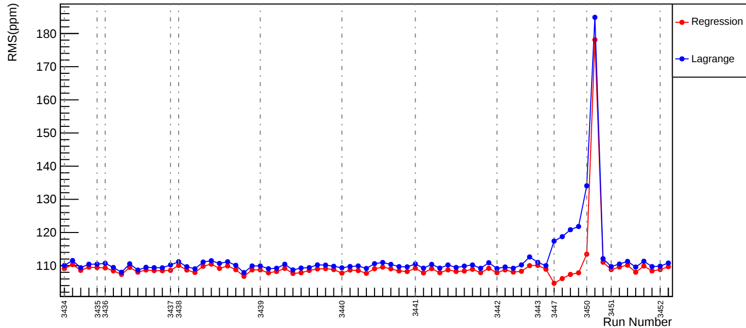
Slug6: Corrected RMS (ppm): asym_us_avg
