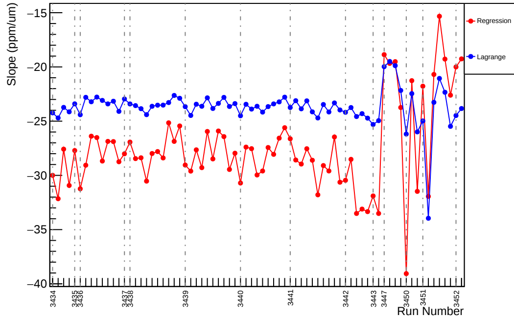
Slug6: Slope : us_avg_vs_evMon4 (ppm/um)
