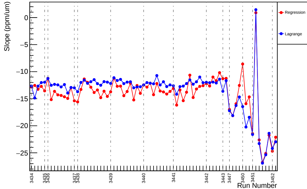
Slug6: Slope : us_avg_vs_evMon3 (ppm/um)
