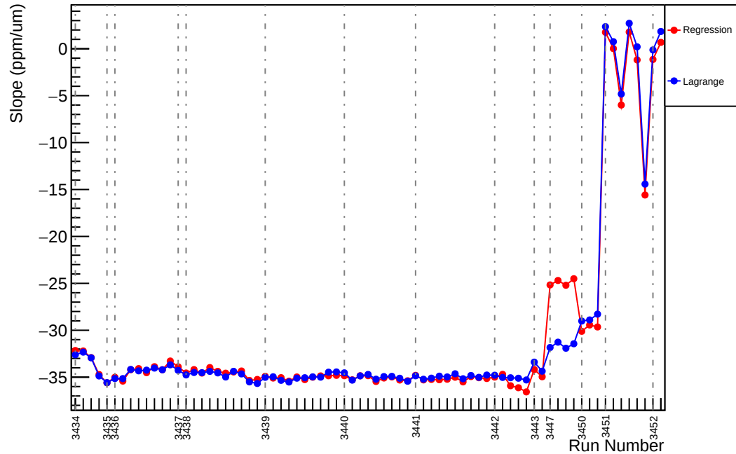
Slug6: Slope : us_avg_vs_evMon1 (ppm/um)
