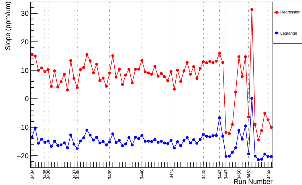
Slug6: Slope : us_dd_vs_evMon3 (ppm/um)
