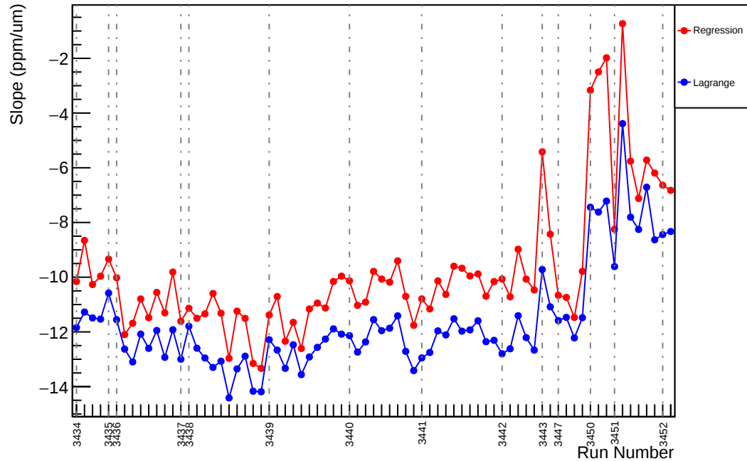
Slug6: Slope : us_dd_vs_evMon1 (ppm/um)
