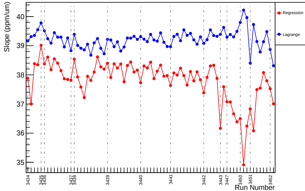
Slug6: Slope : us_dd_vs_evMon0 (ppm/um)
