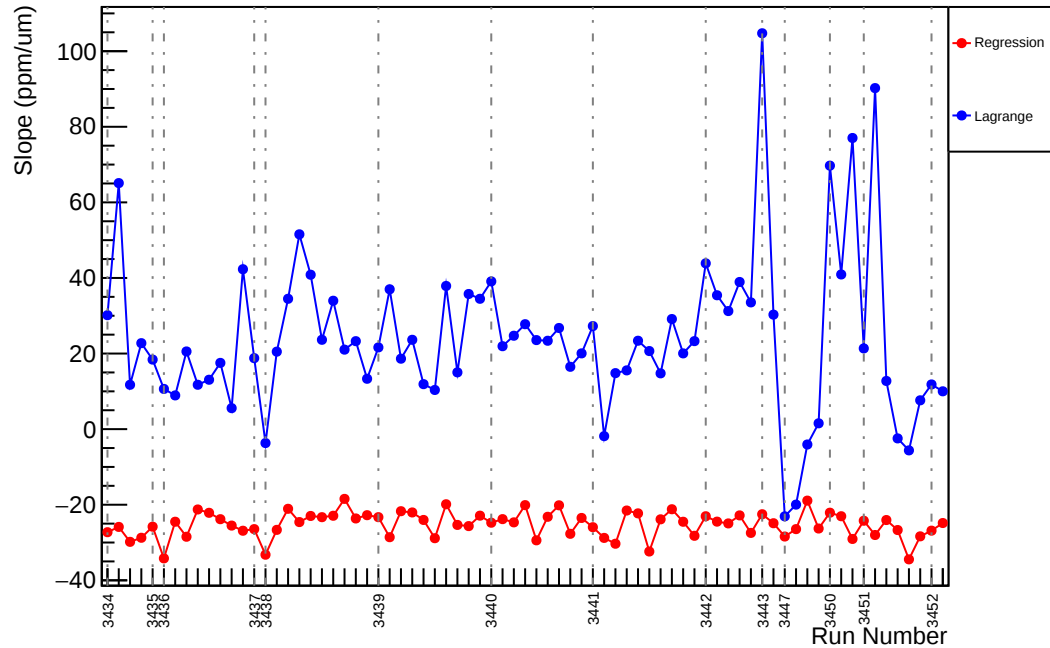
Slug6: Slope : us_dd_vs_evMon5 (ppm/um)
