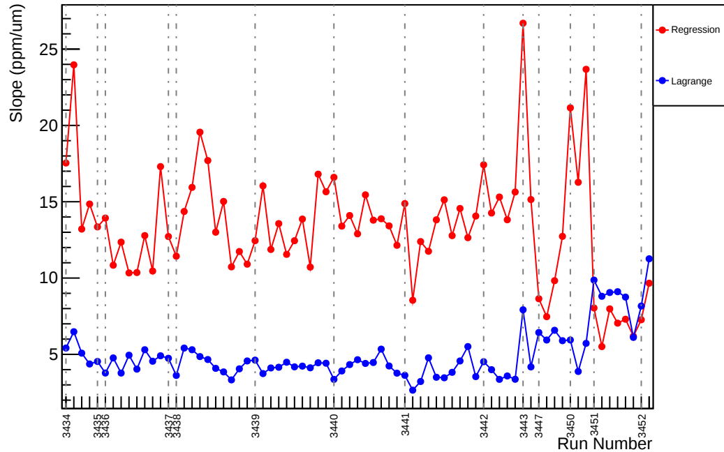
Slug6: Slope : us_dd_vs_evMon2 (ppm/um)
