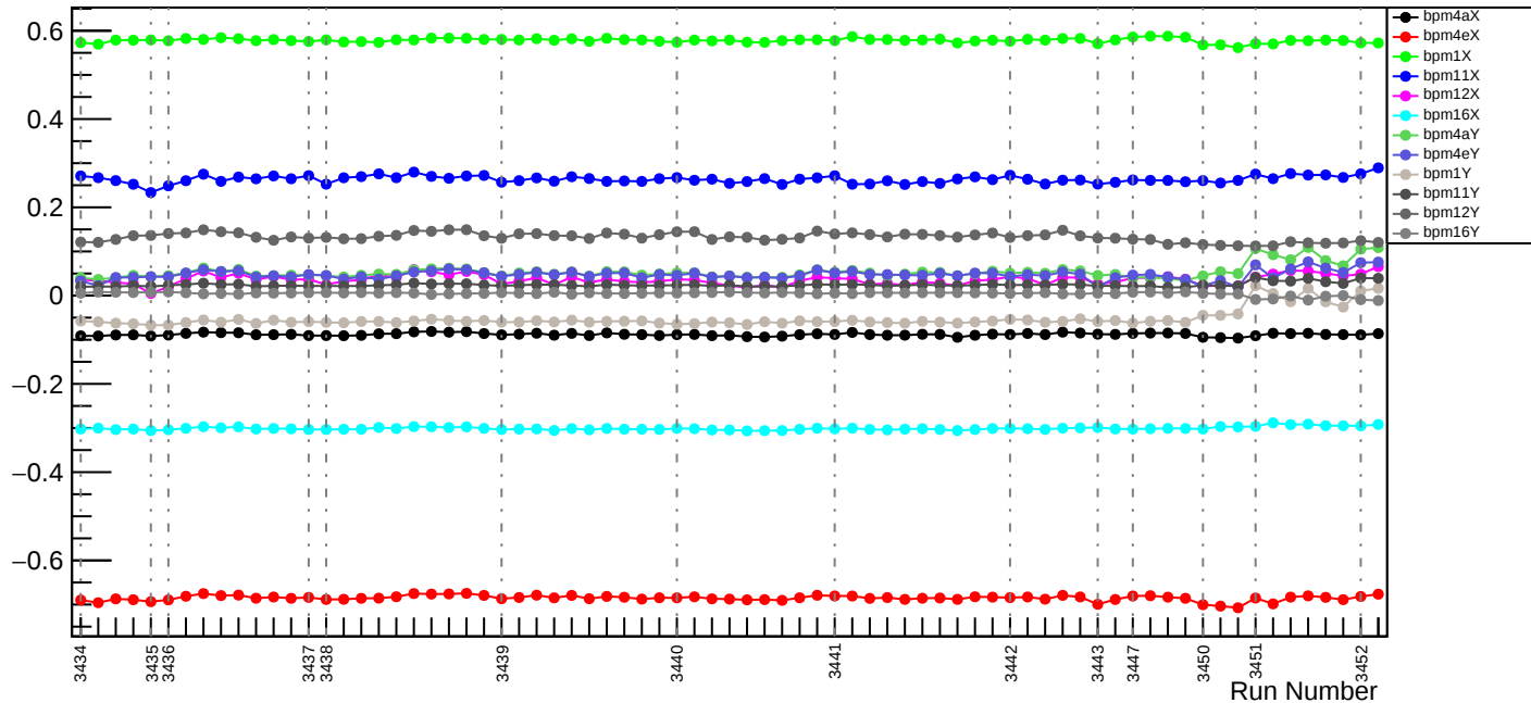
Slug6: EigenVector #0
