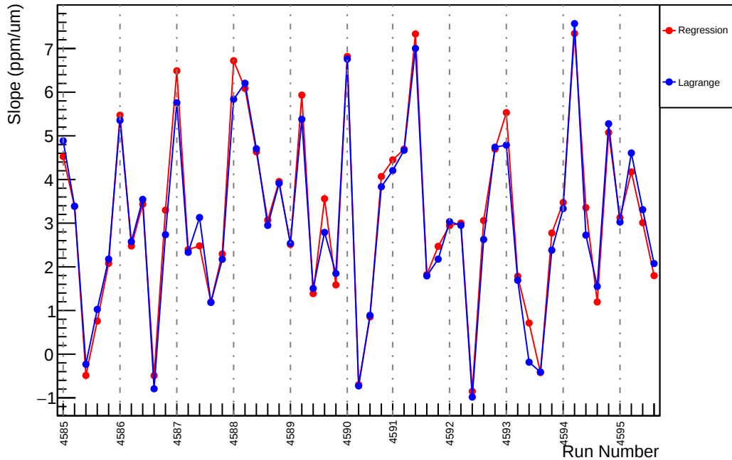
Slug70: Slope : us_dd_vs_evMon8 (ppm/um)
