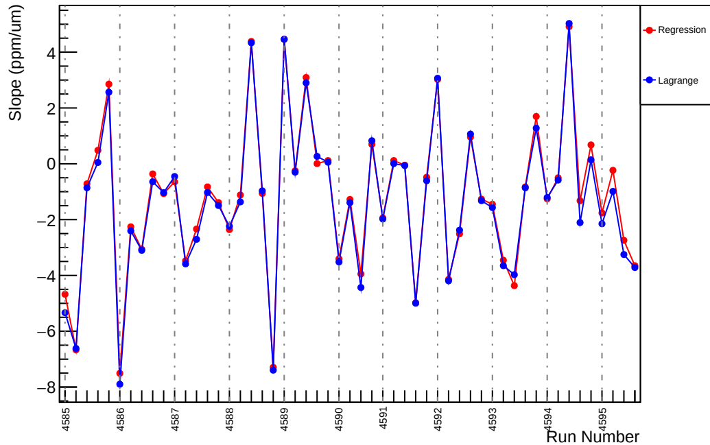
Slug70: Slope : us_dd_vs_evMon9 (ppm/um)
