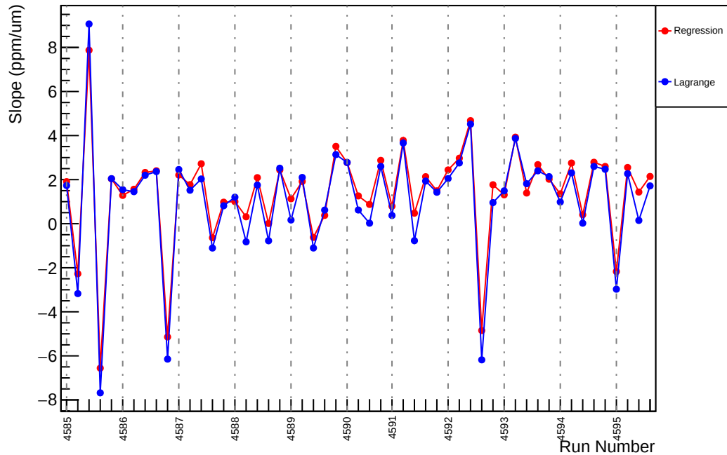
Slug70: Slope : us_dd_vs_evMon4 (ppm/um)
