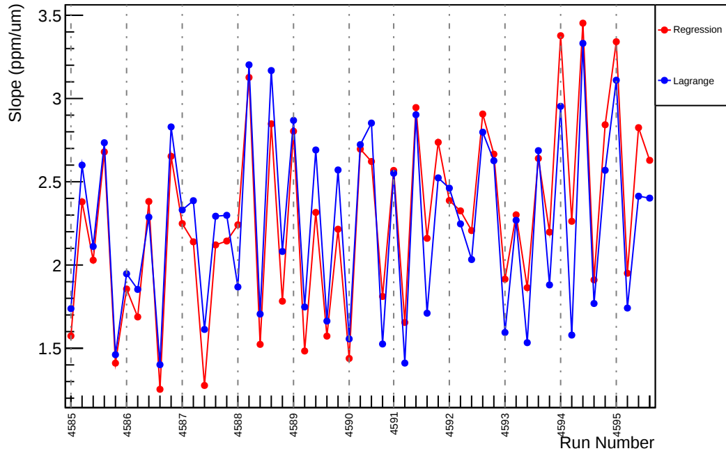
Slug70: Slope : us_dd_vs_evMon2 (ppm/um)
