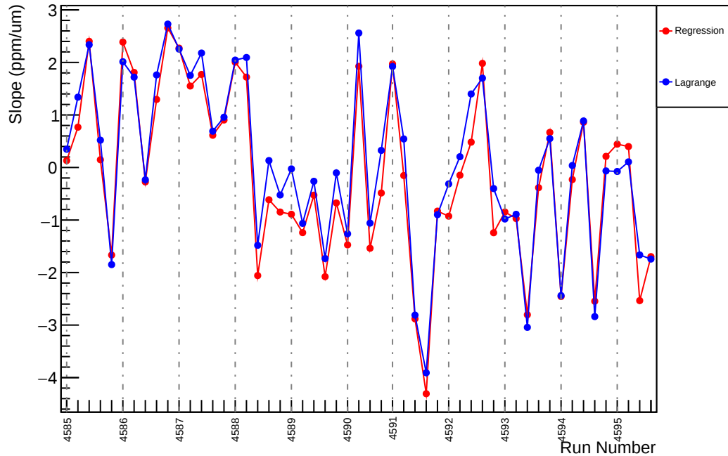
Slug70: Slope : us_dd_vs_evMon6 (ppm/um)
