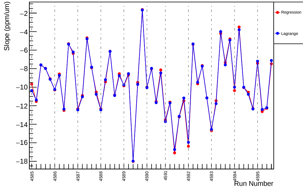
Slug70: Slope : us_dd_vs_evMon11 (ppm/um)
