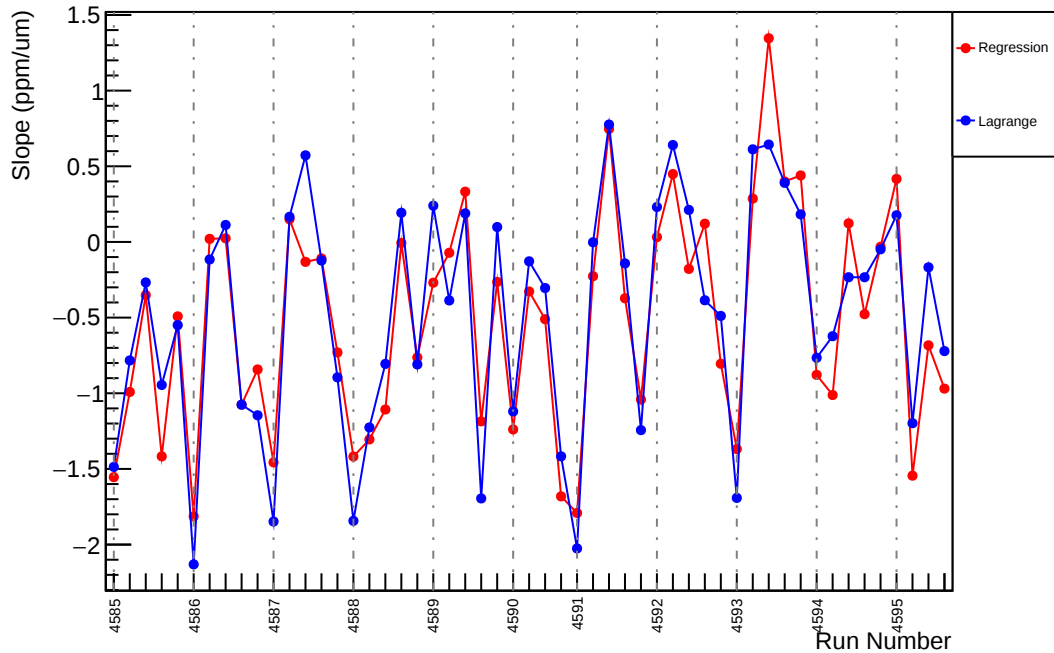
Slug70: Slope : us_dd_vs_evMon5 (ppm/um)
