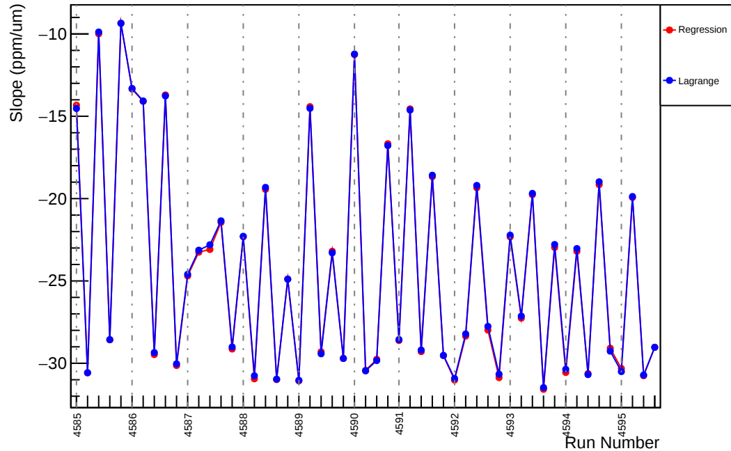
Slug70: Slope : us_dd_vs_evMon0 (ppm/um)
