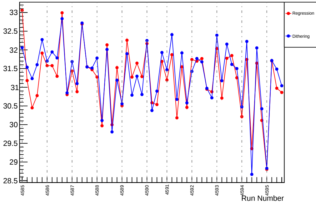
Slug70: Slope : usr_vs_evMon2 (ppm/um)
