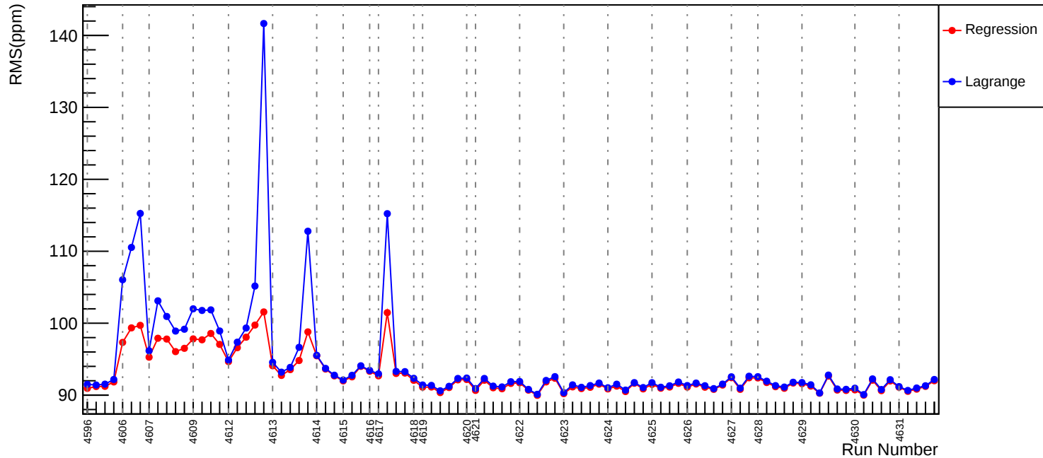
Slug71: Corrected RMS (ppm): asym_us_dd
