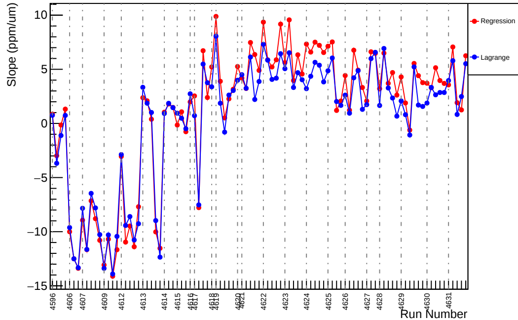
Slug71: Slope : us_dd_vs_evMon8 (ppm/um)
