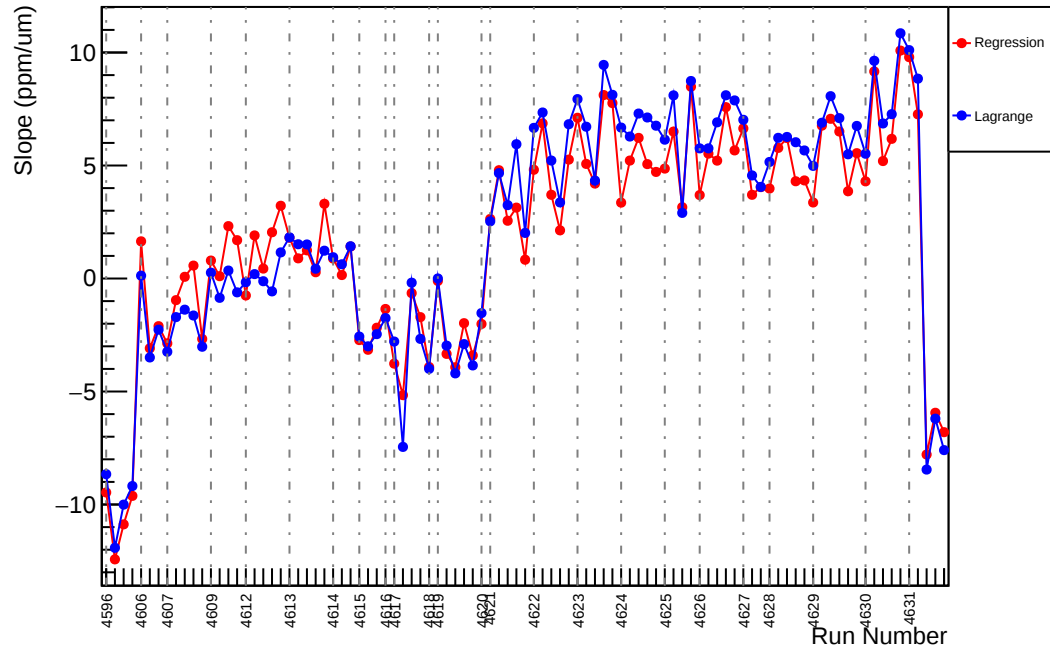
Slug71: Slope : us_dd_vs_evMon7 (ppm/um)
