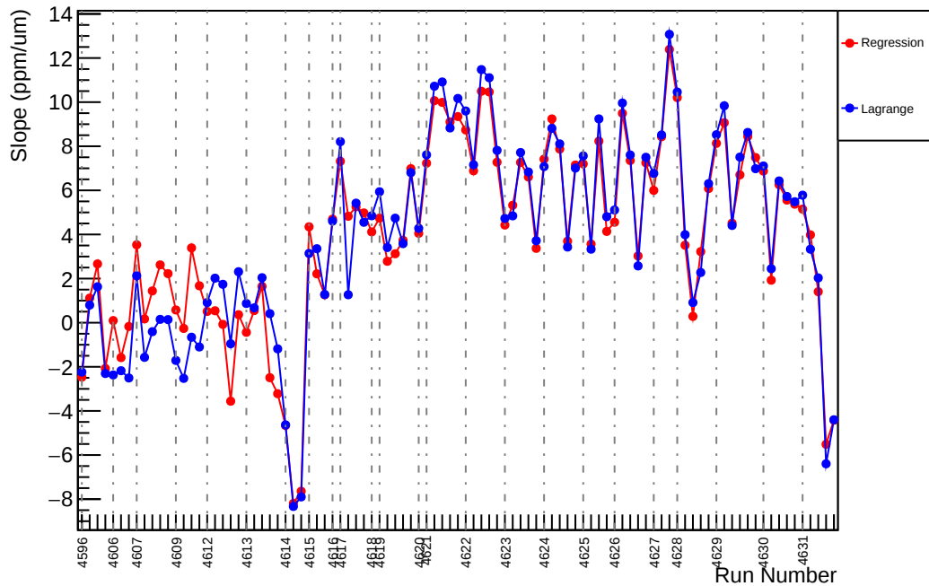
Slug71: Slope : us_dd_vs_evMon6 (ppm/um)
