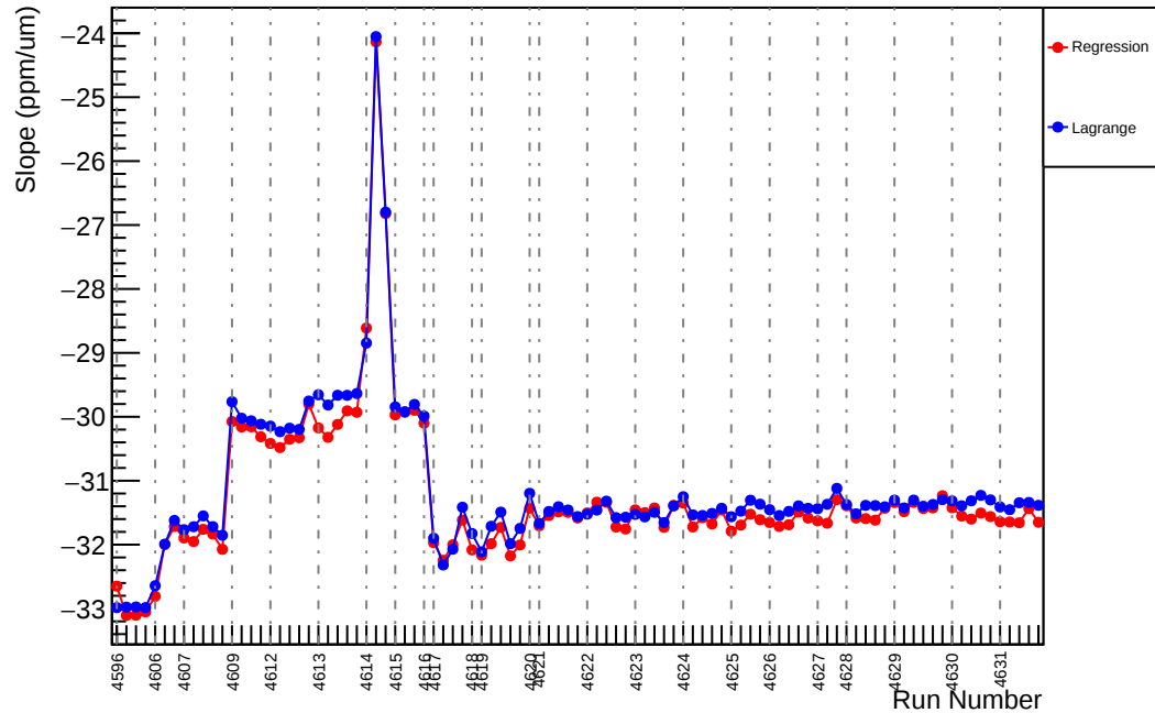
Slug71: Slope : us_dd_vs_evMon0 (ppm/um)
