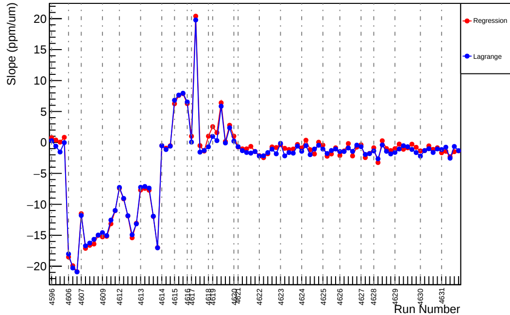
Slug71: Slope : us_dd_vs_evMon5 (ppm/um)
