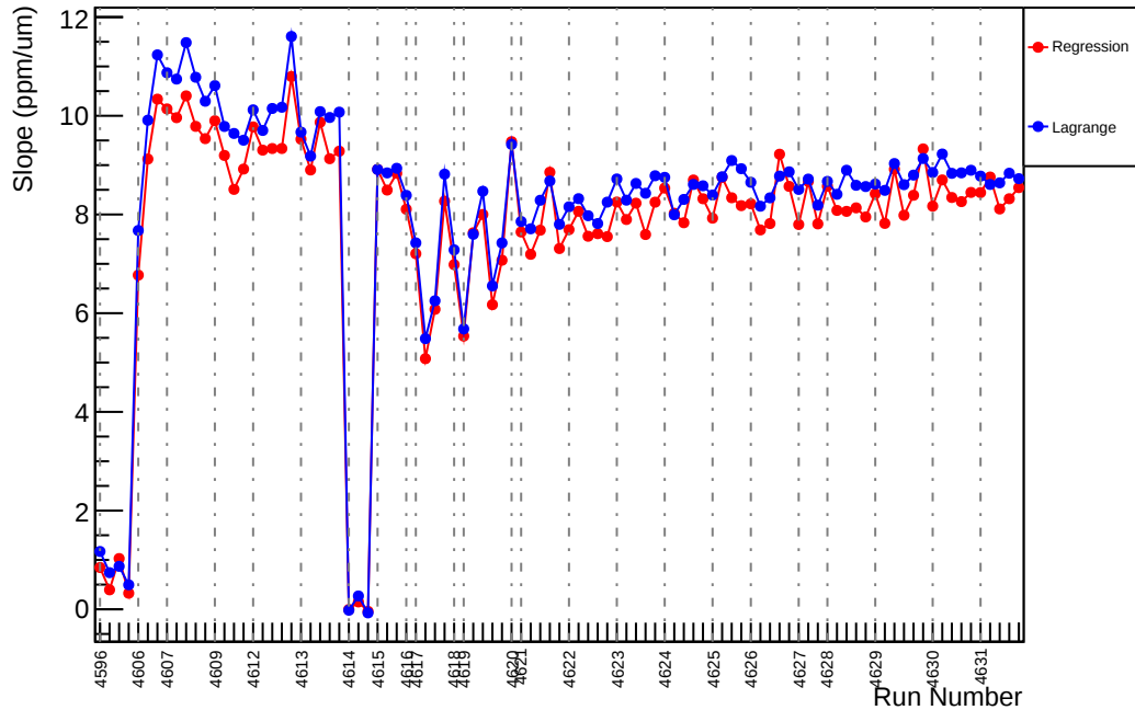
Slug71: Slope : us_dd_vs_evMon2 (ppm/um)
