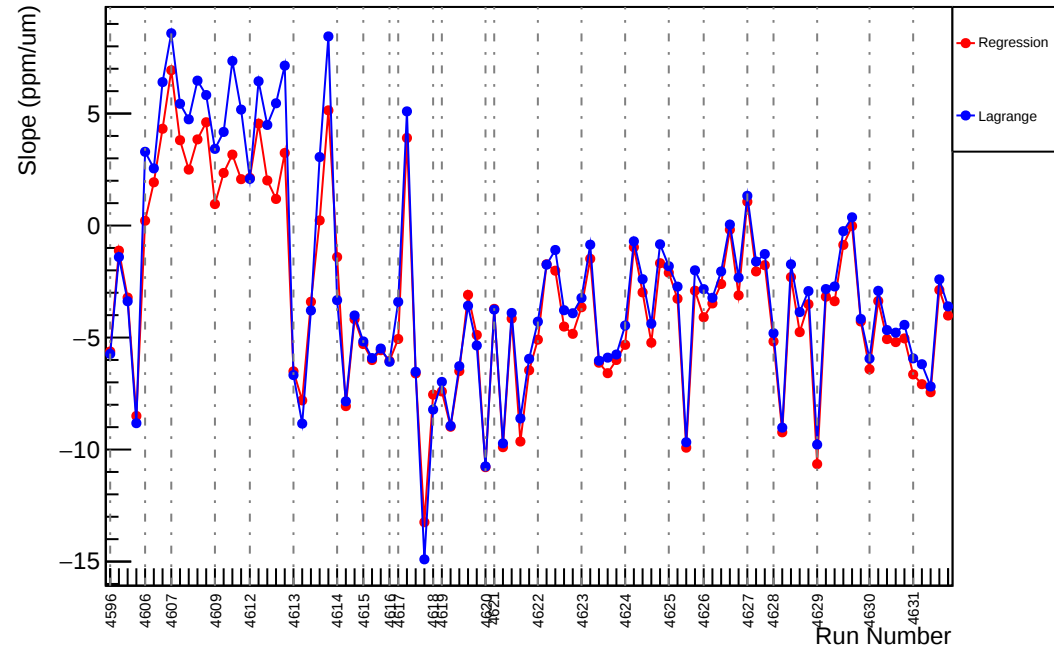
Slug71: Slope : us_dd_vs_evMon10 (ppm/um)
