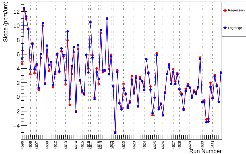
Slug71: Slope : us_dd_vs_evMon11 (ppm/um)
