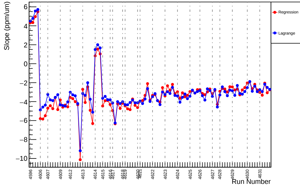
Slug71: Slope : us_dd_vs_evMon3 (ppm/um)
