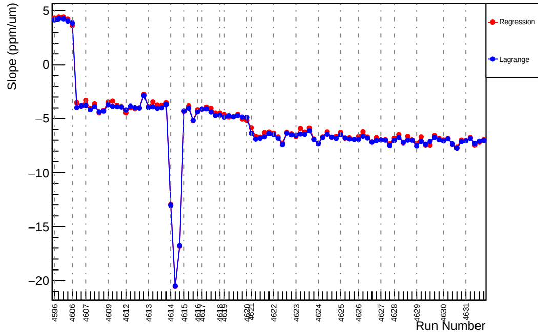
Slug71: Slope : us_dd_vs_evMon1 (ppm/um)
