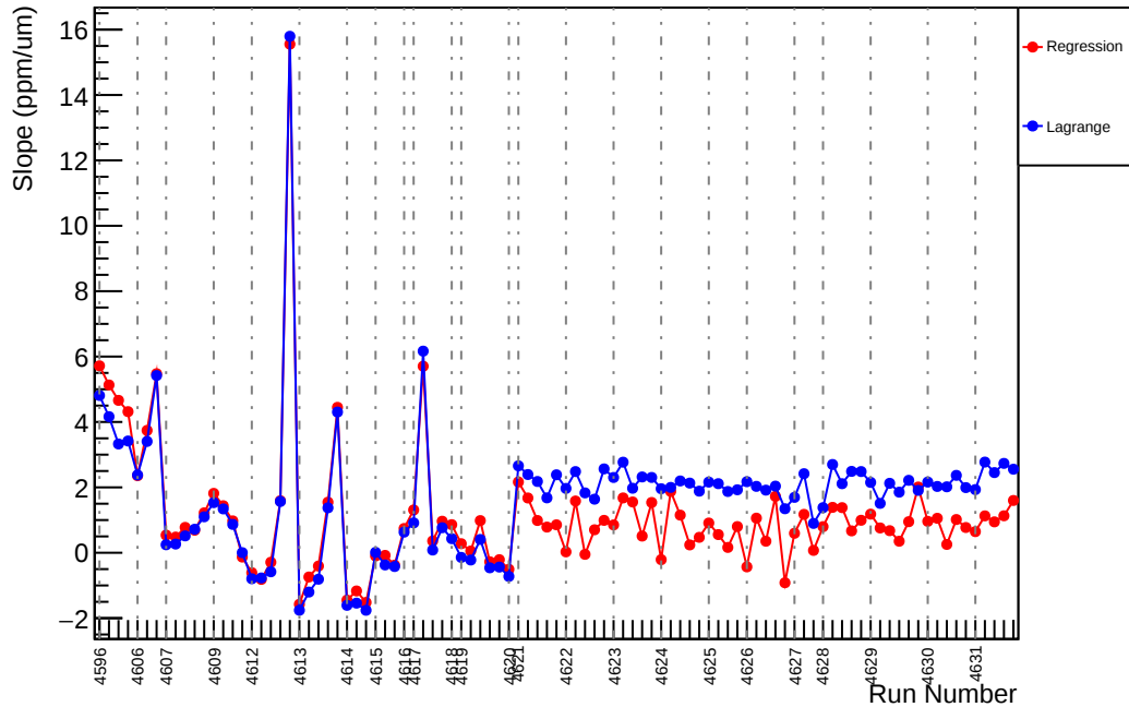
Slug71: Slope : us_dd_vs_evMon4 (ppm/um)
