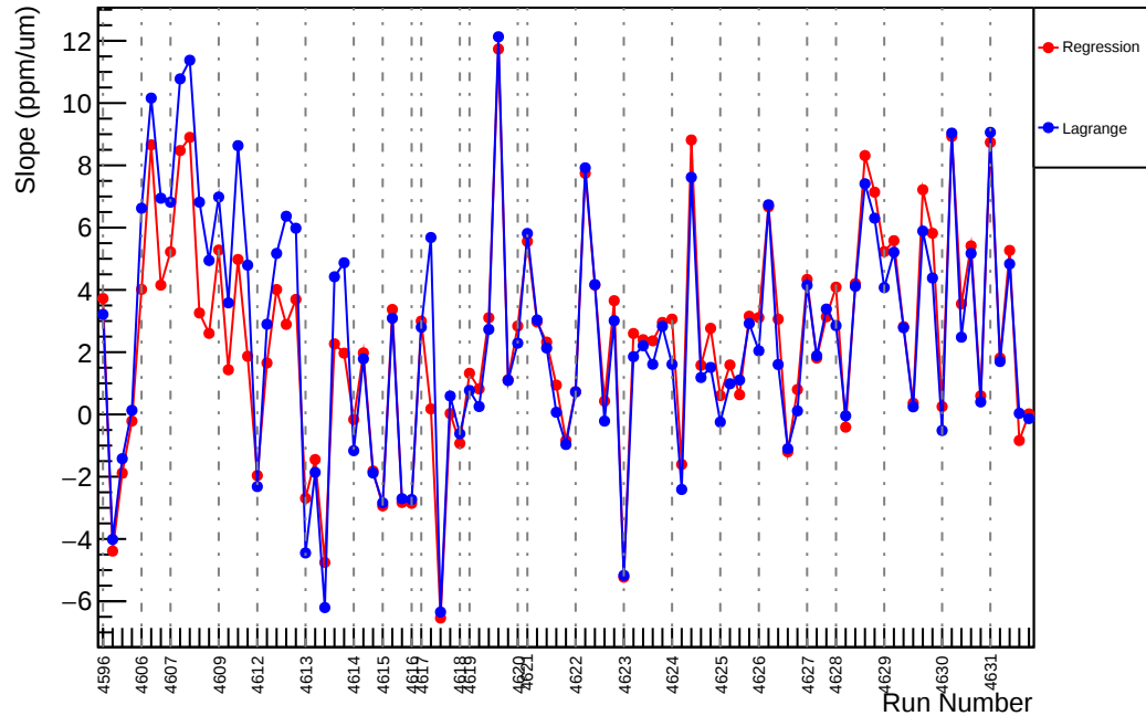
Slug71: Slope : us_dd_vs_evMon9 (ppm/um)
