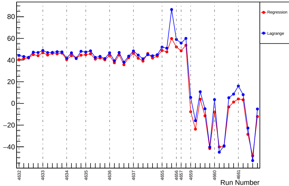
Slug72: Slope : usl_vs_evMon4 (ppm/um)
