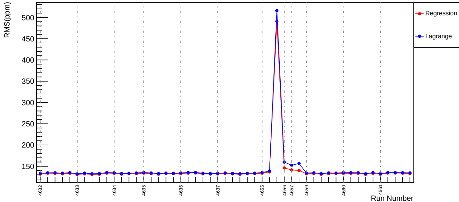
Slug72: Corrected RMS (ppm): asym_usl
