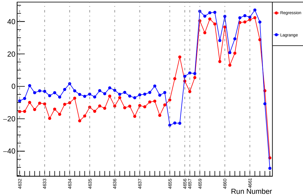
Slug72: Slope : usl_vs_evMon5 (ppm/um)
