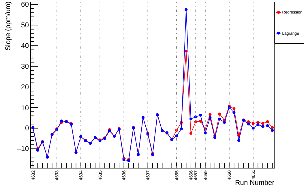
Slug72: Slope : usr_vs_evMon11 (ppm/um)
