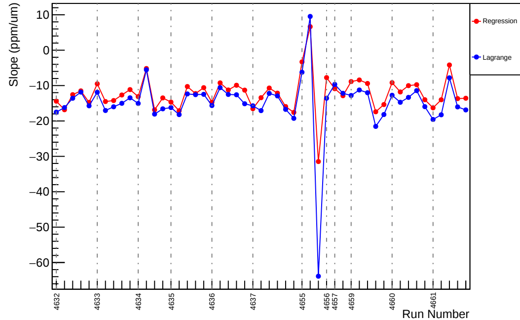
Slug72: Slope : usr_vs_evMon9 (ppm/um)
