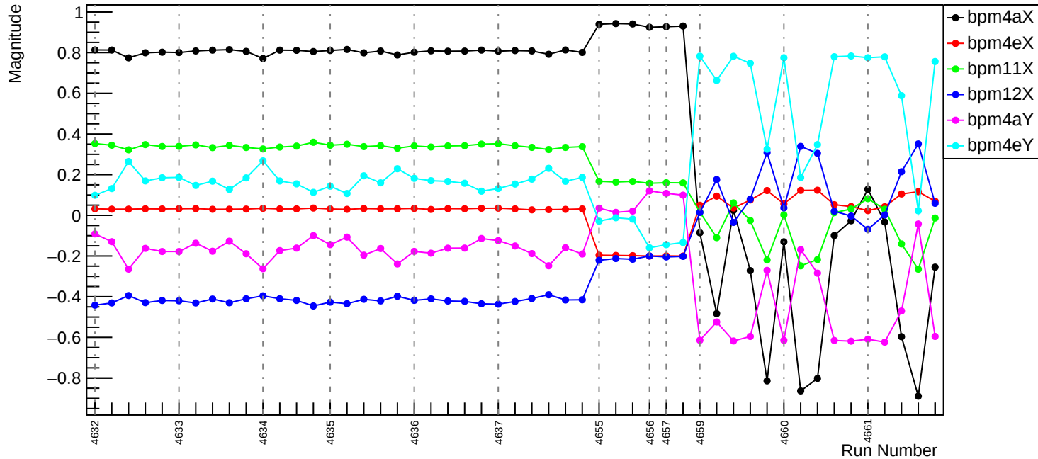
Slug72: EigenVector #4
