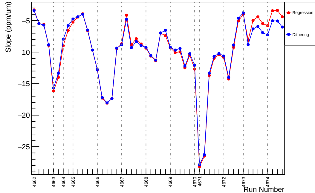
Slug73: Slope : us_avg_vs_evMon0 (ppm/um)
