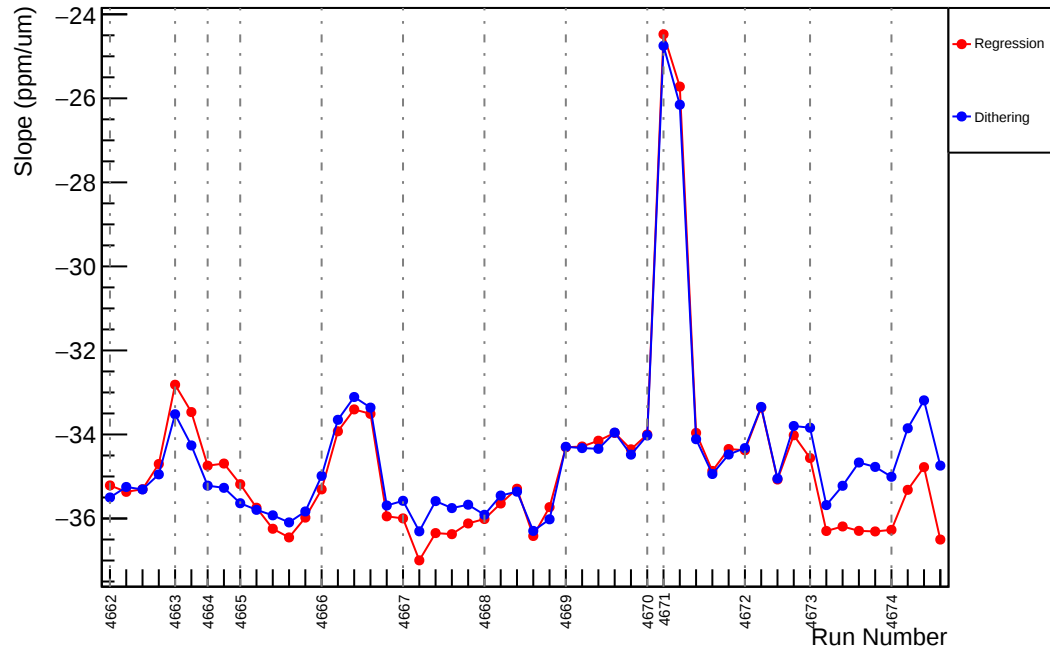
Slug73: Slope : us_avg_vs_evMon1 (ppm/um)
