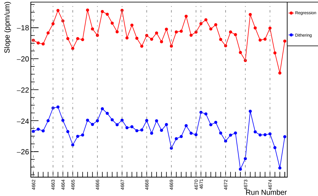
Slug73: Slope : us_avg_vs_evMon2 (ppm/um)
