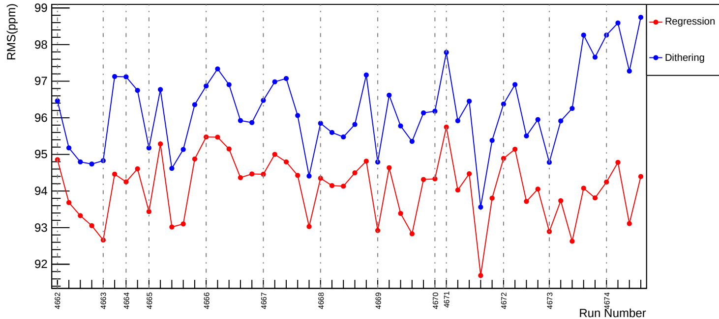
Slug73: Corrected RMS (ppm): asym_us_avg
