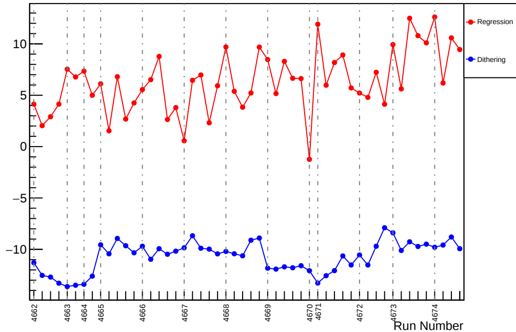
Slug73: Slope : us_avg_vs_evMon4 (ppm/um)
