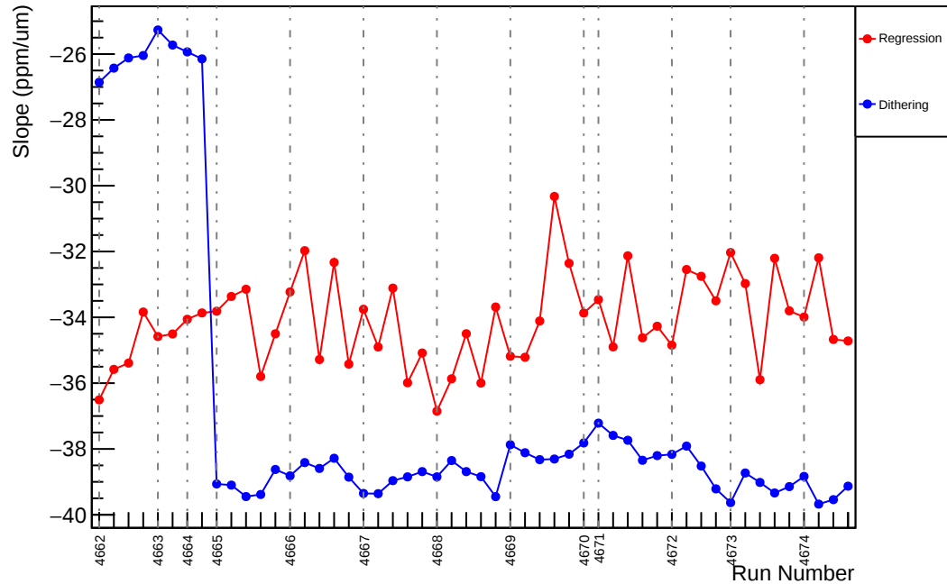
Slug73: Slope : us_avg_vs_evMon3 (ppm/um)
