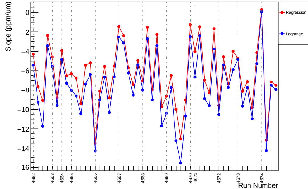
Slug73: Slope : us_avg_vs_evMon11 (ppm/um)
