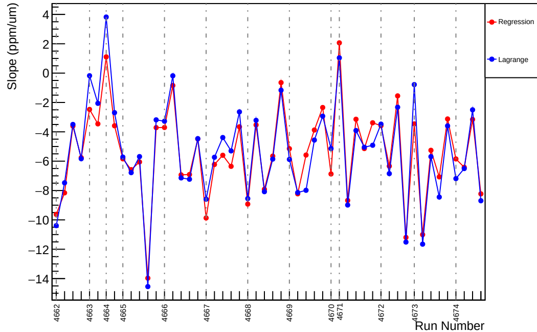
Slug73: Slope : us_avg_vs_evMon10 (ppm/um)
