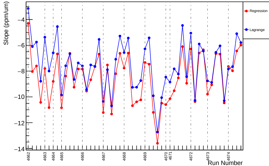
Slug73: Slope : us_avg_vs_evMon6 (ppm/um)
