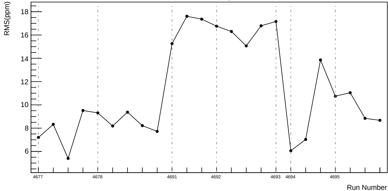
Slug74: asym_us_dd: \sqrt{\sigma_{\text{dit}}^2 - \sigma_{\text{reg}}^2} (ppm)
