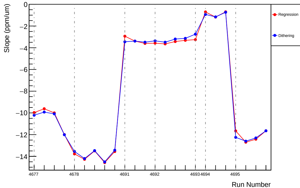
Slug74: Slope : us_dd_vs_evMon1 (ppm/um)
