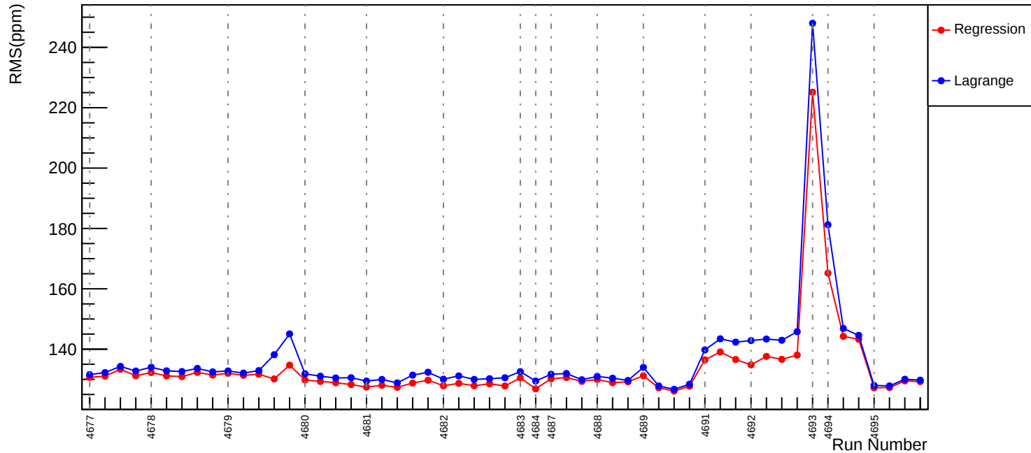
Slug74: Corrected RMS (ppm): asym_usl
