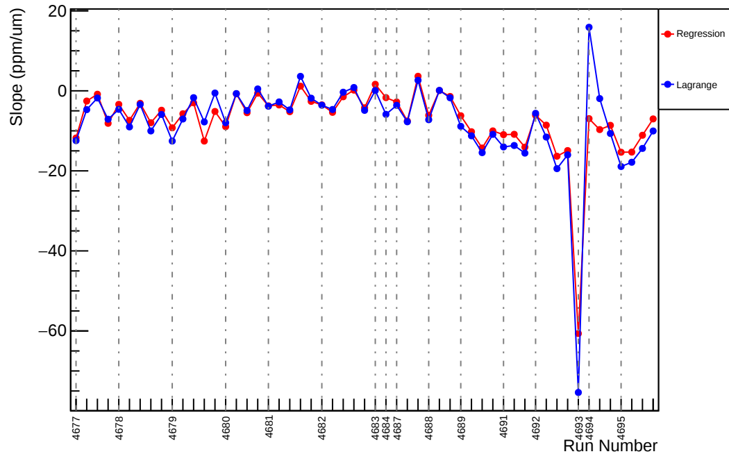
Slug74: Slope : usl_vs_evMon9 (ppm/um)
