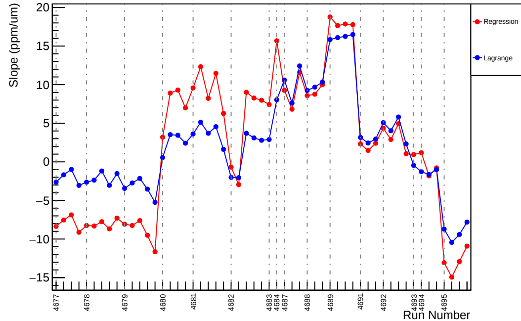
Slug74: Slope : usl_vs_evMon4 (ppm/um)
