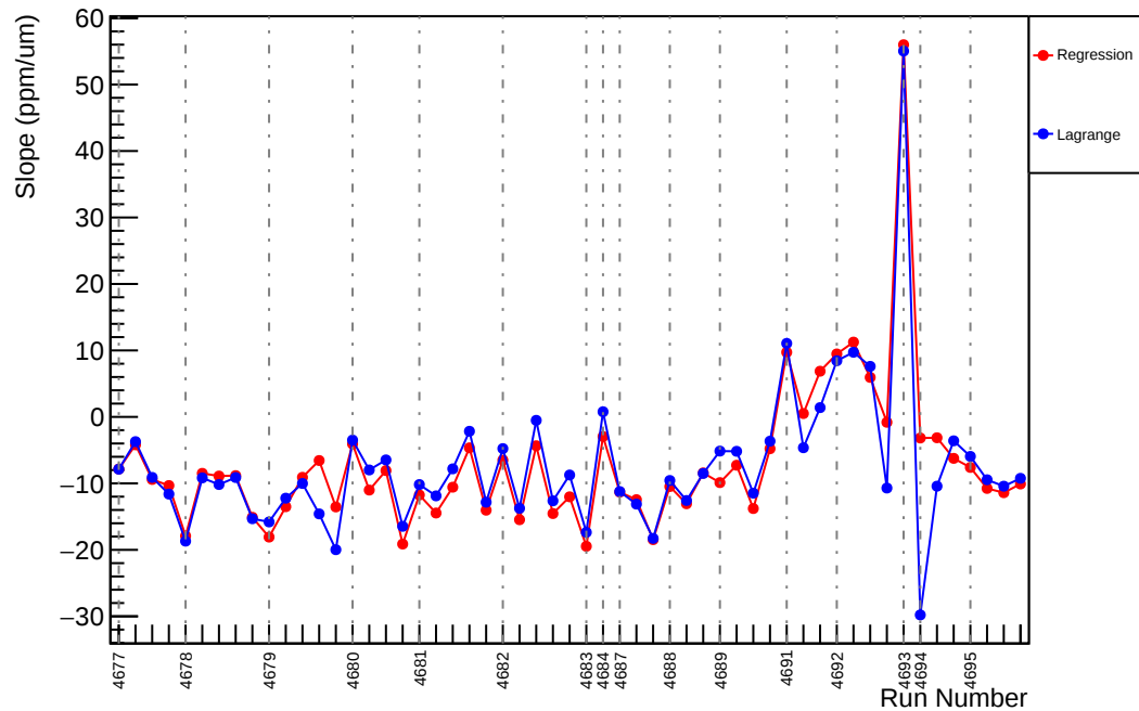
Slug74: Slope : usl_vs_evMon10 (ppm/um)
