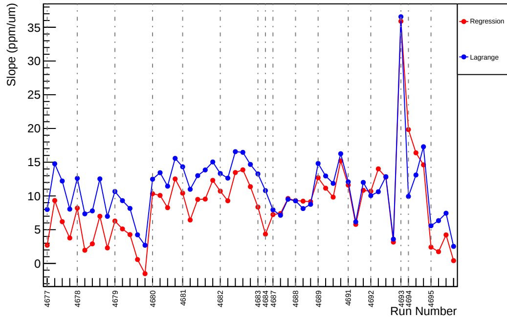
Slug74: Slope : usl_vs_evMon6 (ppm/um)
