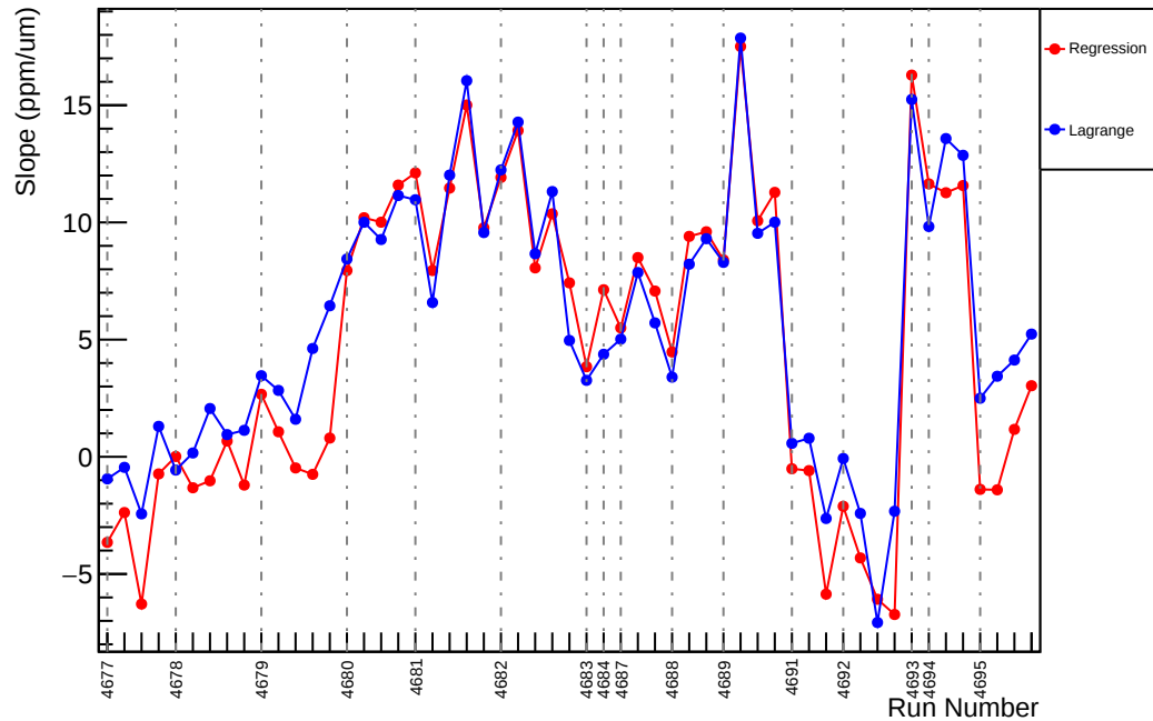
Slug74: Slope : usl_vs_evMon7 (ppm/um)
