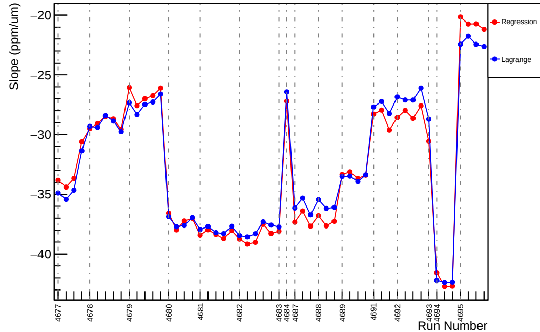
Slug74: Slope : usl_vs_evMon2 (ppm/um)
