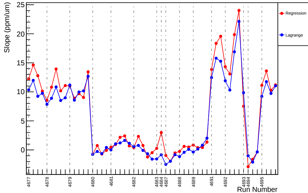
Slug74: Slope : usl_vs_evMon5 (ppm/um)
