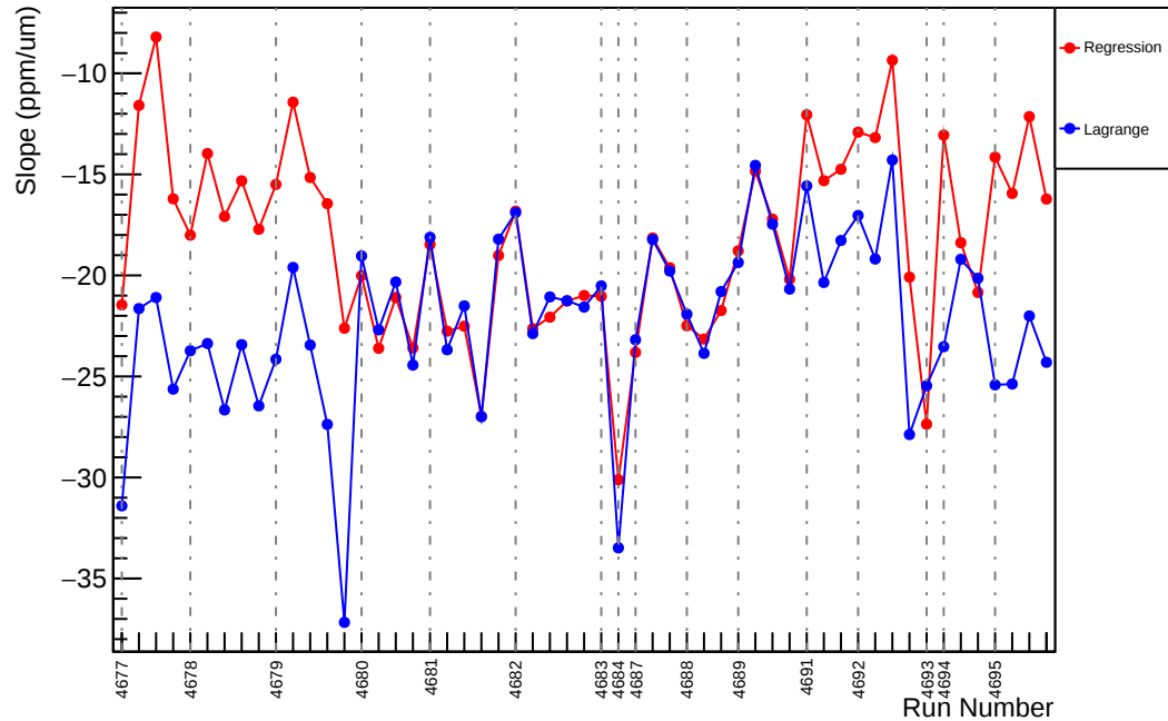
Slug74: Slope : usl_vs_evMon8 (ppm/um)
