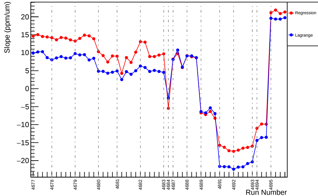
Slug74: Slope : usl_vs_evMon3 (ppm/um)
