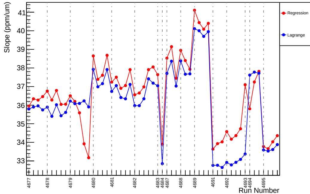
Slug74: Slope : usl_vs_evMon0 (ppm/um)
