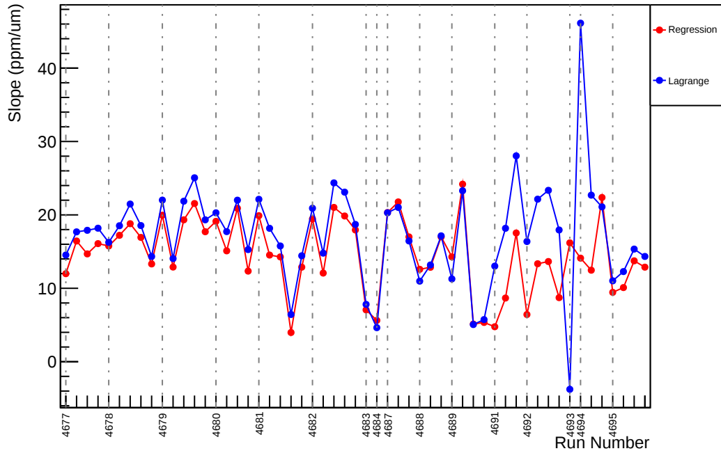
Slug74: Slope : usl_vs_evMon11 (ppm/um)
