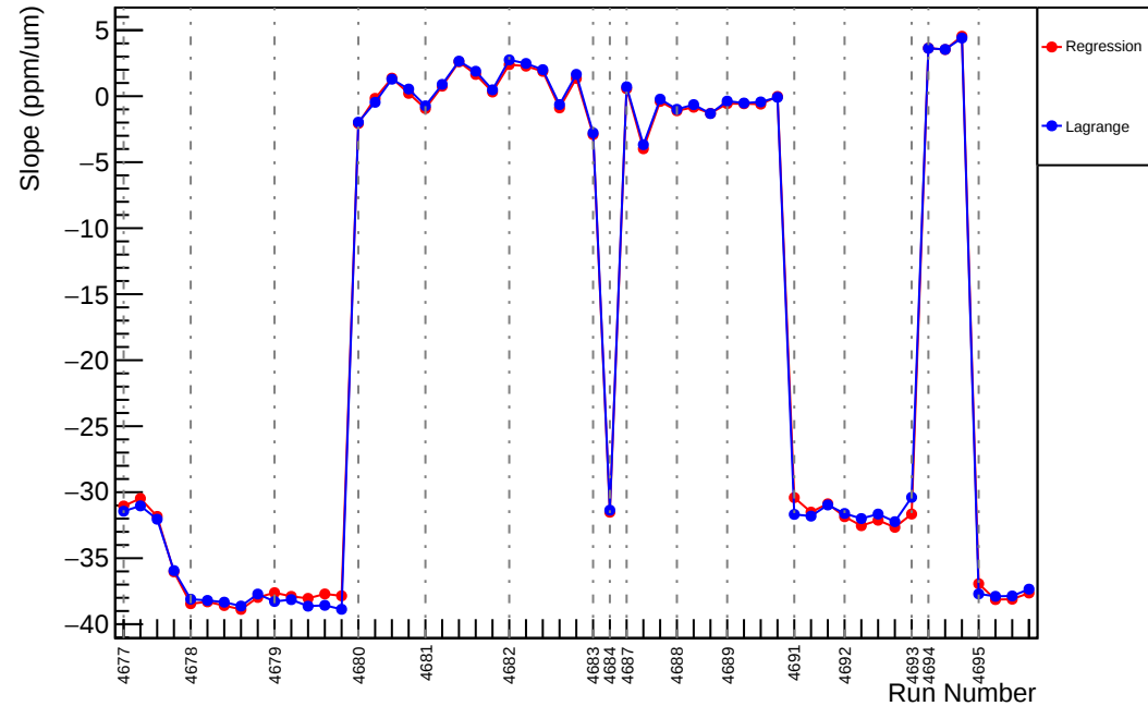
Slug74: Slope : usl_vs_evMon1 (ppm/um)
