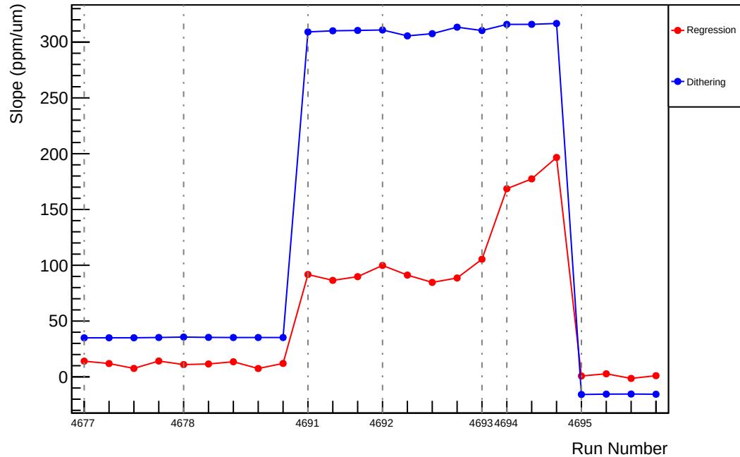
Slug74: Slope : usr_vs_evMon3 (ppm/um)
