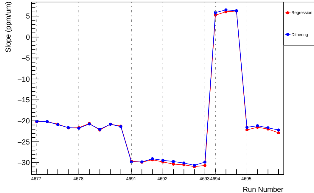
Slug74: Slope : usr_vs_evMon1 (ppm/um)
