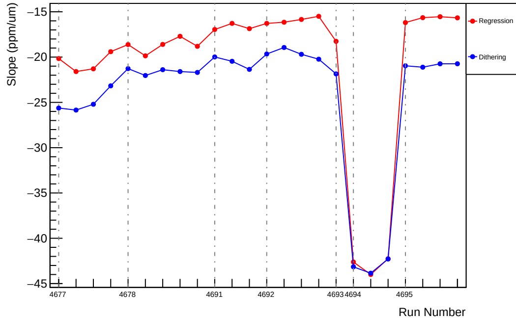
Slug74: Slope : usr_vs_evMon2 (ppm/um)
