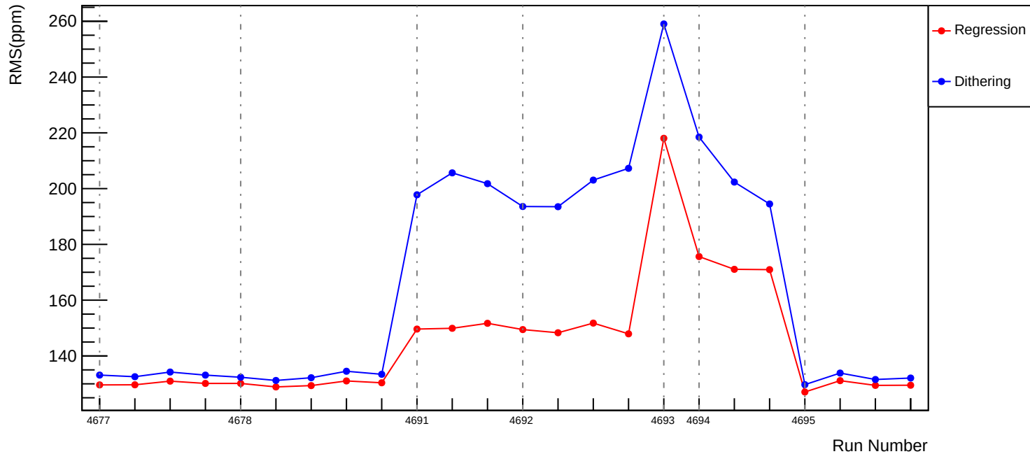
Slug74: Corrected RMS (ppm): asym_usr
