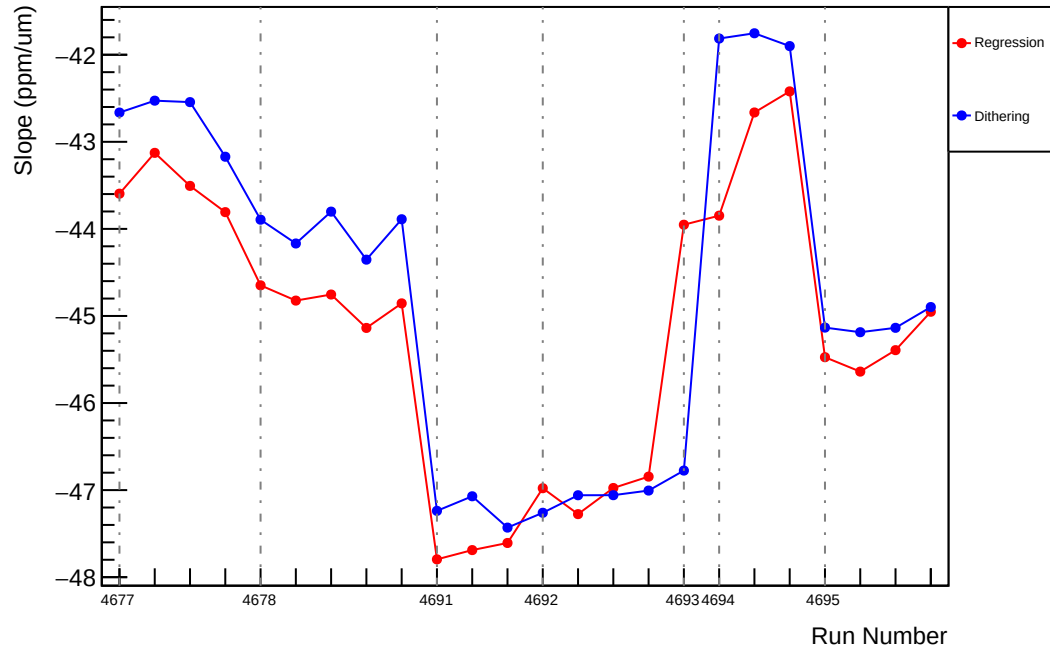
Slug74: Slope : usr_vs_evMon0 (ppm/um)
