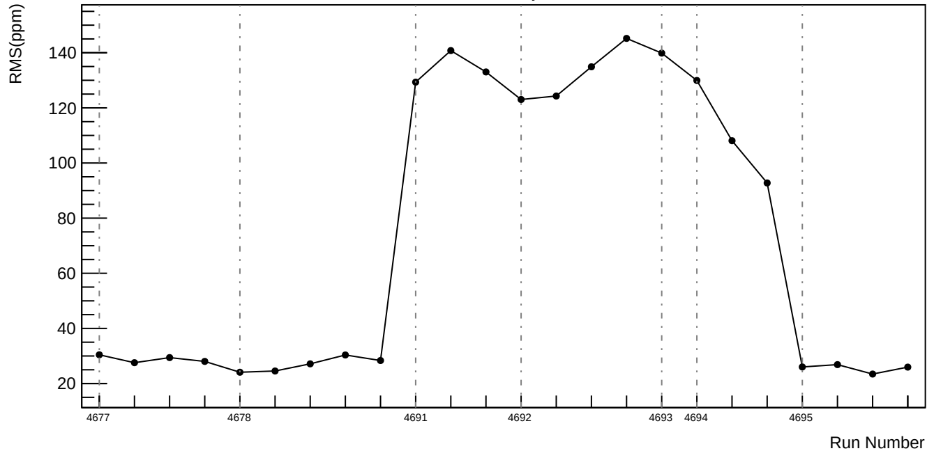
Slug74: asym_usr: \sqrt{\sigma_{\text{dit}}^2 - \sigma_{\text{reg}}^2} (ppm)
