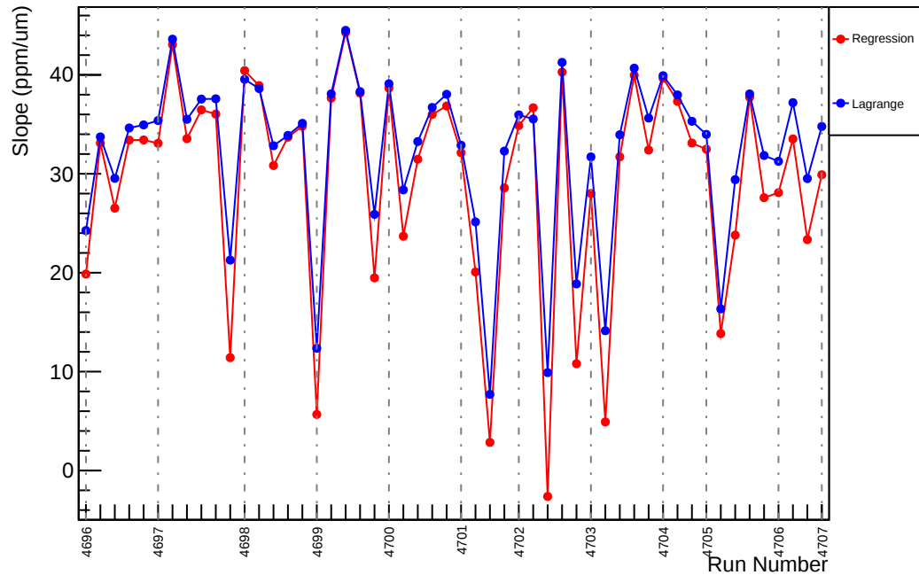
Slug75: Slope : us_dd_vs_evMon4 (ppm/um)
