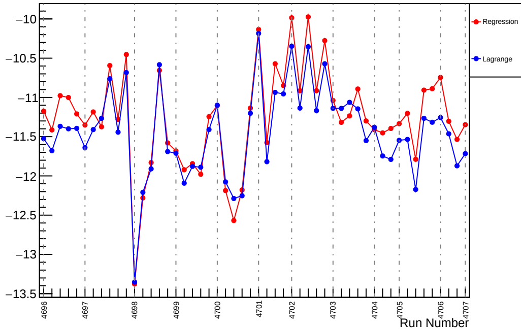
Slug75: Slope : us_dd_vs_evMon1 (ppm/um)
