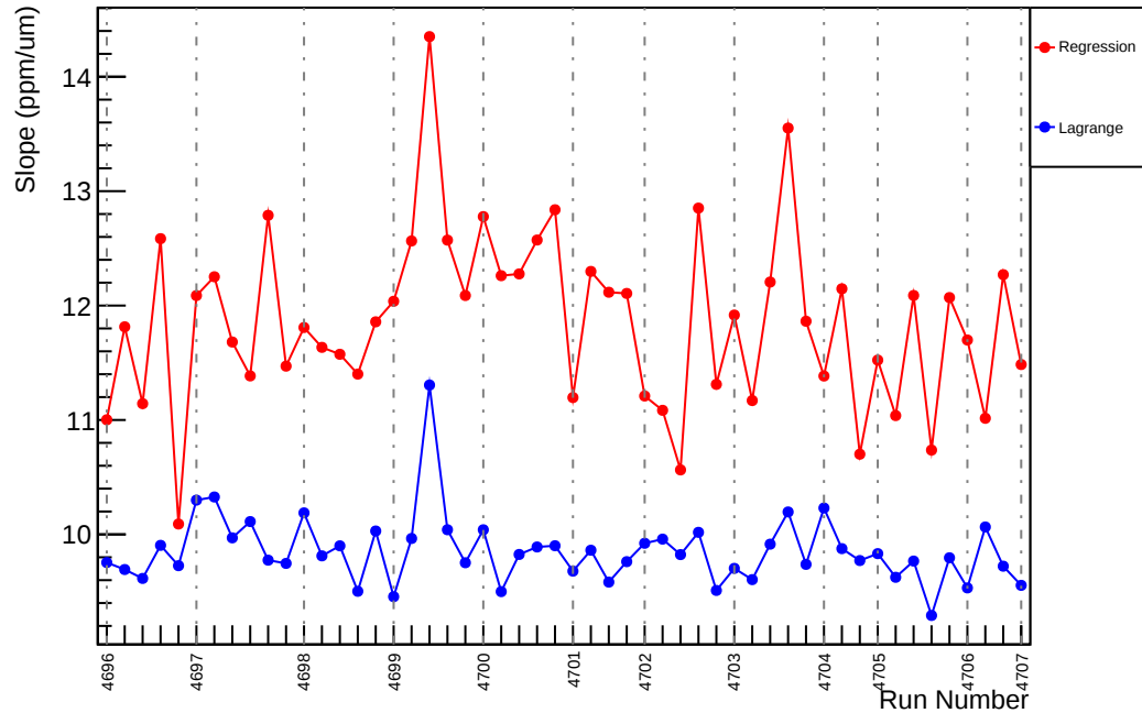
Slug75: Slope : us_dd_vs_evMon3 (ppm/um)
