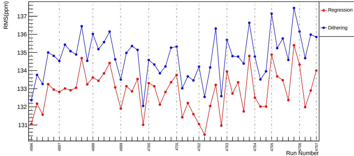
Slug75: Corrected RMS (ppm): asym_usl
