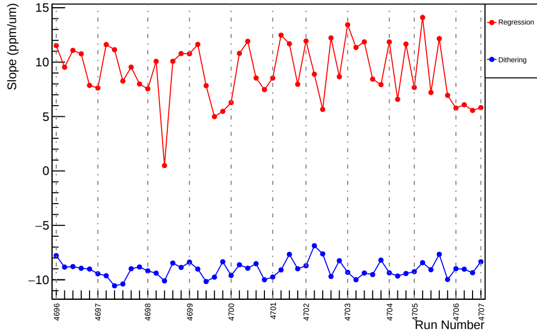
Slug75: Slope : usl_vs_evMon4 (ppm/um)
