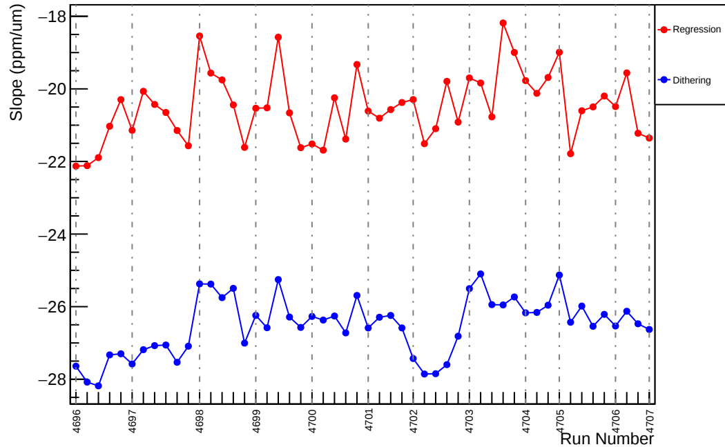
Slug75: Slope : usl_vs_evMon2 (ppm/um)
