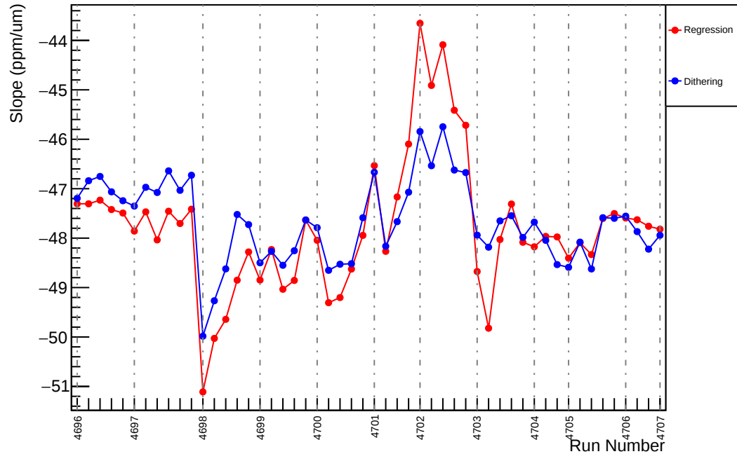
Slug75: Slope : usl_vs_evMon1 (ppm/um)
