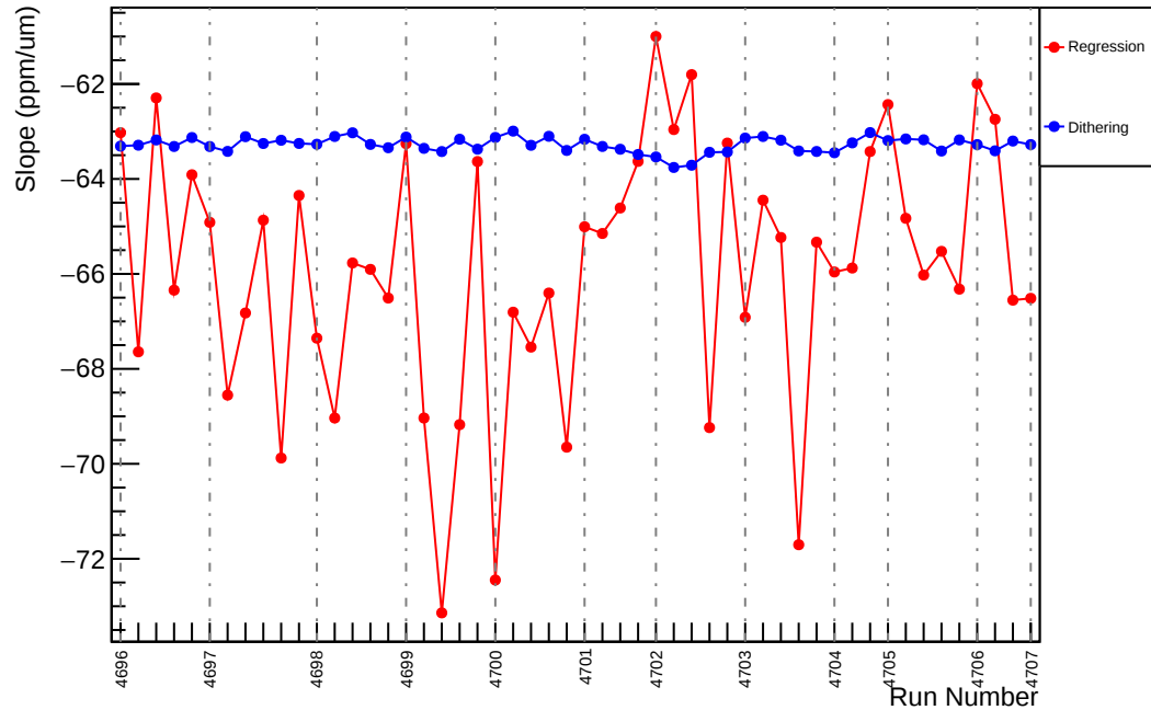
Slug75: Slope : usl_vs_evMon3 (ppm/um)
