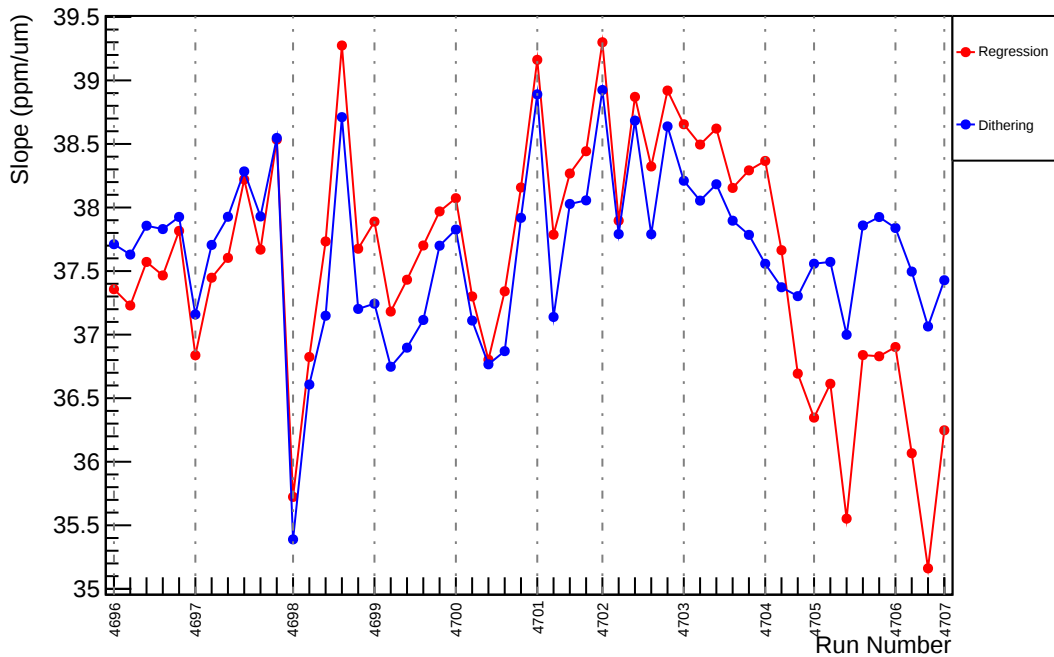
Slug75: Slope : usl_vs_evMon0 (ppm/um)
