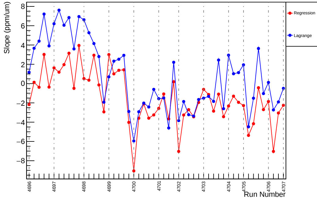
Slug75: Slope : usl_vs_evMon7 (ppm/um)
