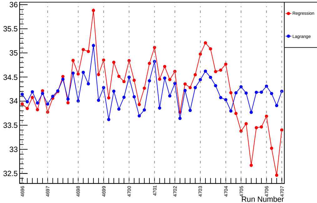
Slug75: Slope : usl_vs_evMon0 (ppm/um)
