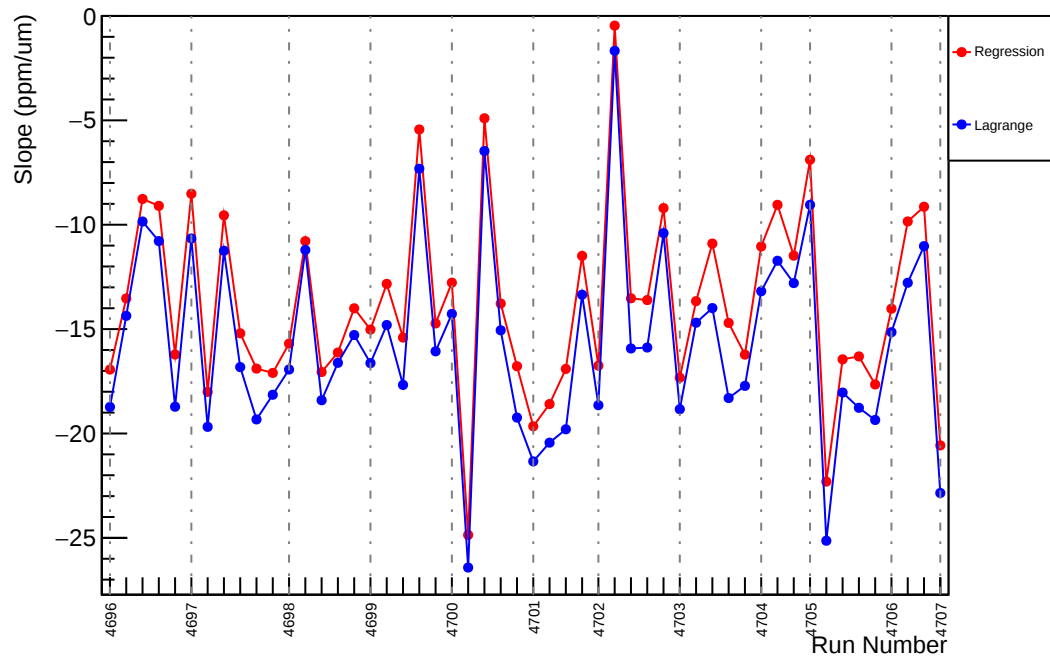
Slug75: Slope : usl_vs_evMon11 (ppm/um)
