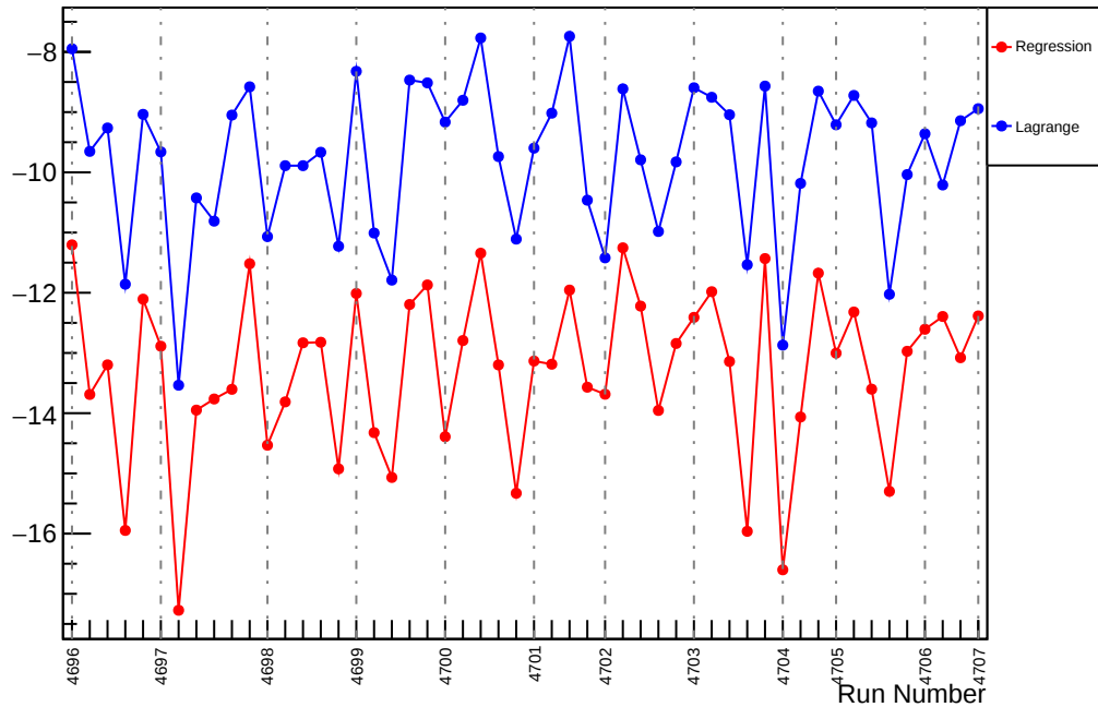
Slug75: Slope : usl_vs_evMon4 (ppm/um)
