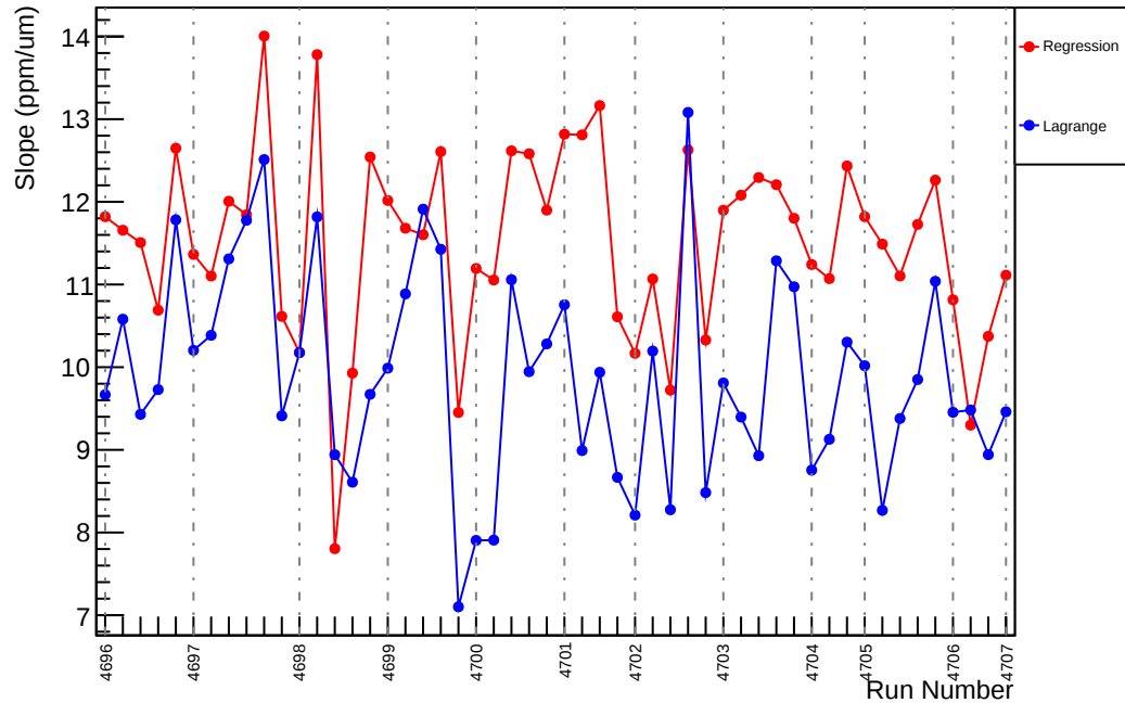
Slug75: Slope : usl_vs_evMon5 (ppm/um)
