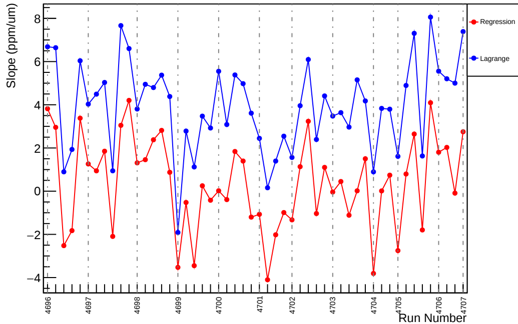
Slug75: Slope : usl_vs_evMon6 (ppm/um)
