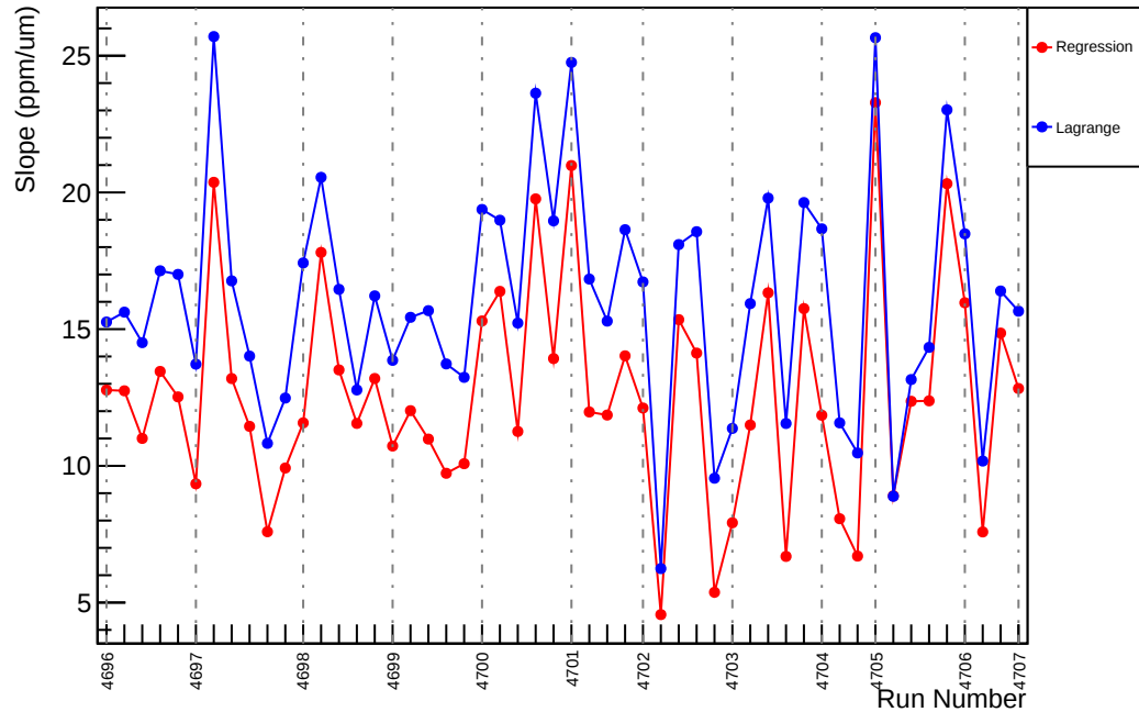
Slug75: Slope : usl_vs_evMon9 (ppm/um)
