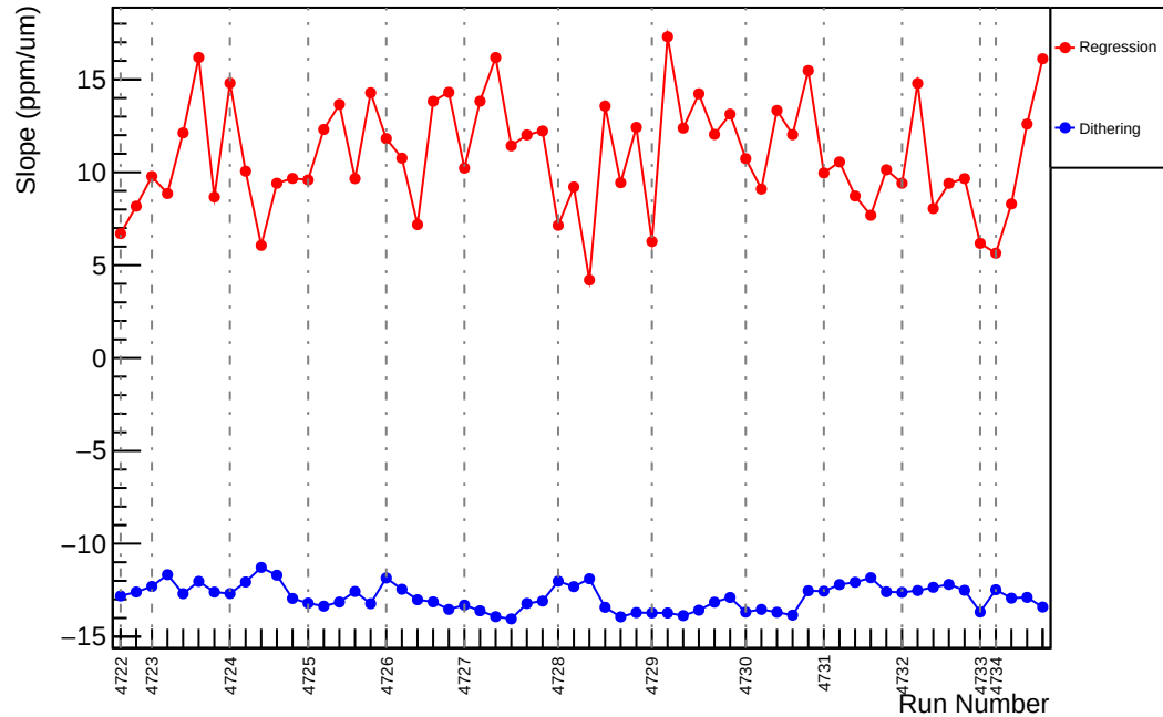
Slug76: Slope : usr_vs_evMon4 (ppm/um)
