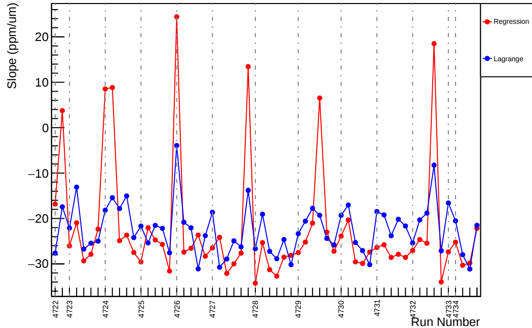
Slug76: Slope : usr_vs_evMon5 (ppm/um)
