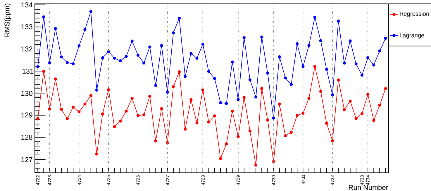
Slug76: Corrected RMS (ppm): asym_usr
