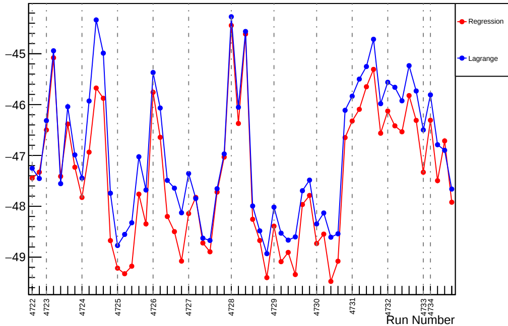
Slug76: Slope : usr_vs_evMon0 (ppm/um)
