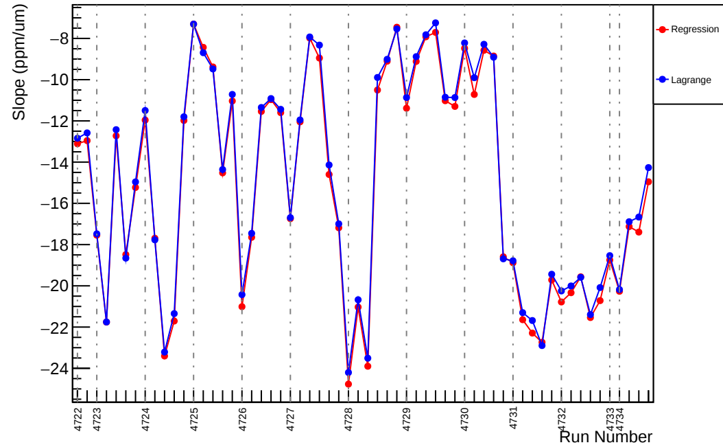
Slug76: Slope : usr_vs_evMon1 (ppm/um)
