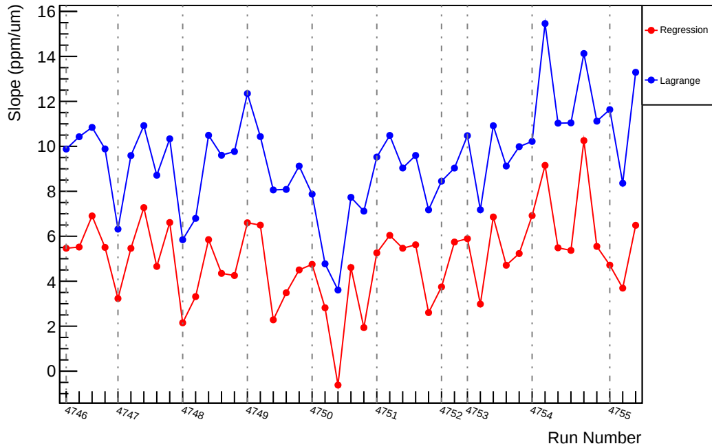
Slug78: Slope : us_avg_vs_evMon7 (ppm/um)
