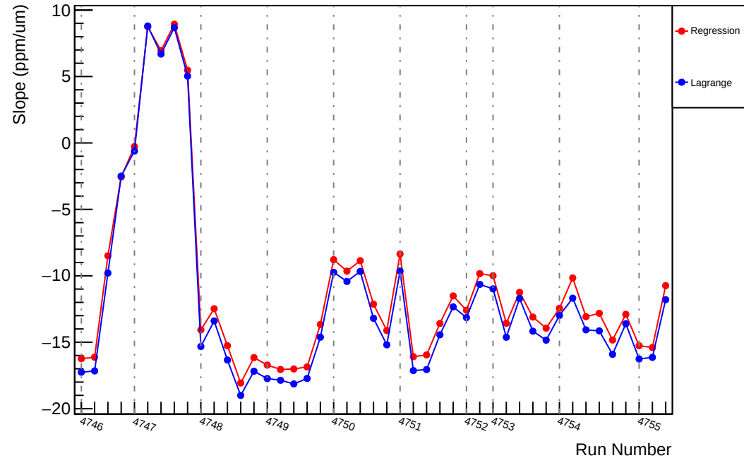
Slug78: Slope : us_avg_vs_evMon2 (ppm/um)
