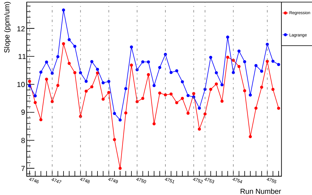
Slug78: Slope : us_avg_vs_evMon5 (ppm/um)
