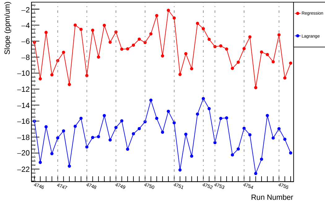
Slug78: Slope : us_avg_vs_evMon8 (ppm/um)
