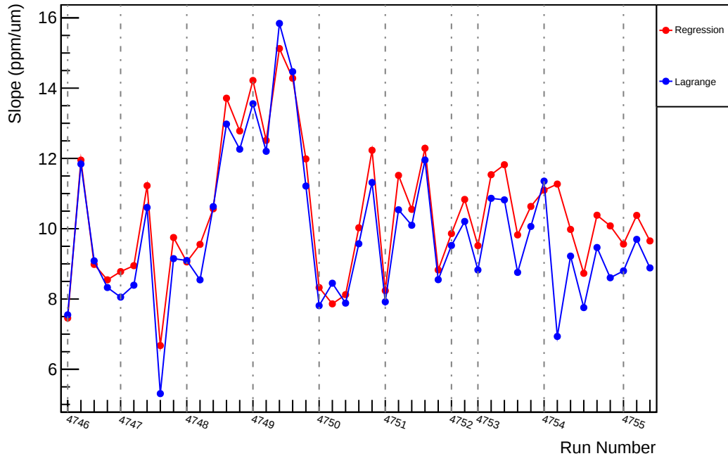
Slug78: Slope : us_avg_vs_evMon6 (ppm/um)
