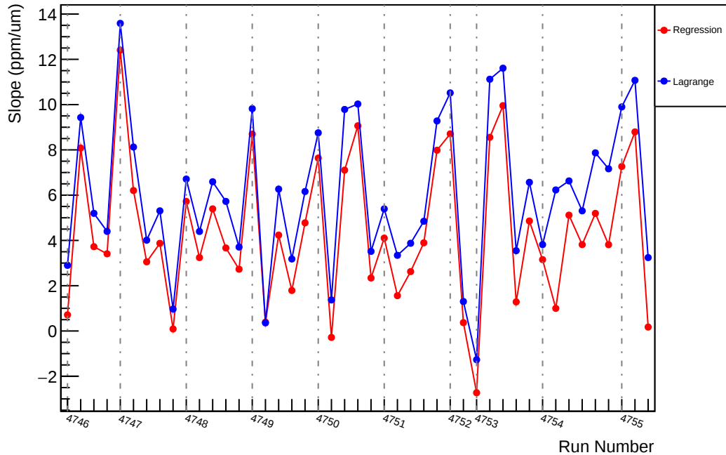
Slug78: Slope : us_avg_vs_evMon11 (ppm/um)
