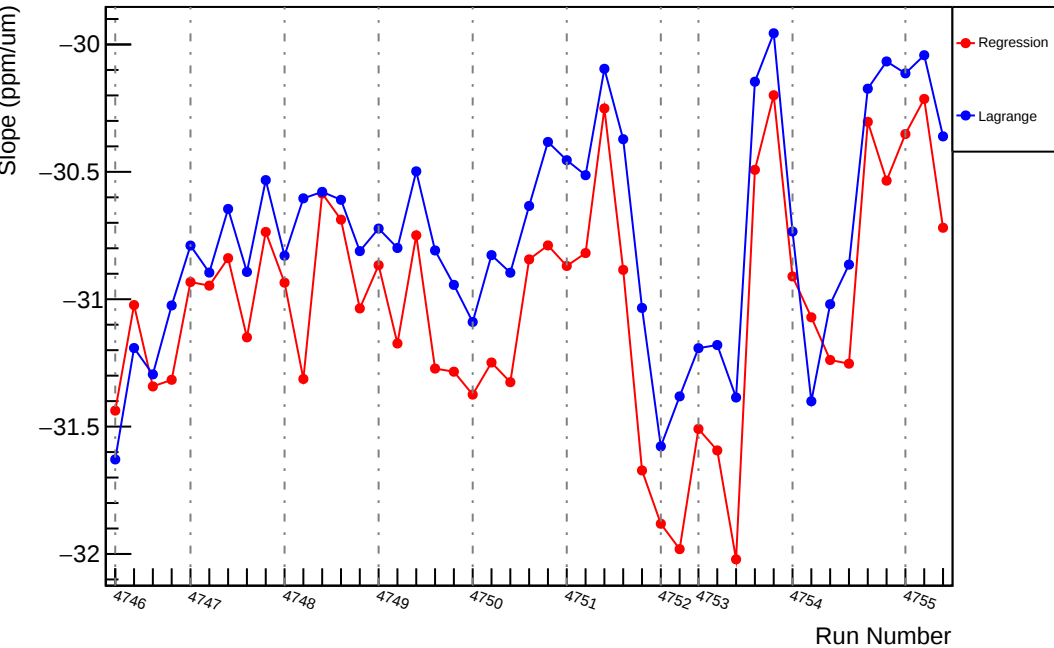
Slug78: Slope : us_avg_vs_evMon1 (ppm/um)
