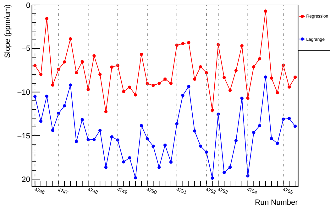
Slug78: Slope : us_avg_vs_evMon9 (ppm/um)
