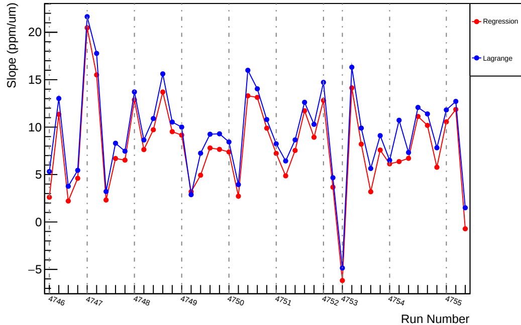
Slug78: Slope : usl_vs_evMon11 (ppm/um)
