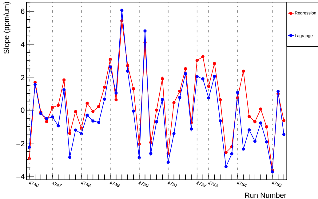
Slug78: Slope : usl_vs_evMon6 (ppm/um)
