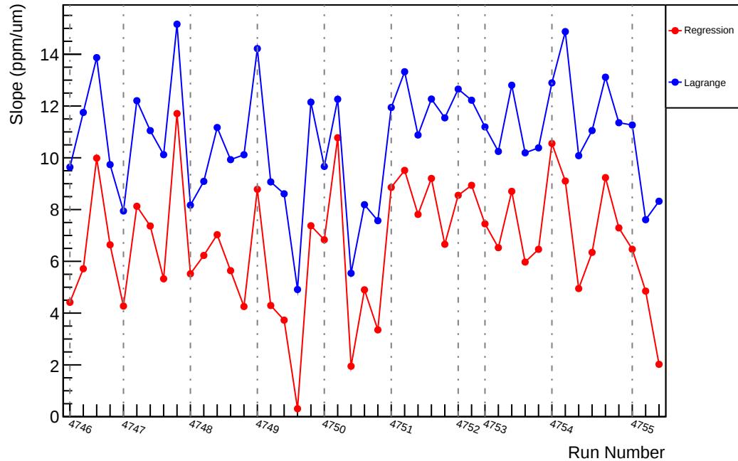
Slug78: Slope : usl_vs_evMon7 (ppm/um)
