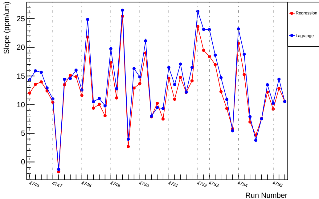
Slug78: Slope : usl_vs_evMon10 (ppm/um)
