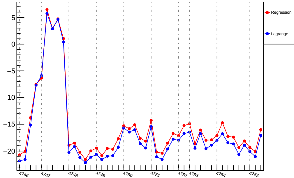
Slug78: Slope : usl_vs_evMon2 (ppm/um)
