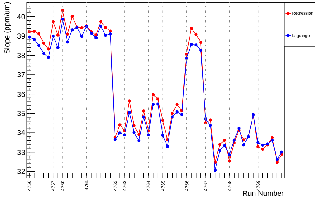
Slug79: Slope : usl_vs_evMon0 (ppm/um)
