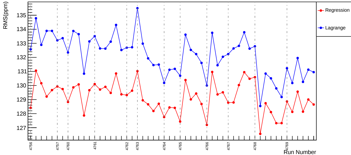
Slug79: Corrected RMS (ppm): asym_usr
