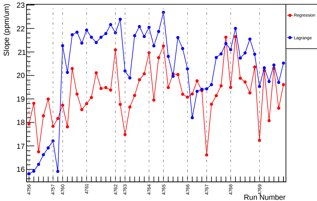
Slug79: Slope : usr_vs_evMon3 (ppm/um)
