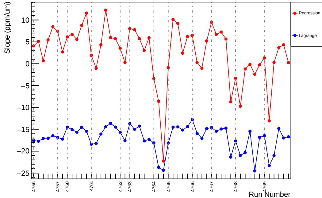
Slug79: Slope : usr_vs_evMon5 (ppm/um)
