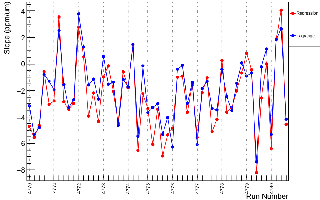
Slug80: Slope : us_dd_vs_evMon9 (ppm/um)
