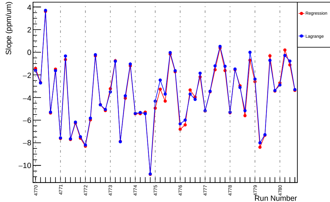
Slug80: Slope : us_dd_vs_evMon11 (ppm/um)
