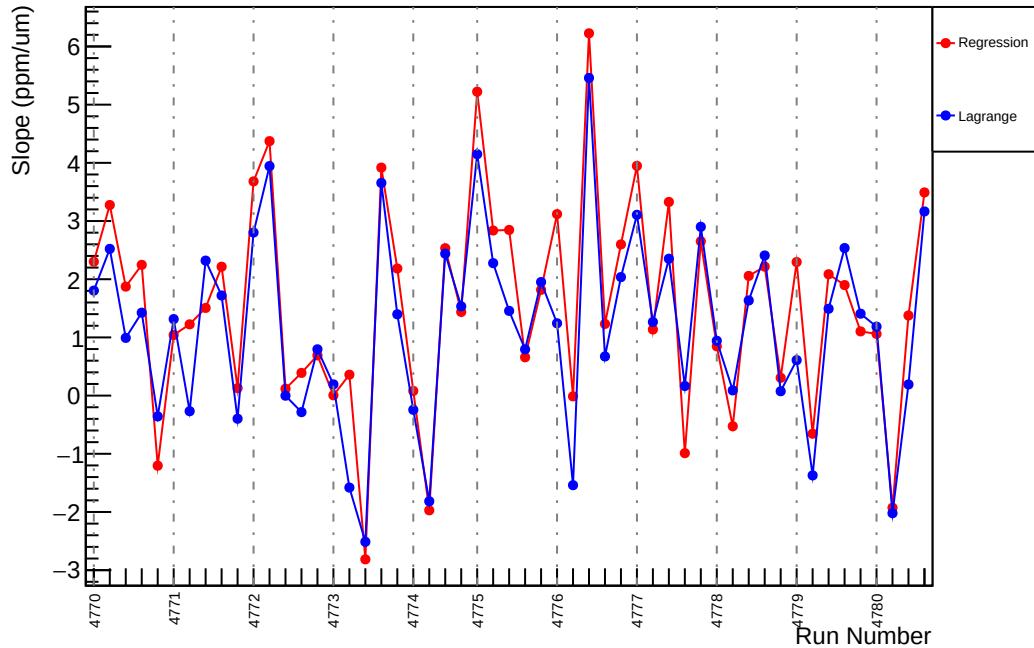
Slug80: Slope : us_dd_vs_evMon7 (ppm/um)
