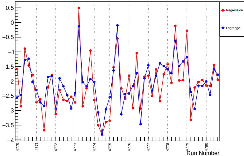
Slug80: Slope : us_dd_vs_evMon5 (ppm/um)
