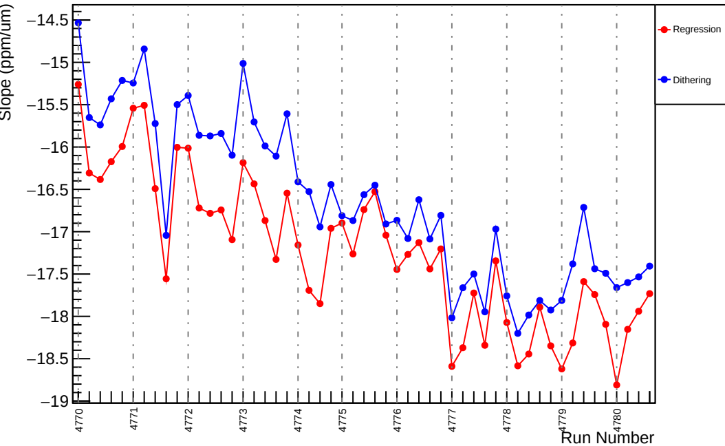
Slug80: Slope : usr_vs_evMon1 (ppm/um)
