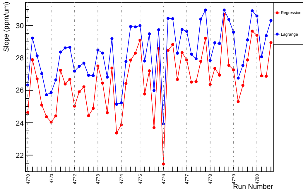
Slug80: Slope : usr_vs_evMon3 (ppm/um)
