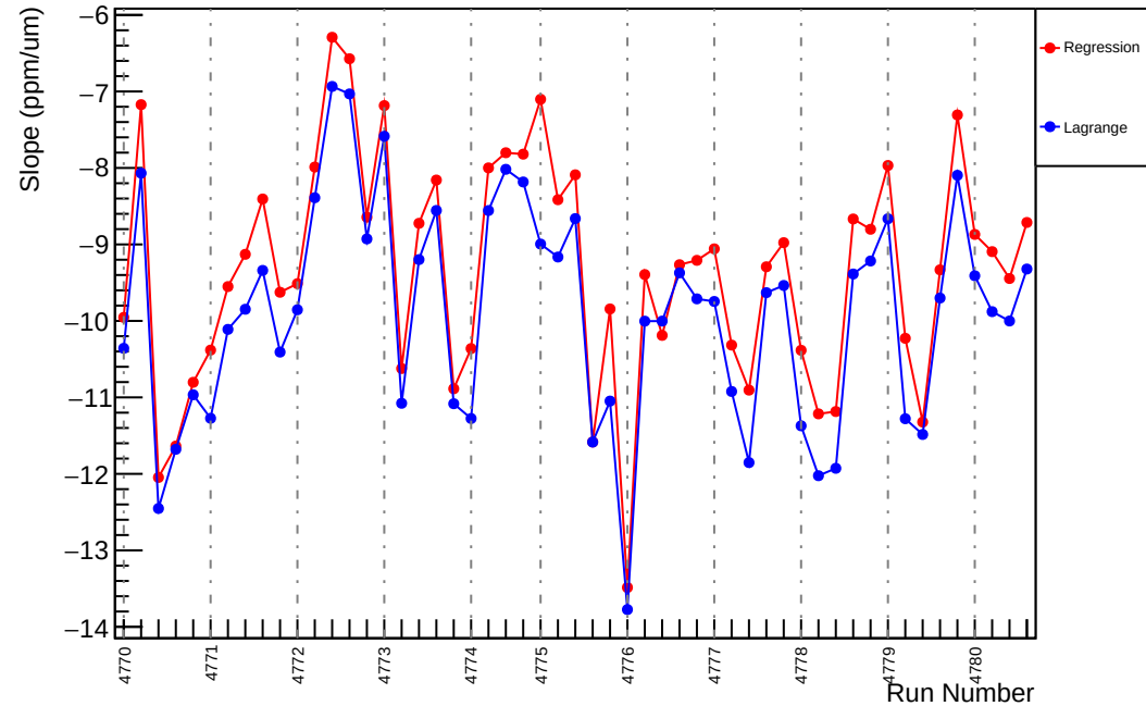
Slug80: Slope : usr_vs_evMon2 (ppm/um)
