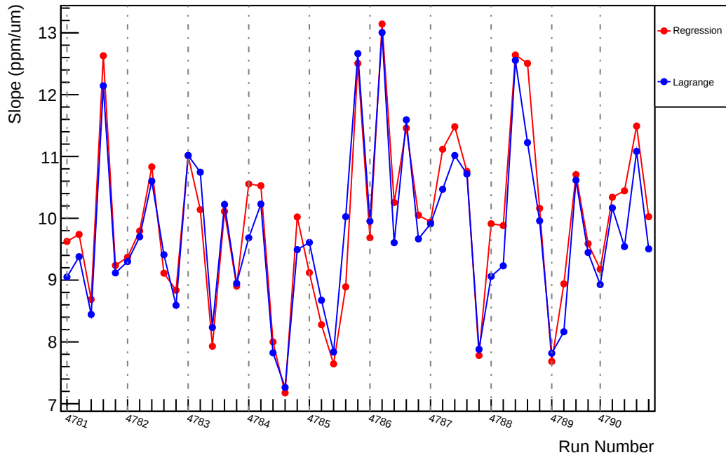
Slug81: Slope : us_dd_vs_evMon6 (ppm/um)
