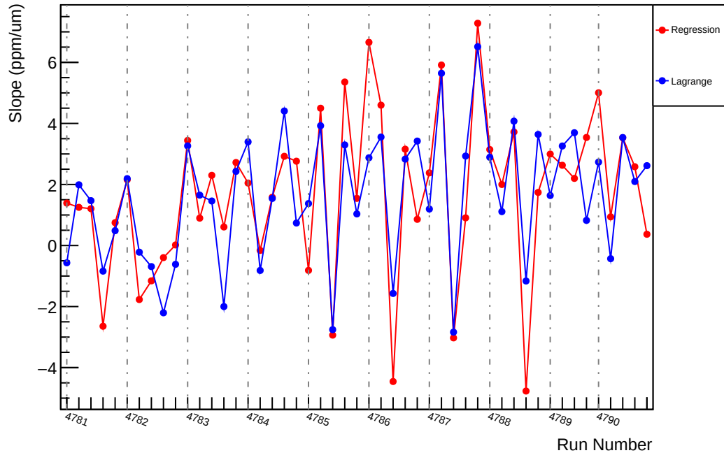
Slug81: Slope : us_dd_vs_evMon8 (ppm/um)
