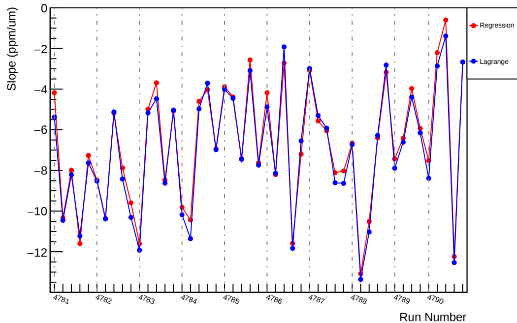
Slug81: Slope : us_dd_vs_evMon10 (ppm/um)
