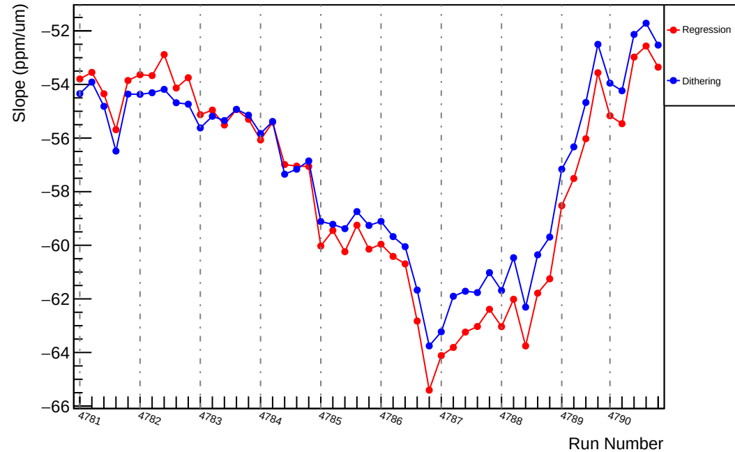
Slug81: Slope : usl_vs_evMon1 (ppm/um)
