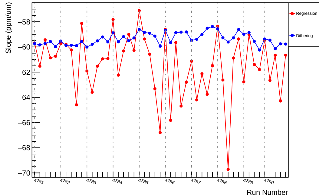
Slug81: Slope : usl_vs_evMon3 (ppm/um)
