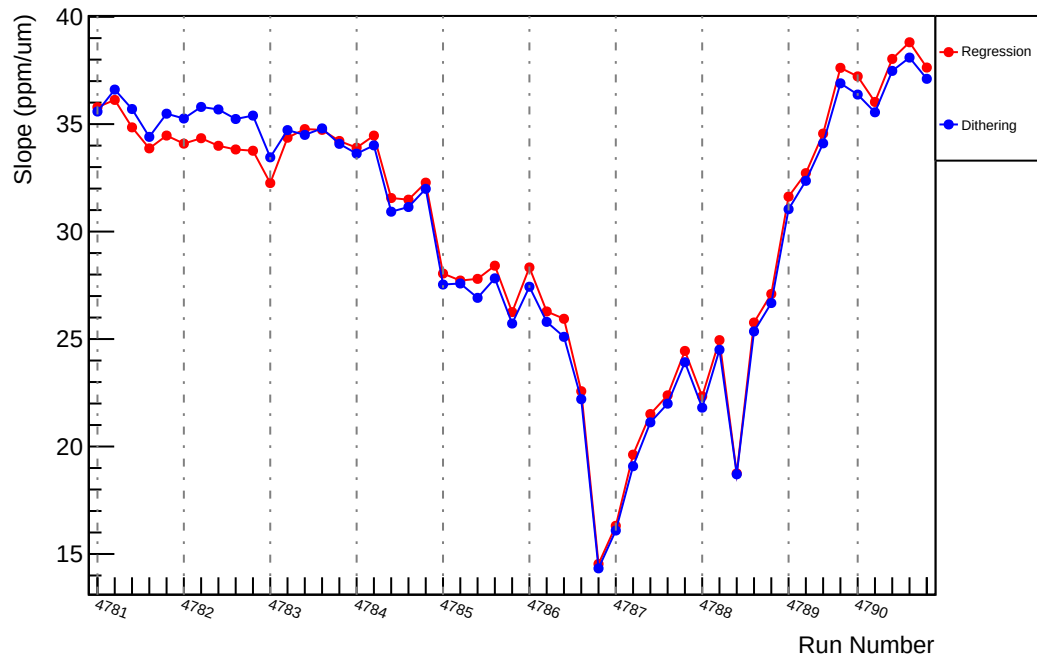
Slug81: Slope : usl_vs_evMon0 (ppm/um)
