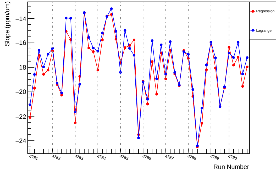
Slug81: Slope : usr_vs_evMon6 (ppm/um)
