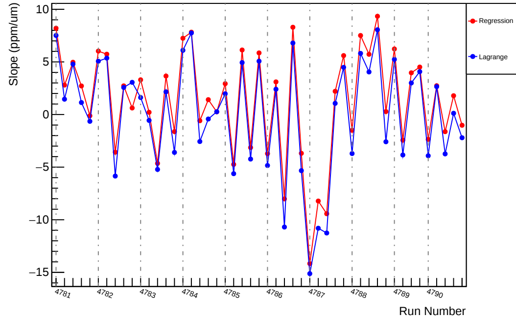
Slug81: Slope : usr_vs_evMon10 (ppm/um)
