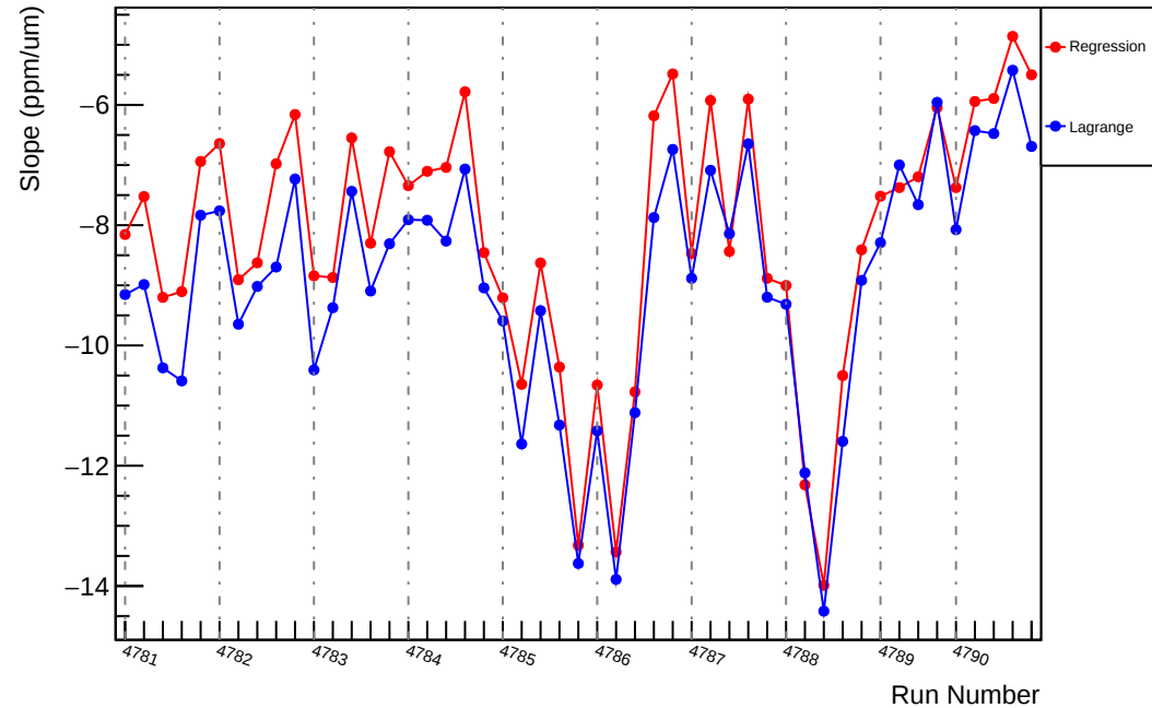
Slug81: Slope : usr_vs_evMon2 (ppm/um)
