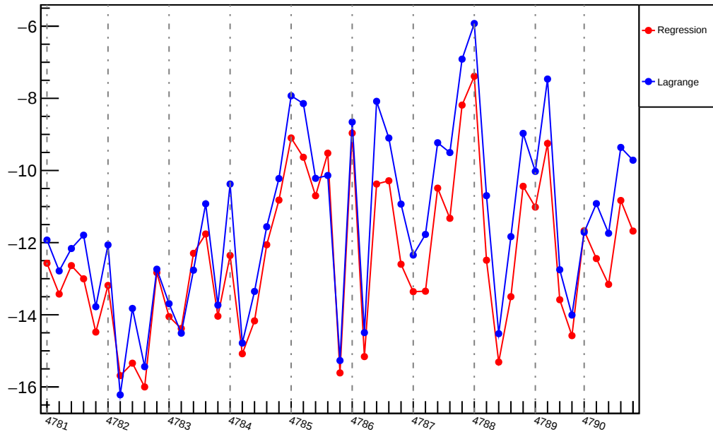
Slug81: Slope : usr_vs_evMon4 (ppm/um)
