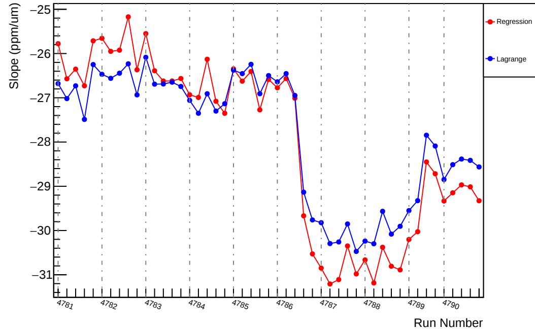
Slug81: Slope : usr_vs_evMon1 (ppm/um)
