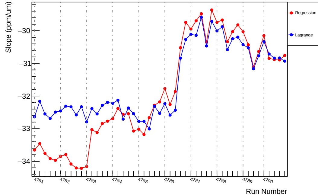
Slug81: Slope : usr_vs_evMon0 (ppm/um)
