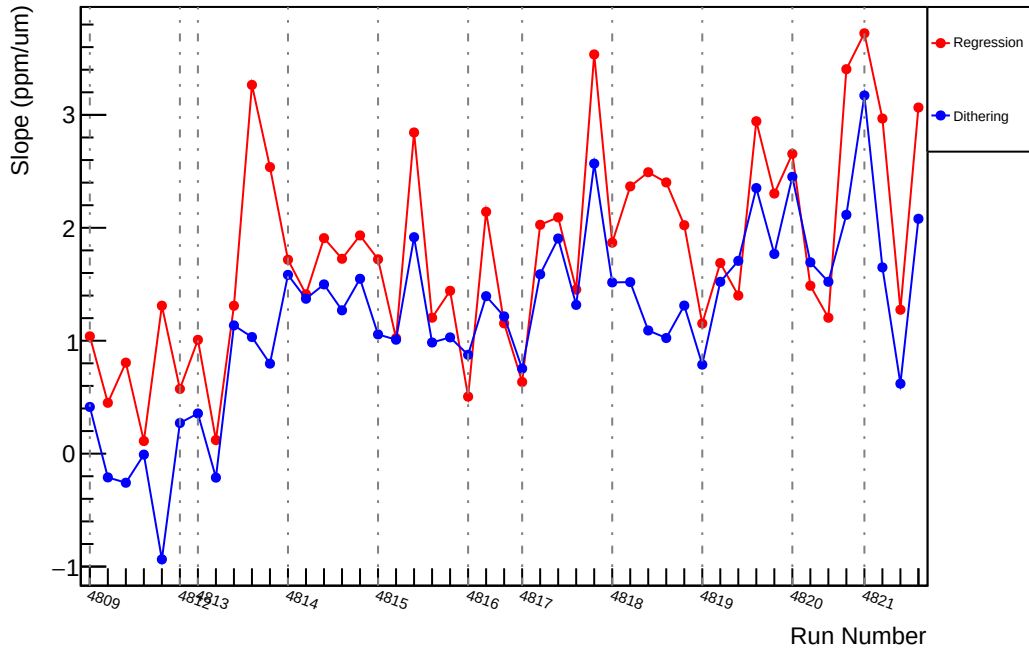
Slug83: Slope : us_dd_vs_evMon2 (ppm/um)
