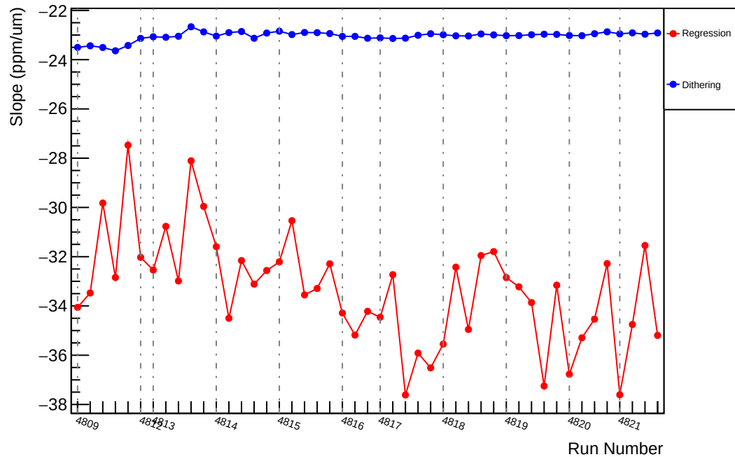
Slug83: Slope : us_dd_vs_evMon3 (ppm/um)
