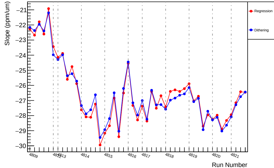
Slug83: Slope : us_dd_vs_evMon1 (ppm/um)
