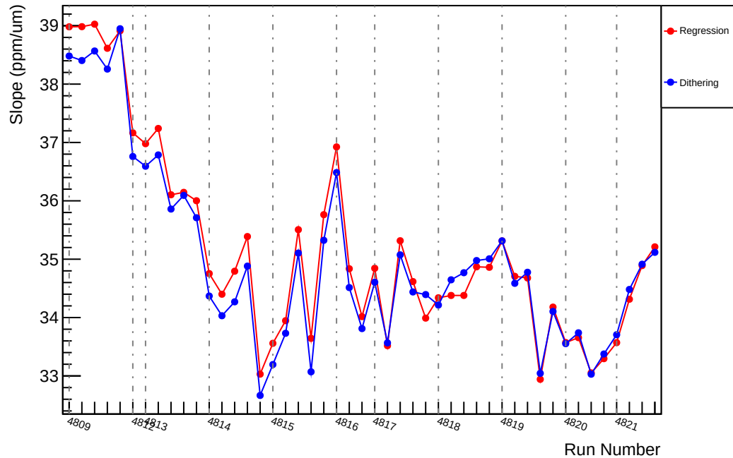
Slug83: Slope : us_dd_vs_evMon0 (ppm/um)
