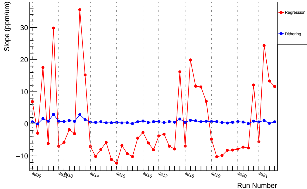
Slug83: Slope : us_dd_vs_evMon4 (ppm/um)
