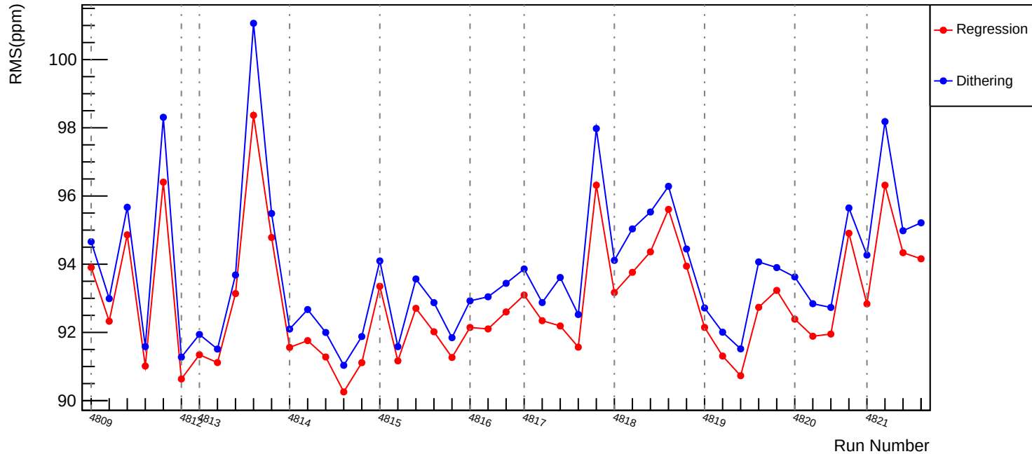
Slug83: Corrected RMS (ppm): asym_us_dd
