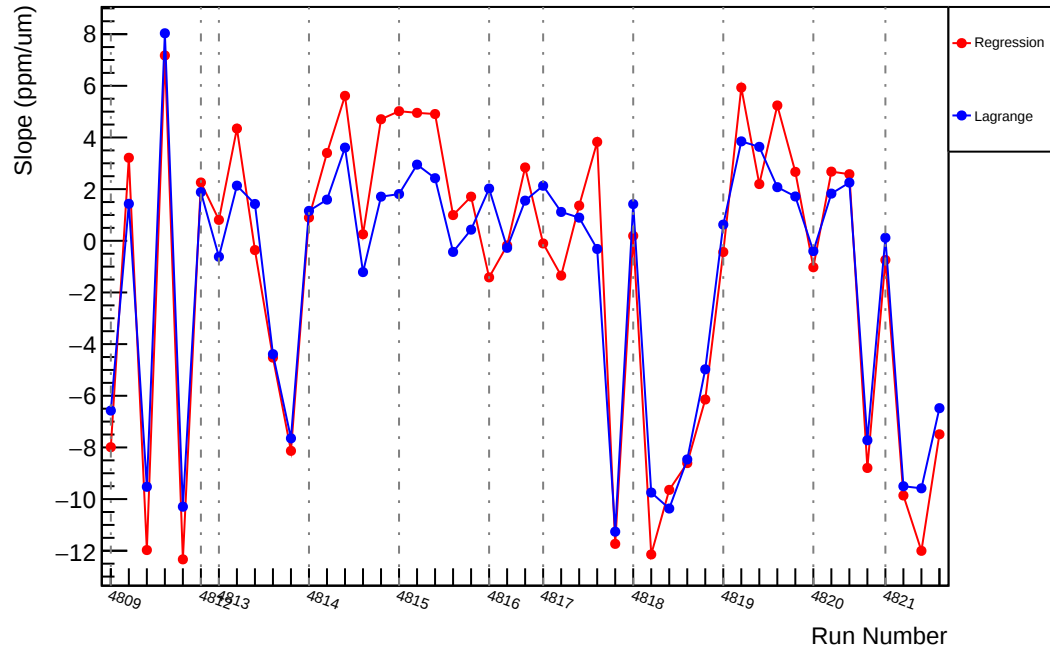
Slug83: Slope : us_dd_vs_evMon8 (ppm/um)
