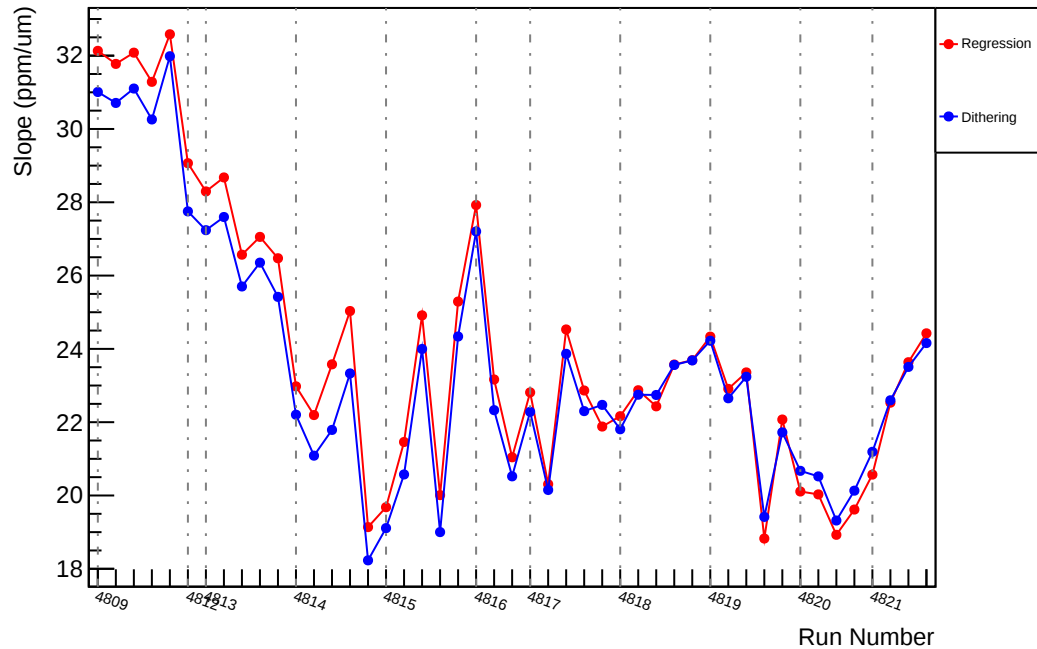
Slug83: Slope : usl_vs_evMon0 (ppm/um)
