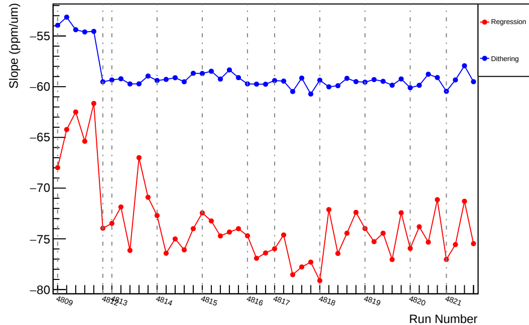
Slug83: Slope : usl_vs_evMon3 (ppm/um)
