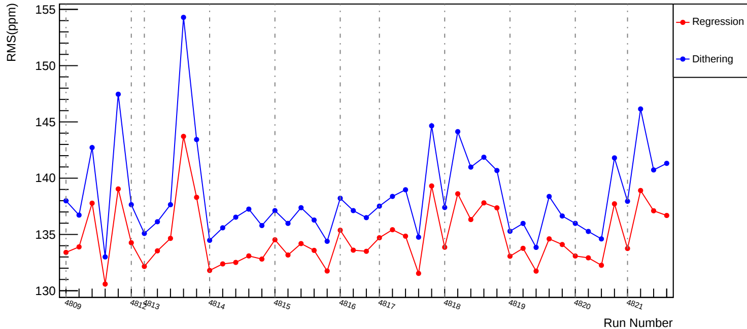
Slug83: Corrected RMS (ppm): asym_usl
