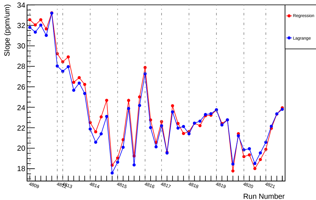
Slug83: Slope : usl_vs_evMon0 (ppm/um)
