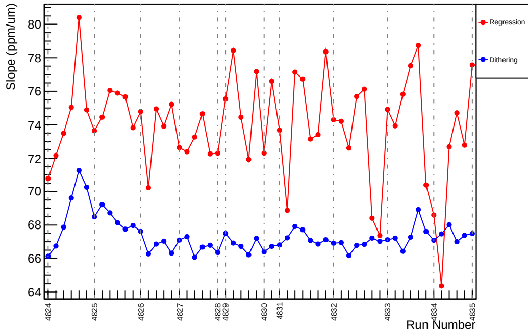
Slug84: Slope : usl_vs_evMon3 (ppm/um)
