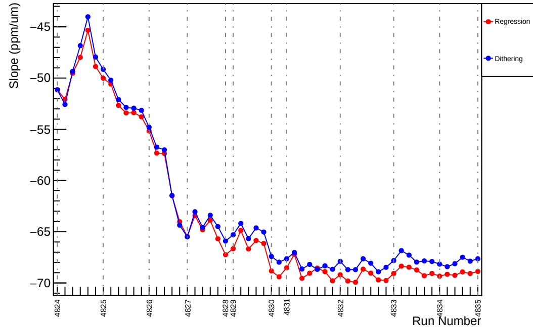
Slug84: Slope : usl_vs_evMon1 (ppm/um)
