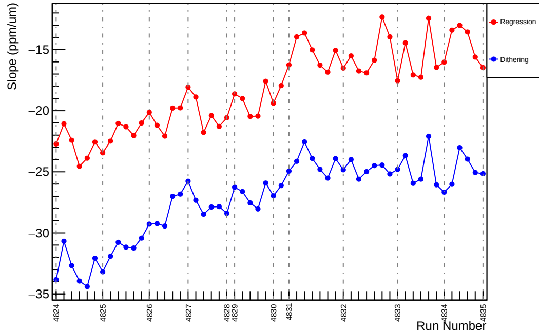
Slug84: Slope : usl_vs_evMon2 (ppm/um)
