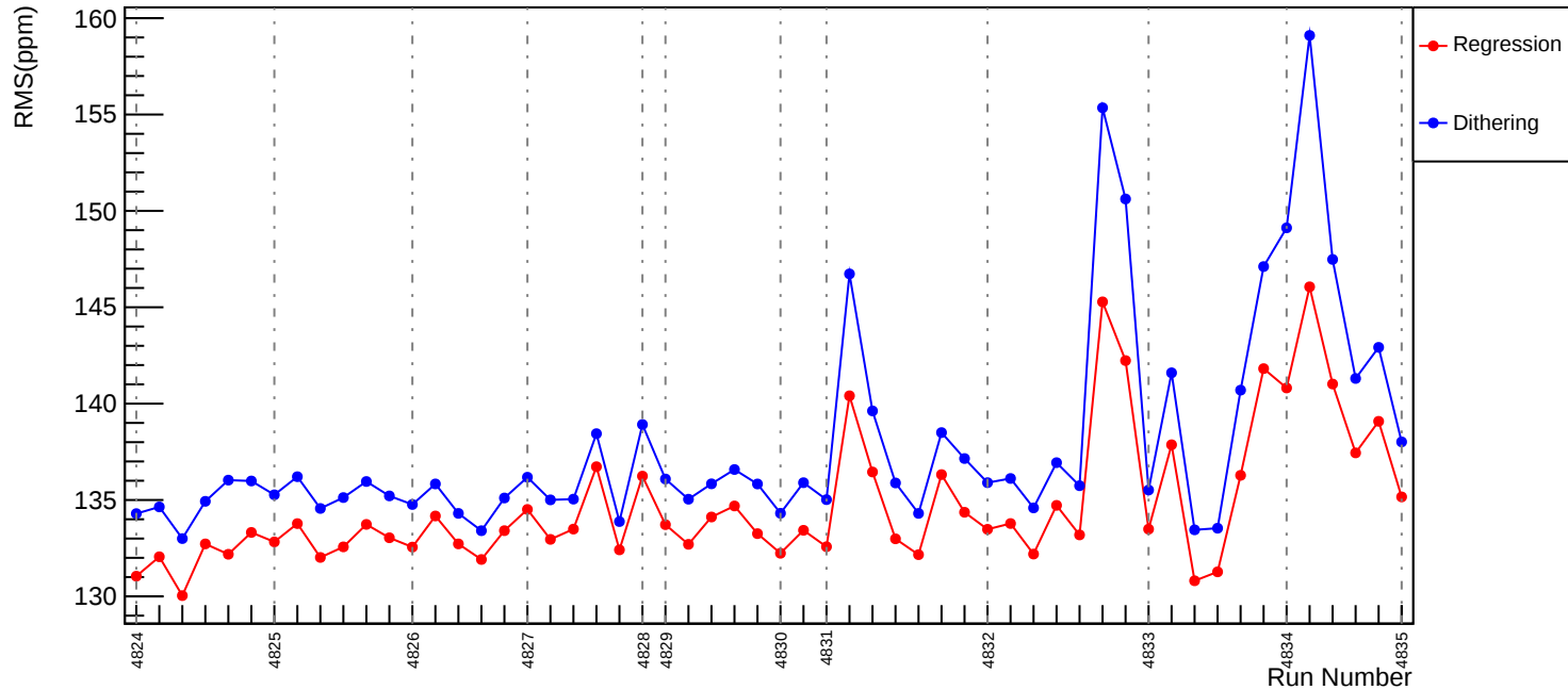
Slug84: Corrected RMS (ppm): asym_usl
