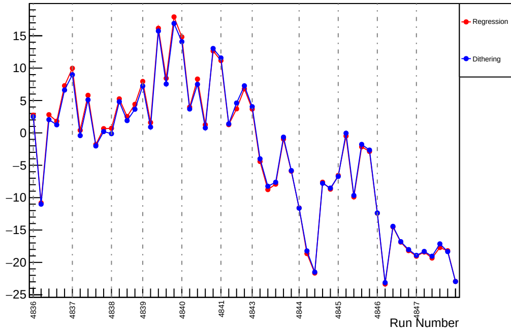
Slug85: Slope : usl_vs_evMon0 (ppm/um)
