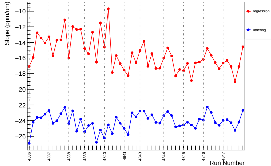
Slug85: Slope : usl_vs_evMon2 (ppm/um)
