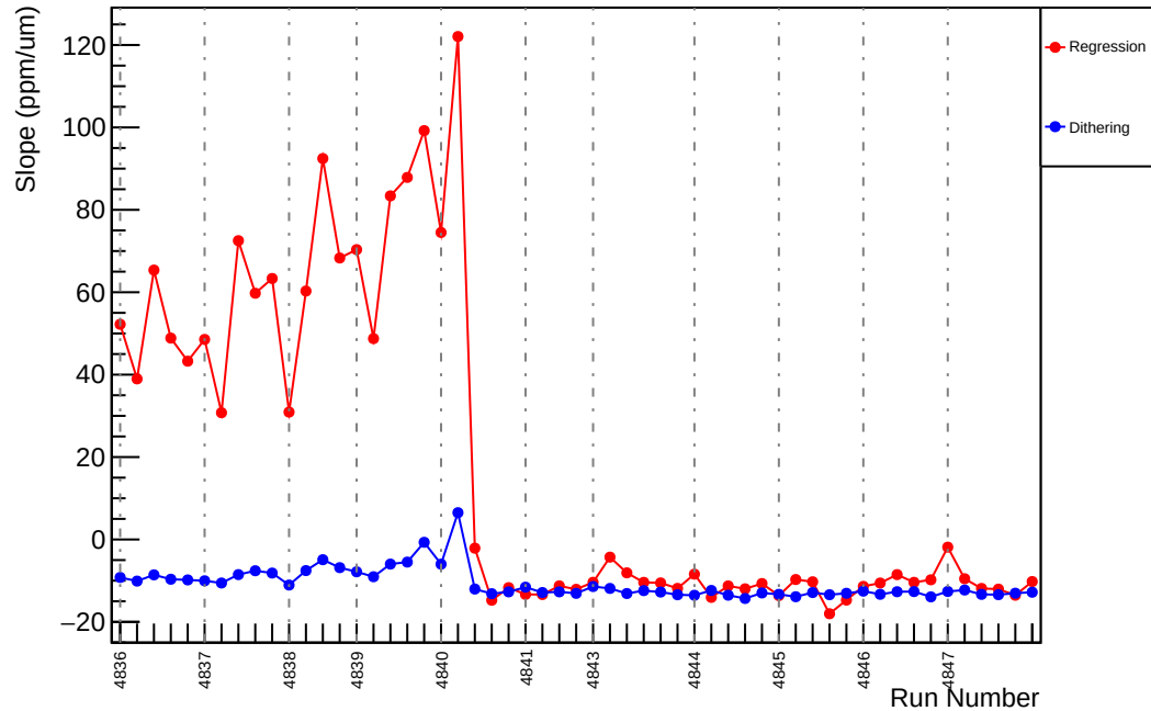
Slug85: Slope : usl_vs_evMon4 (ppm/um)
